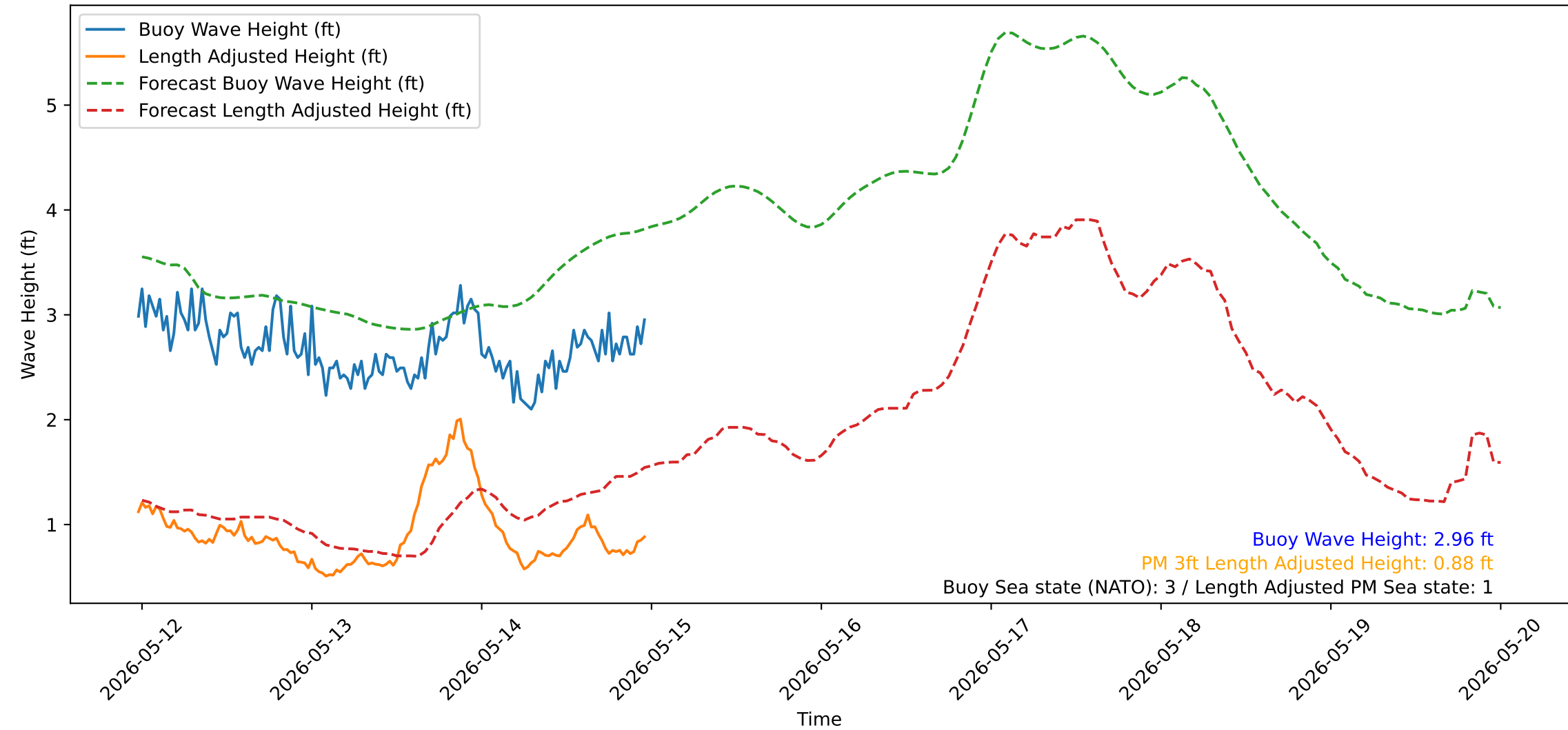
Wave Heights over Time for Green Beach at 2026-05-14 23:41:15
