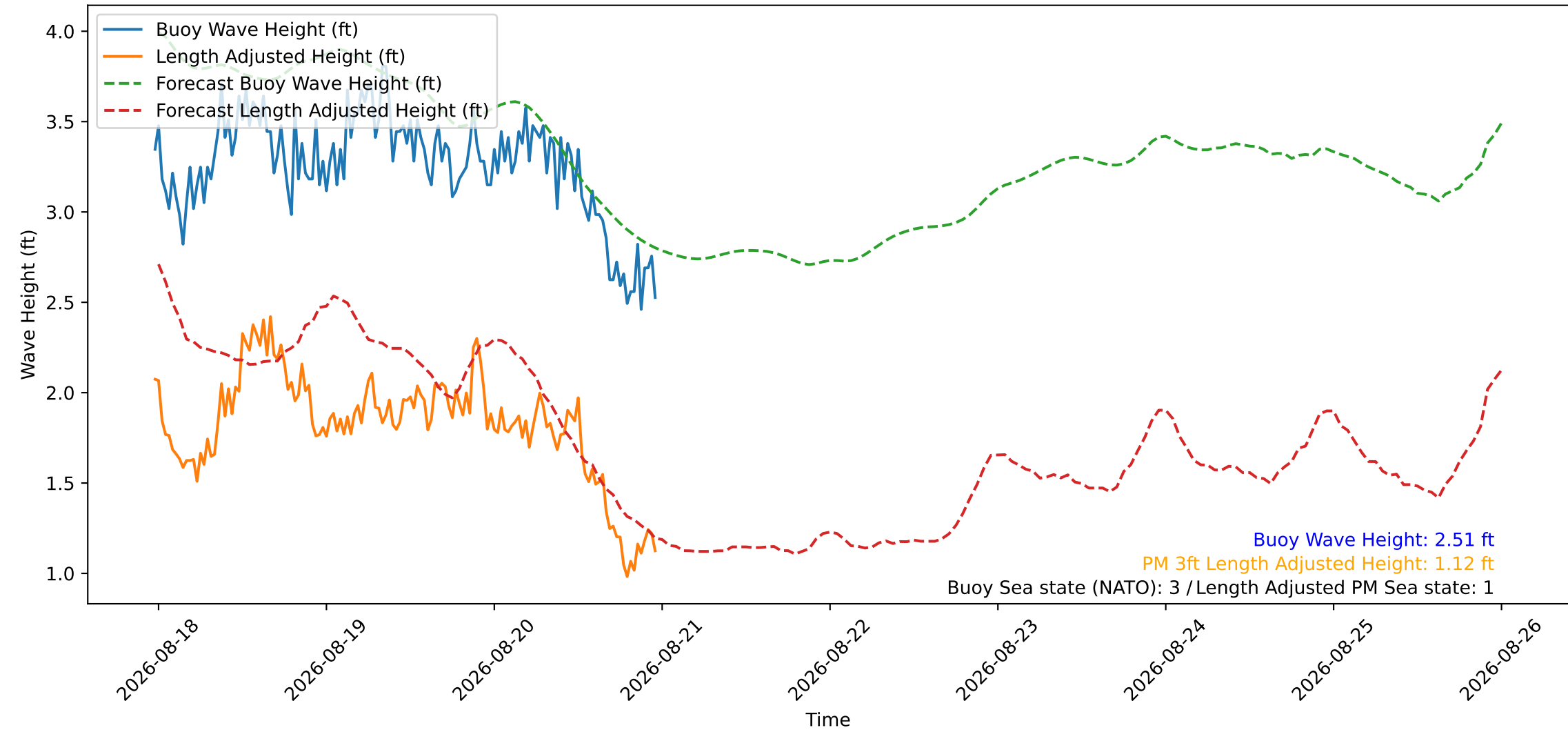
Wave Heights over Time for Oceanside Harbor at 2026-08-20 23:40:26
