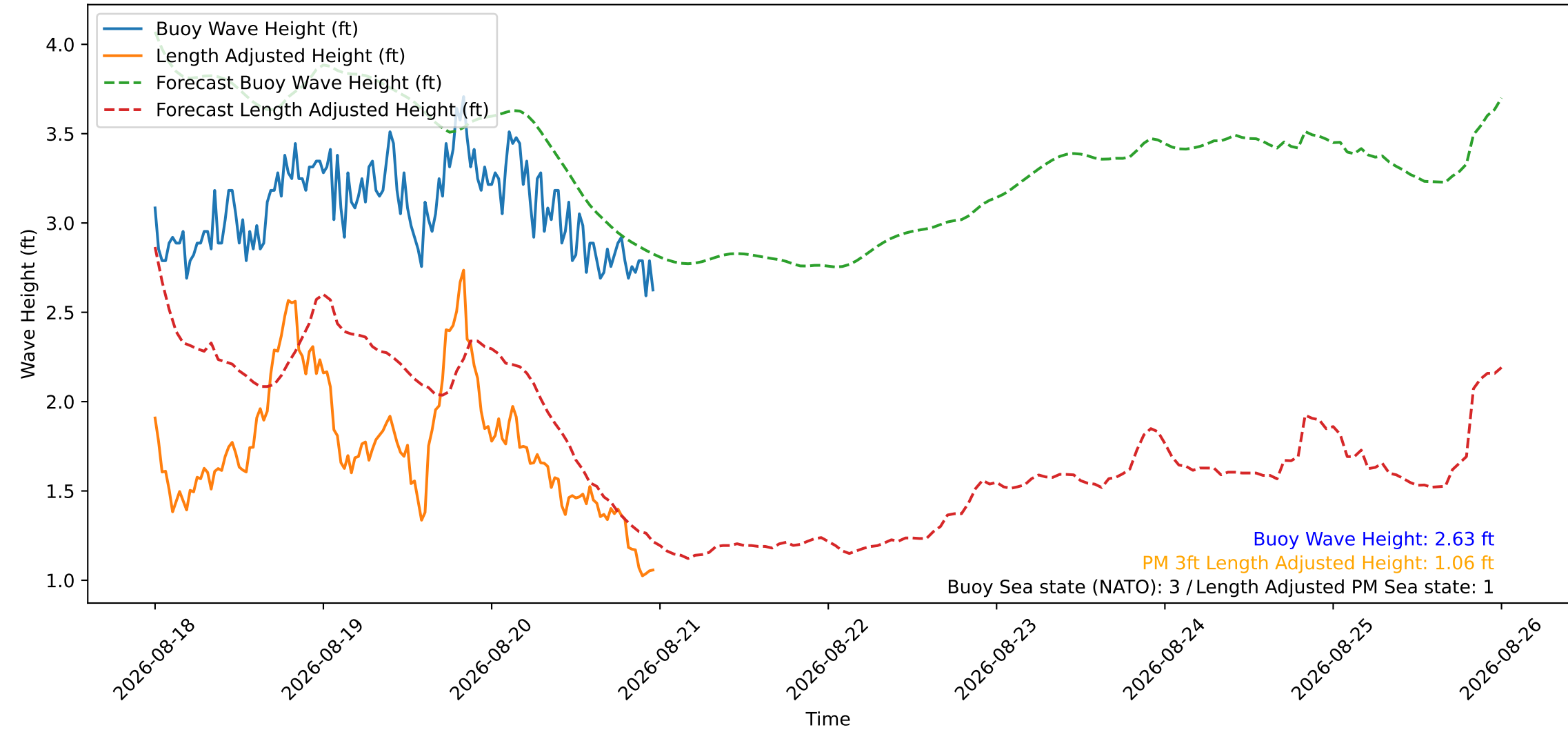
Wave Heights over Time for Green Beach at 2026-08-20 23:41:09
