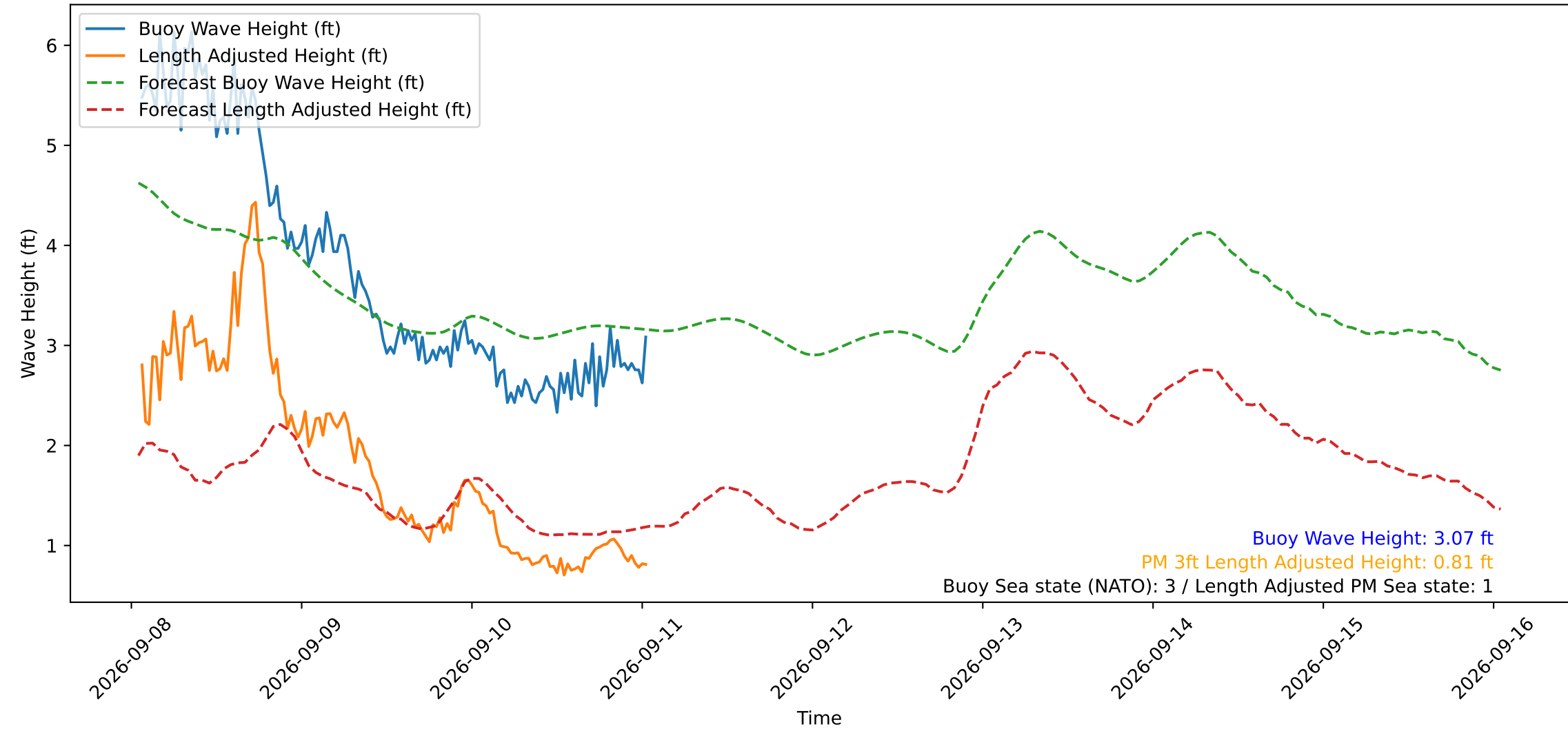
Wave Heights over Time for Red Beach at 2026-09-11 01:20:51
