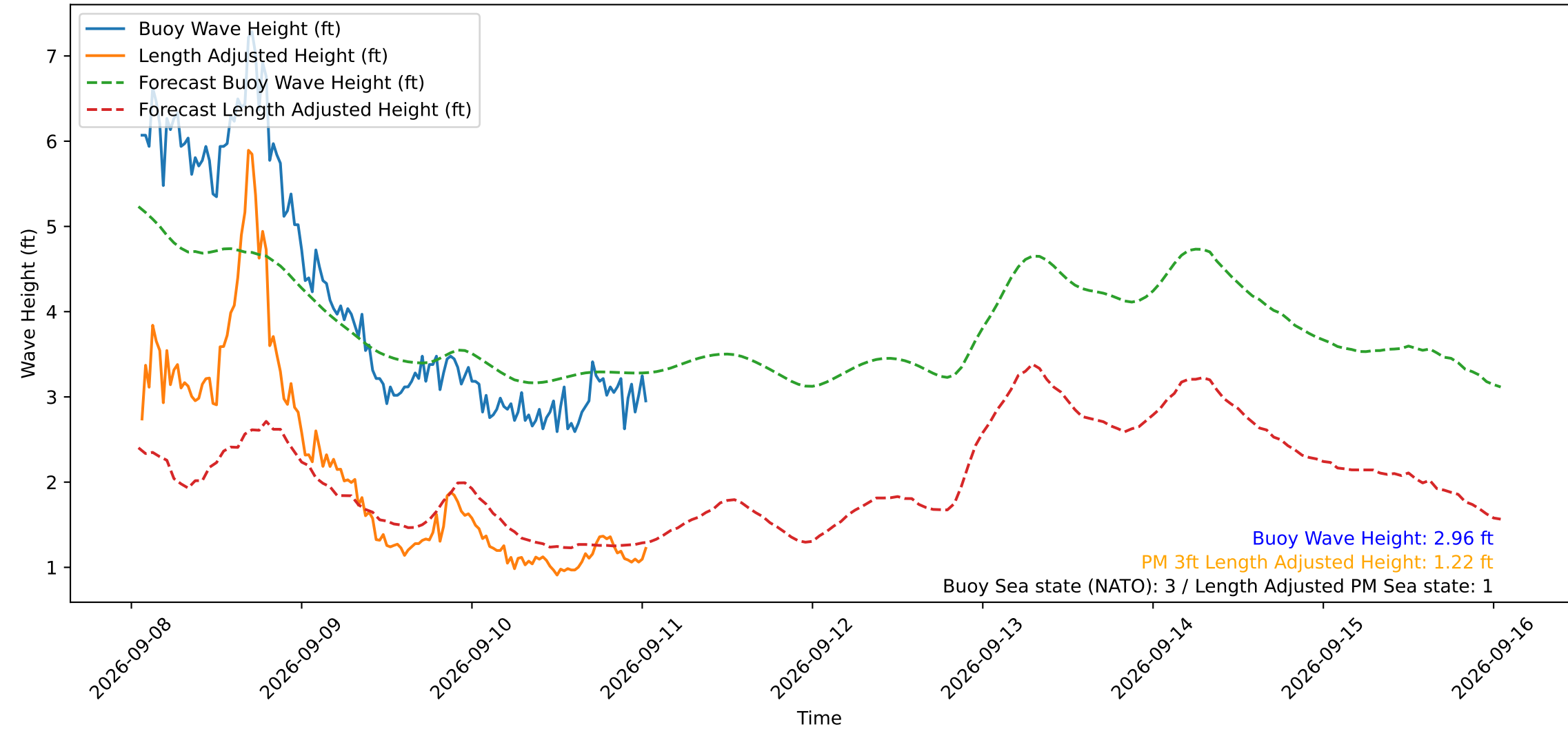
Wave Heights over Time for Green Beach at 2026-09-11 01:21:14
