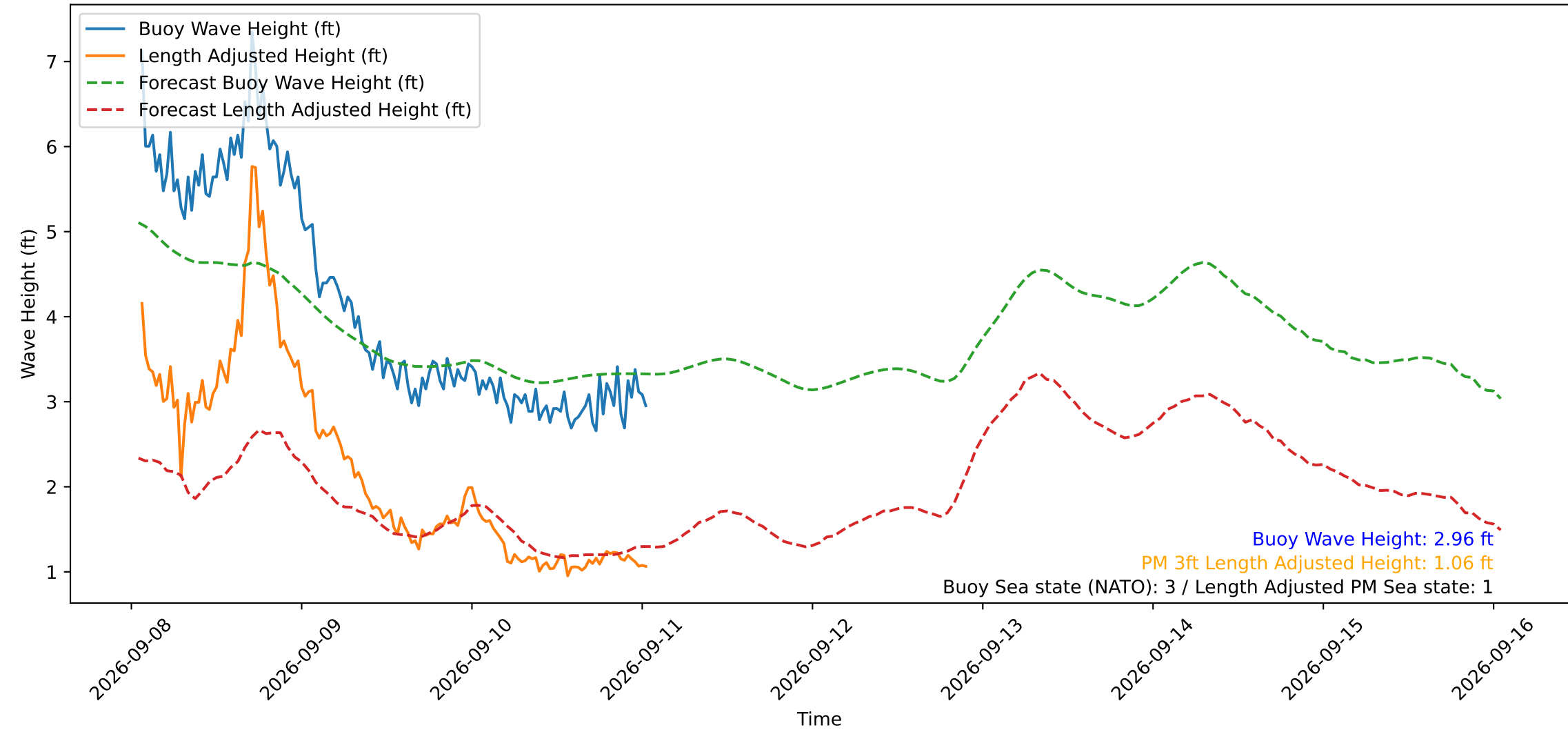
Wave Heights over Time for Oceanside Harbor at 2026-09-11 01:20:29
