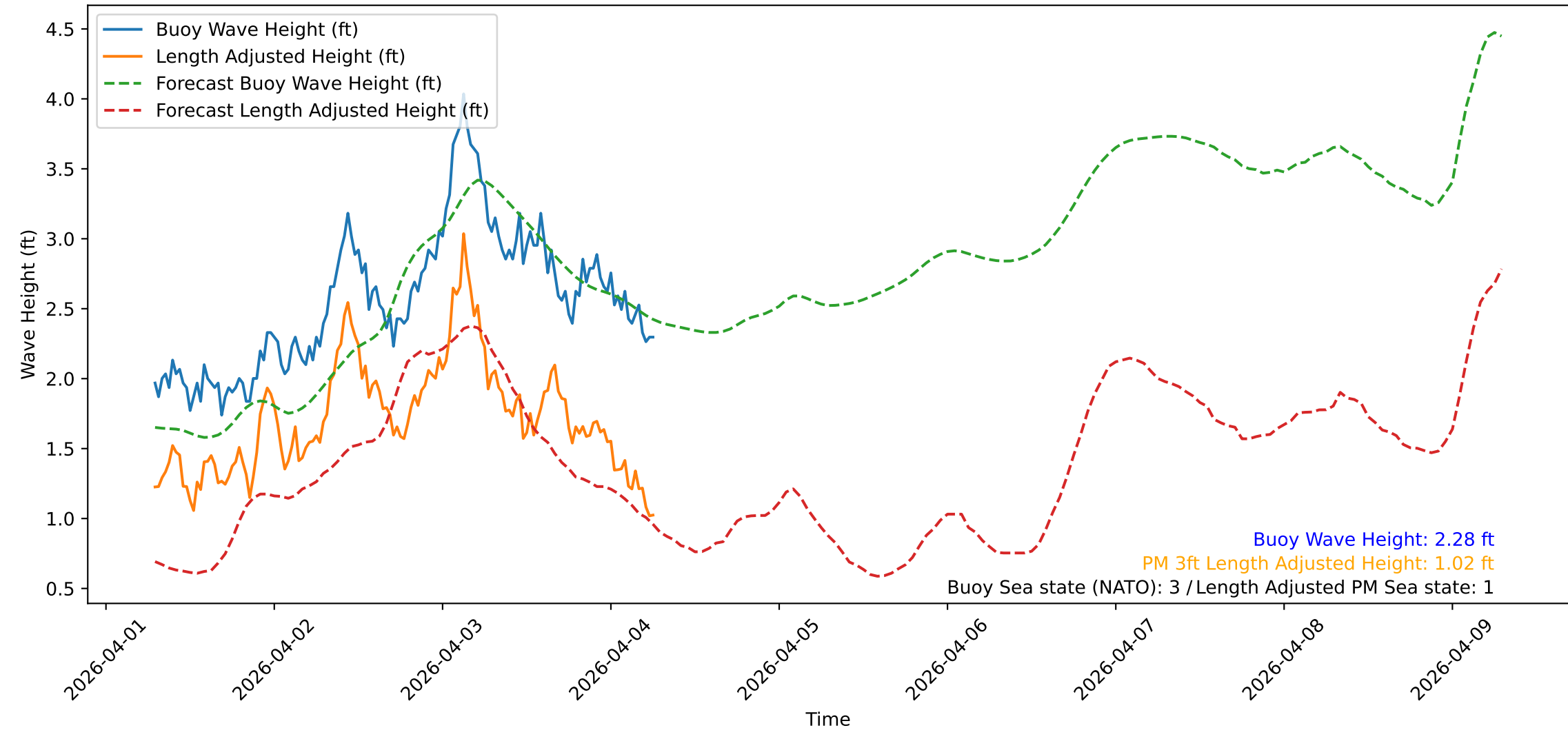
Wave Heights over Time for Oceanside Harbor at 2026-04-04 07:10:31
