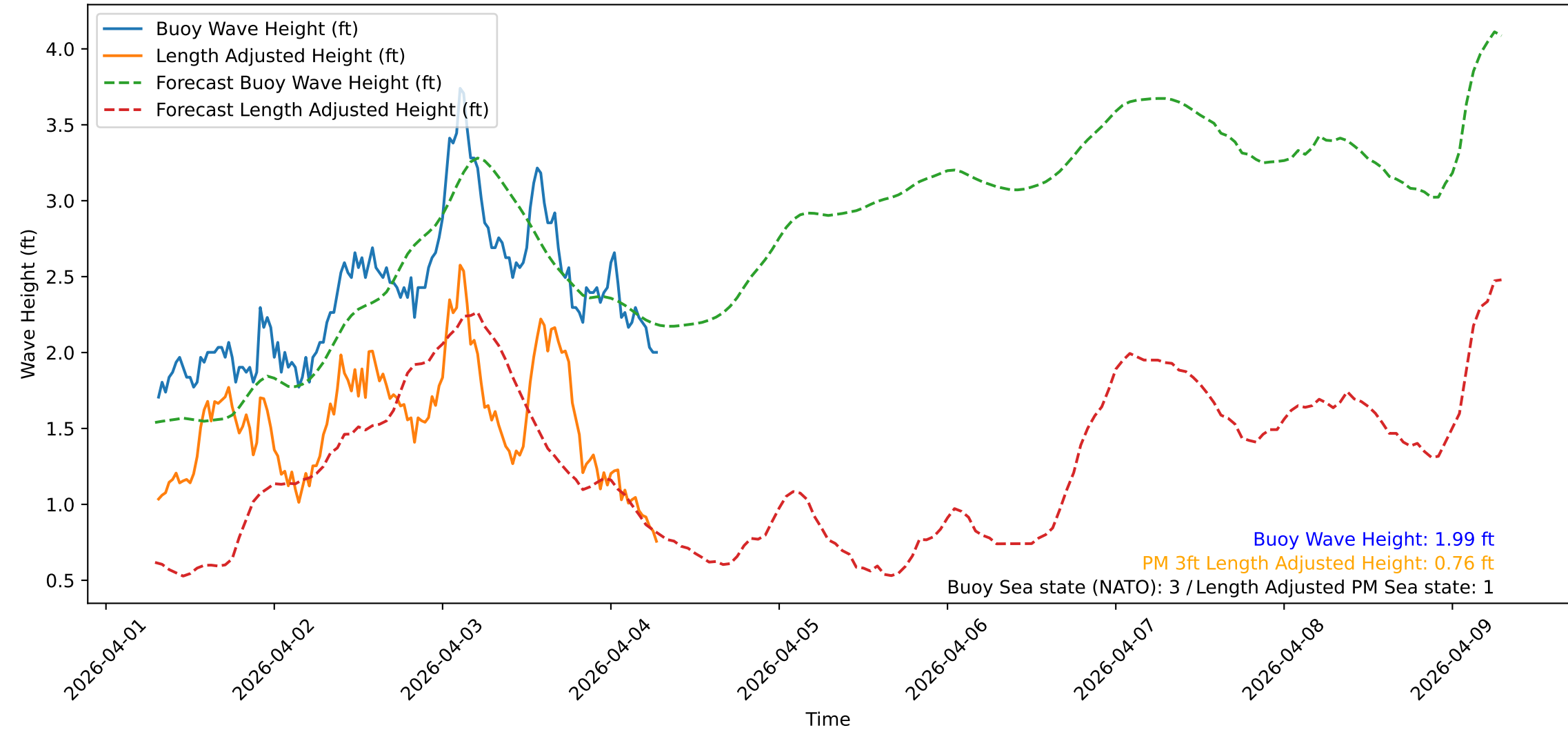
Wave Heights over Time for Red Beach at 2026-04-04 07:10:47
