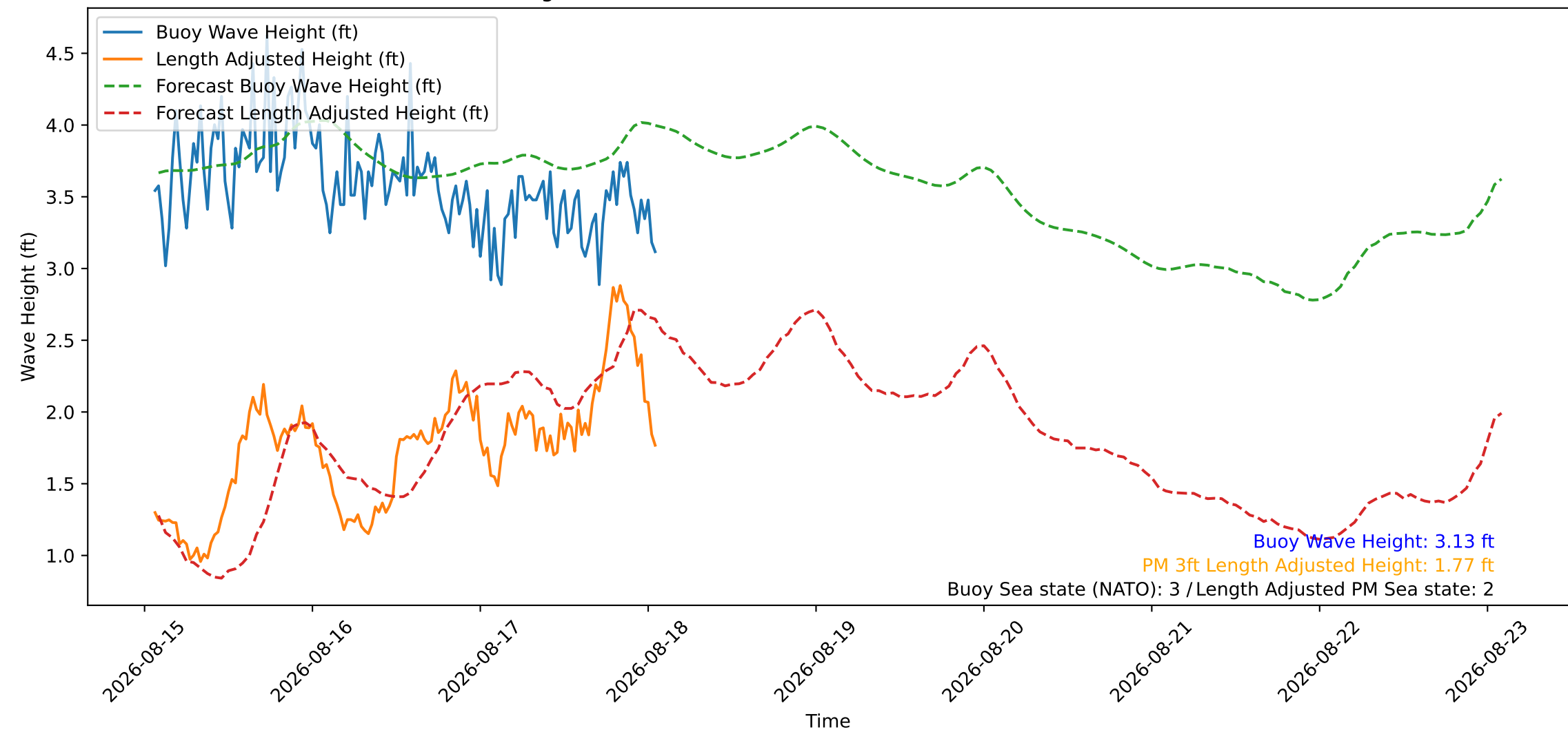
Wave Heights over Time for Oceanside Harbor at 2026-08-18 01:40:27
