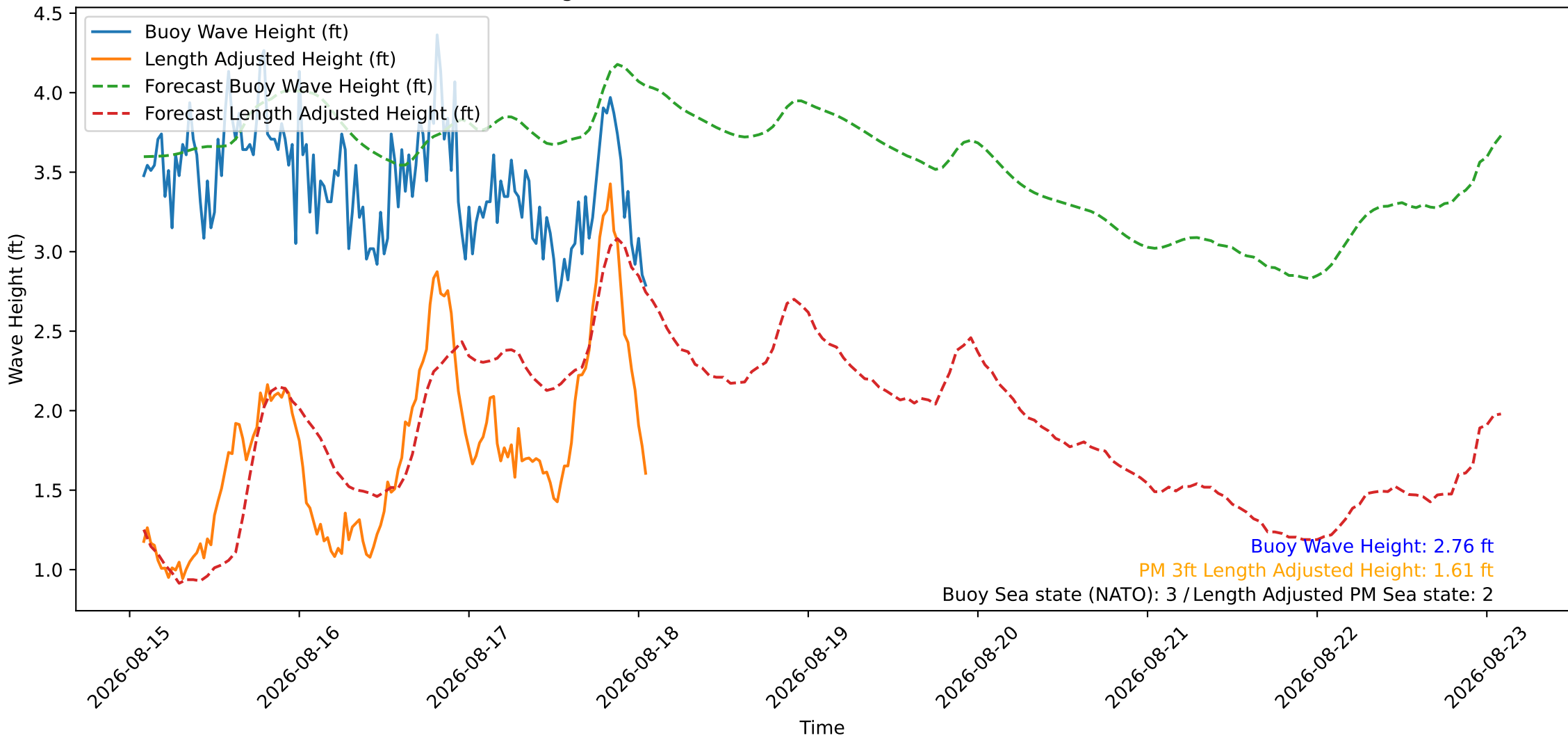
Wave Heights over Time for Green Beach at 2026-08-18 01:41:09
