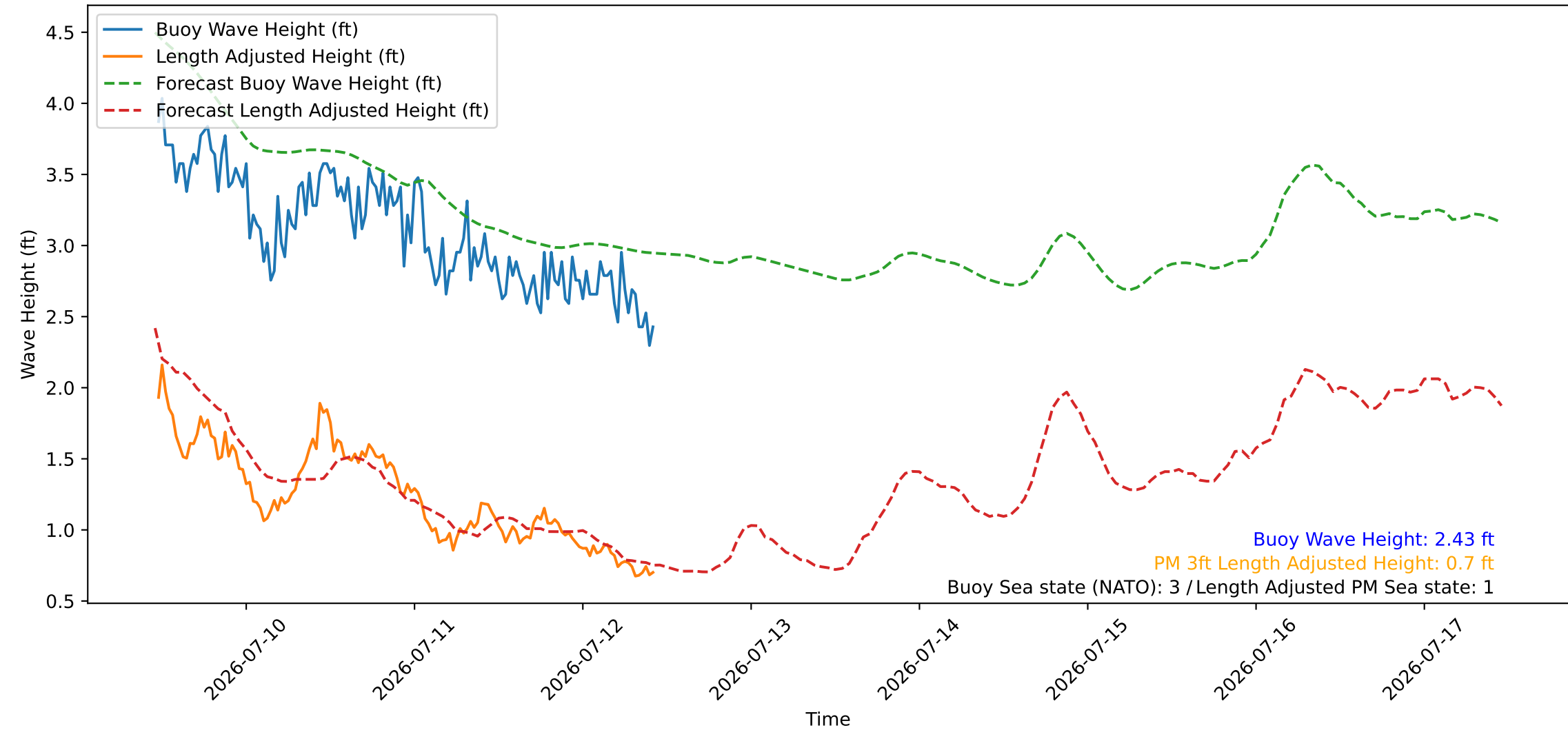
Wave Heights over Time for Green Beach at 2026-07-12 11:21:09
