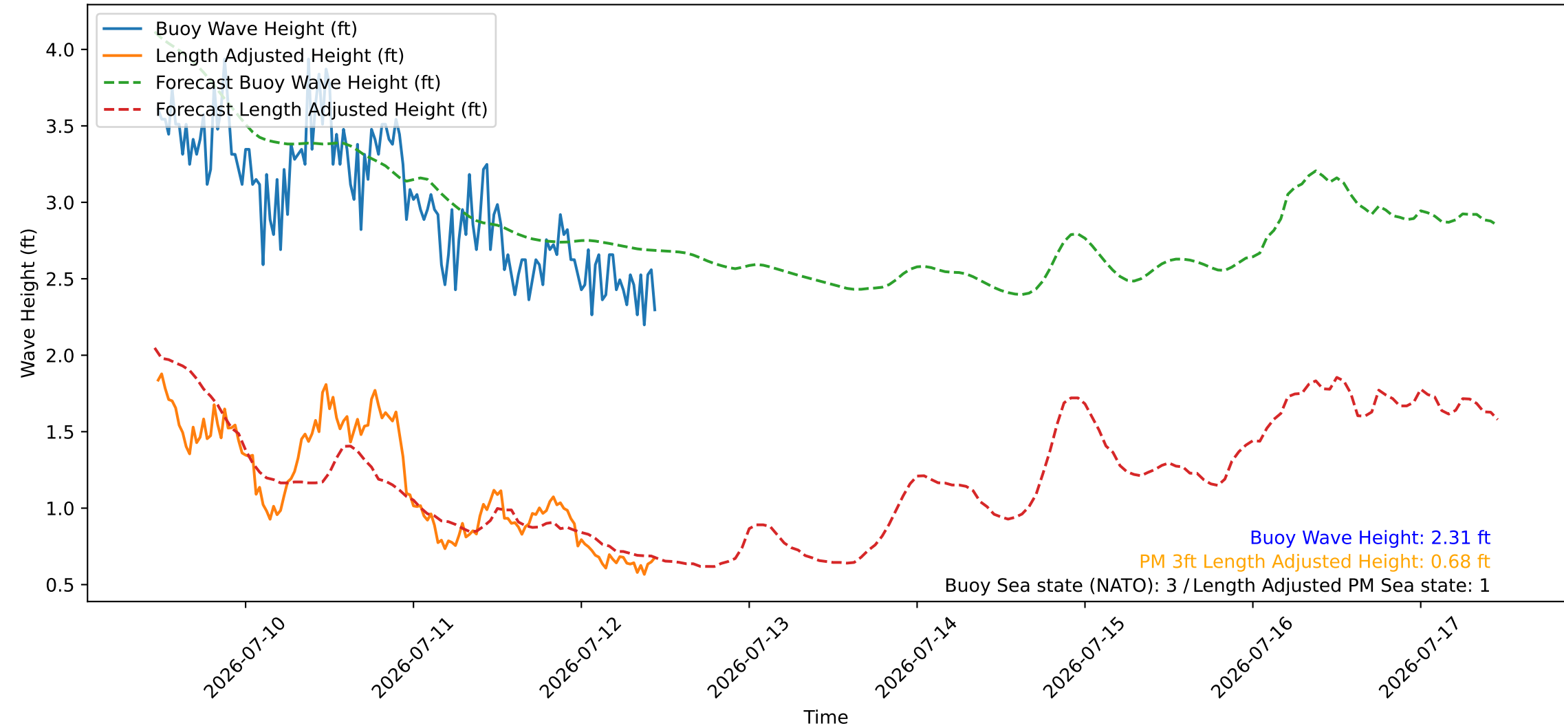
Wave Heights over Time for Red Beach at 2026-07-12 11:20:47
