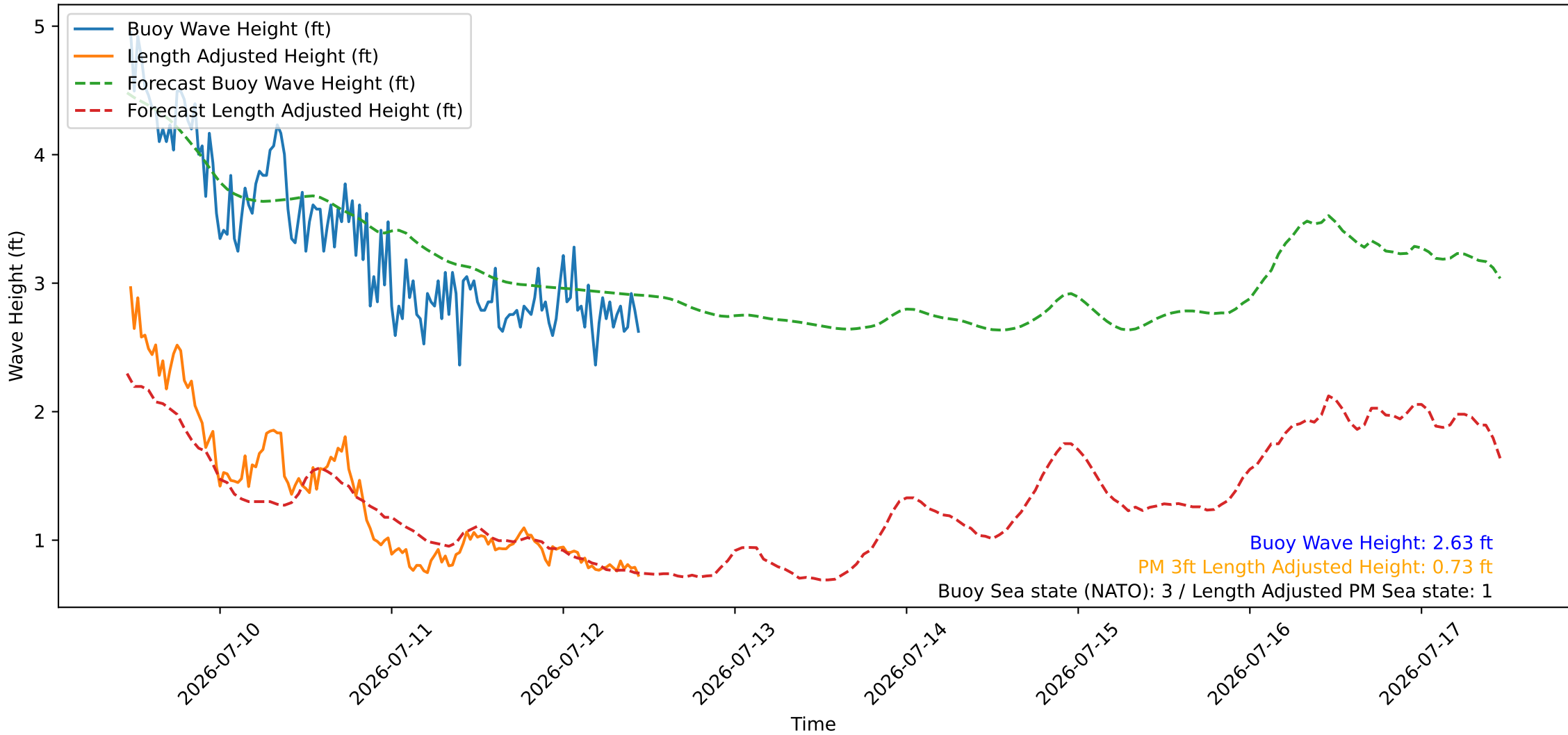
Wave Heights over Time for Oceanside Harbor at 2026-07-12 11:20:26
