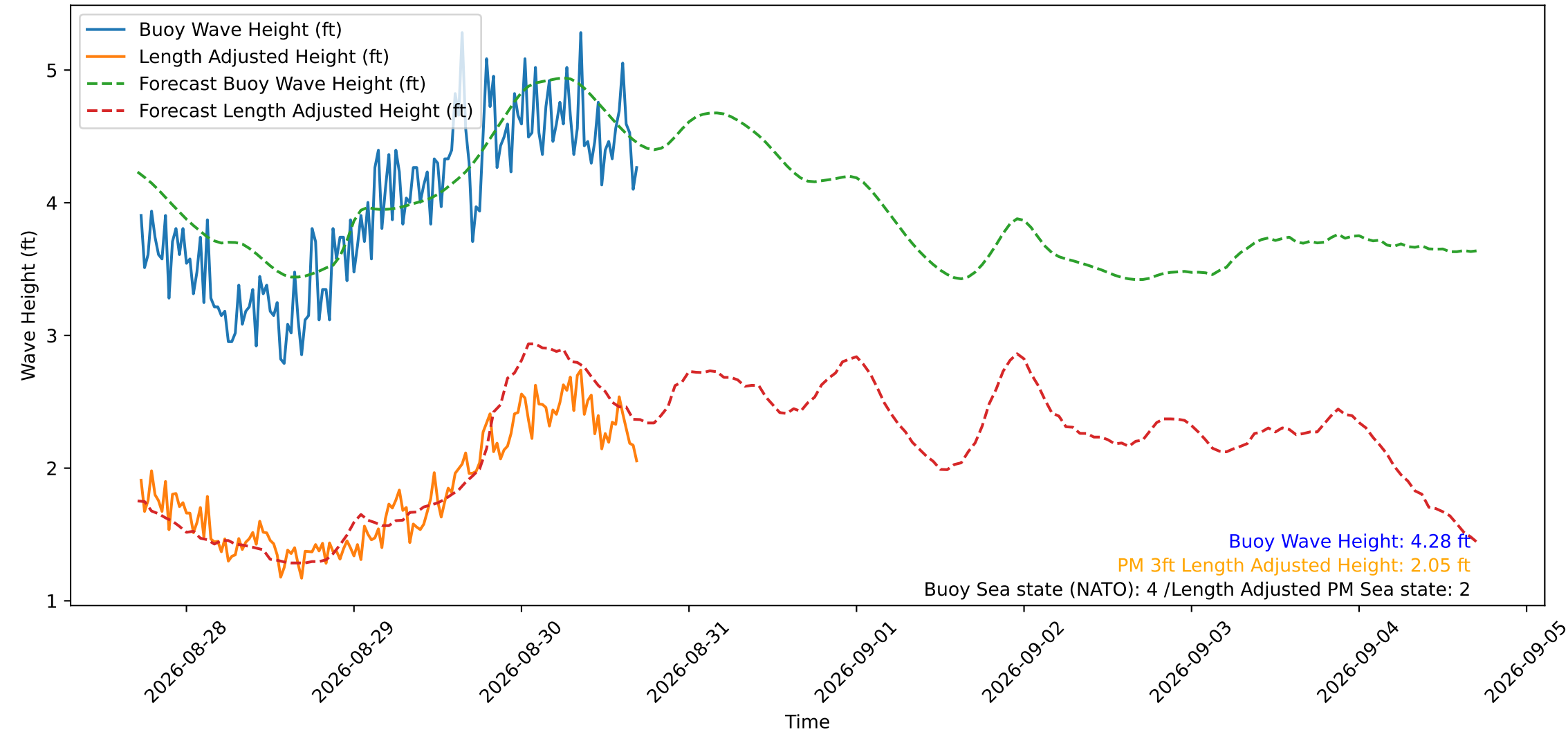
Wave Heights over Time for Oceanside Harbor at 2026-08-30 17:20:30
