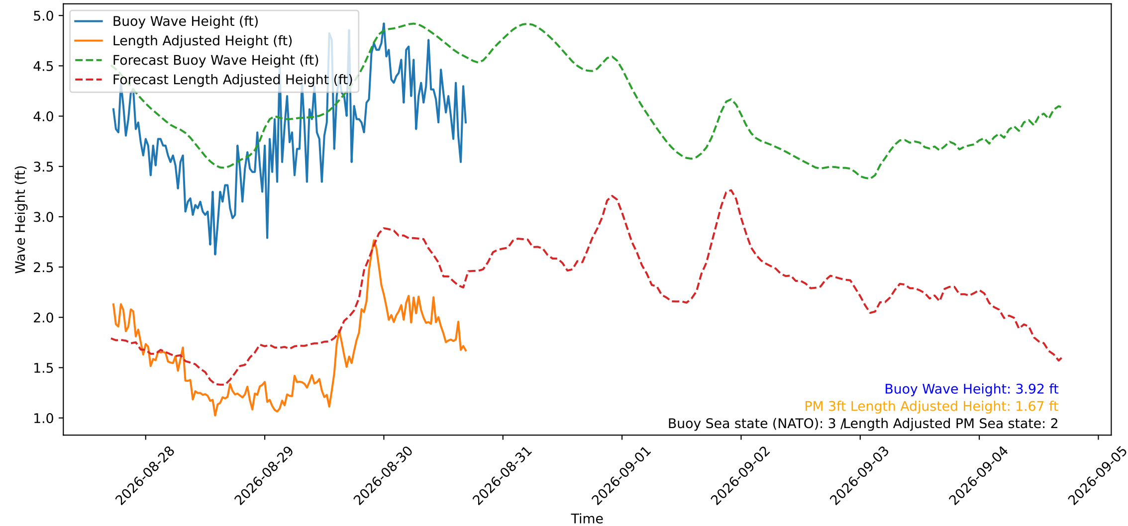
Wave Heights over Time for Green Beach at 2026-08-30 17:21:14
