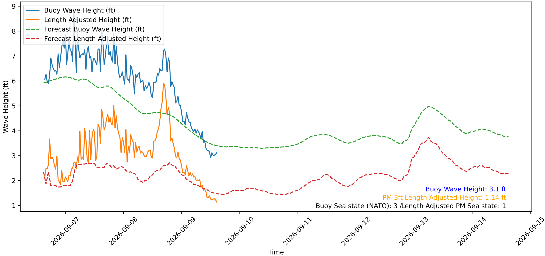
Wave Heights over Time for Green Beach at 2026-09-09 15:21:15
