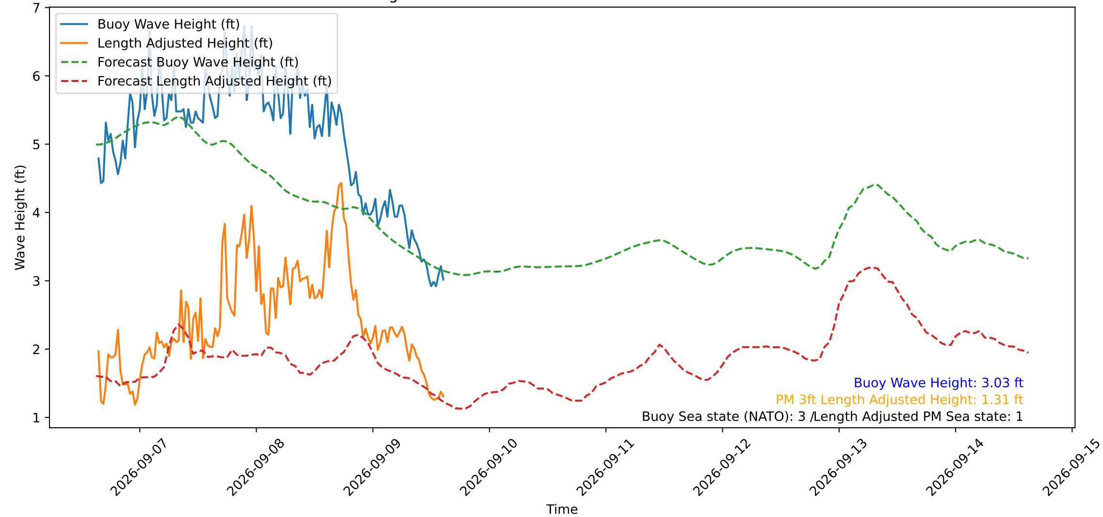
Wave Heights over Time for Red Beach at 2026-09-09 15:20:51
