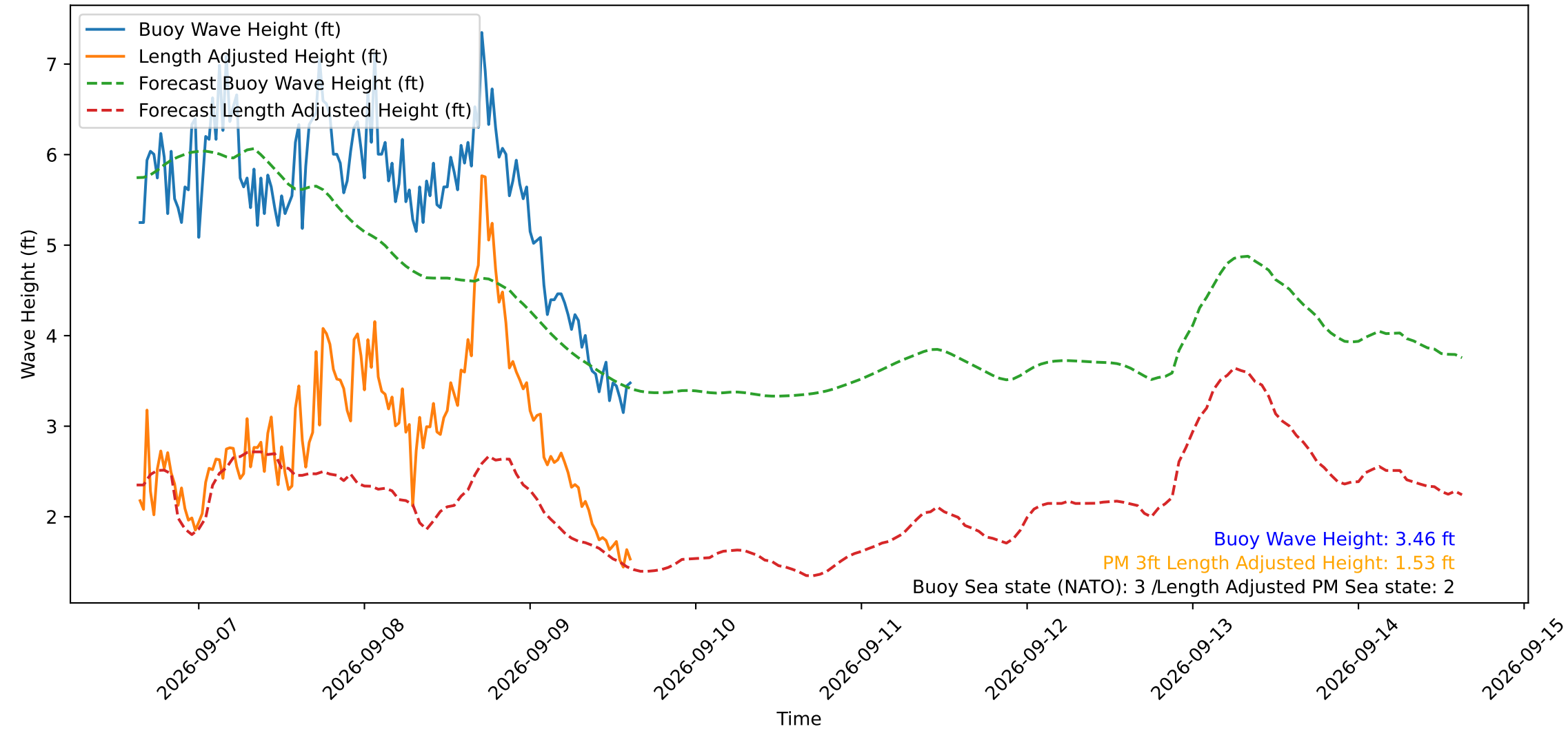
Wave Heights over Time for Oceanside Harbor at 2026-09-09 15:20:31
