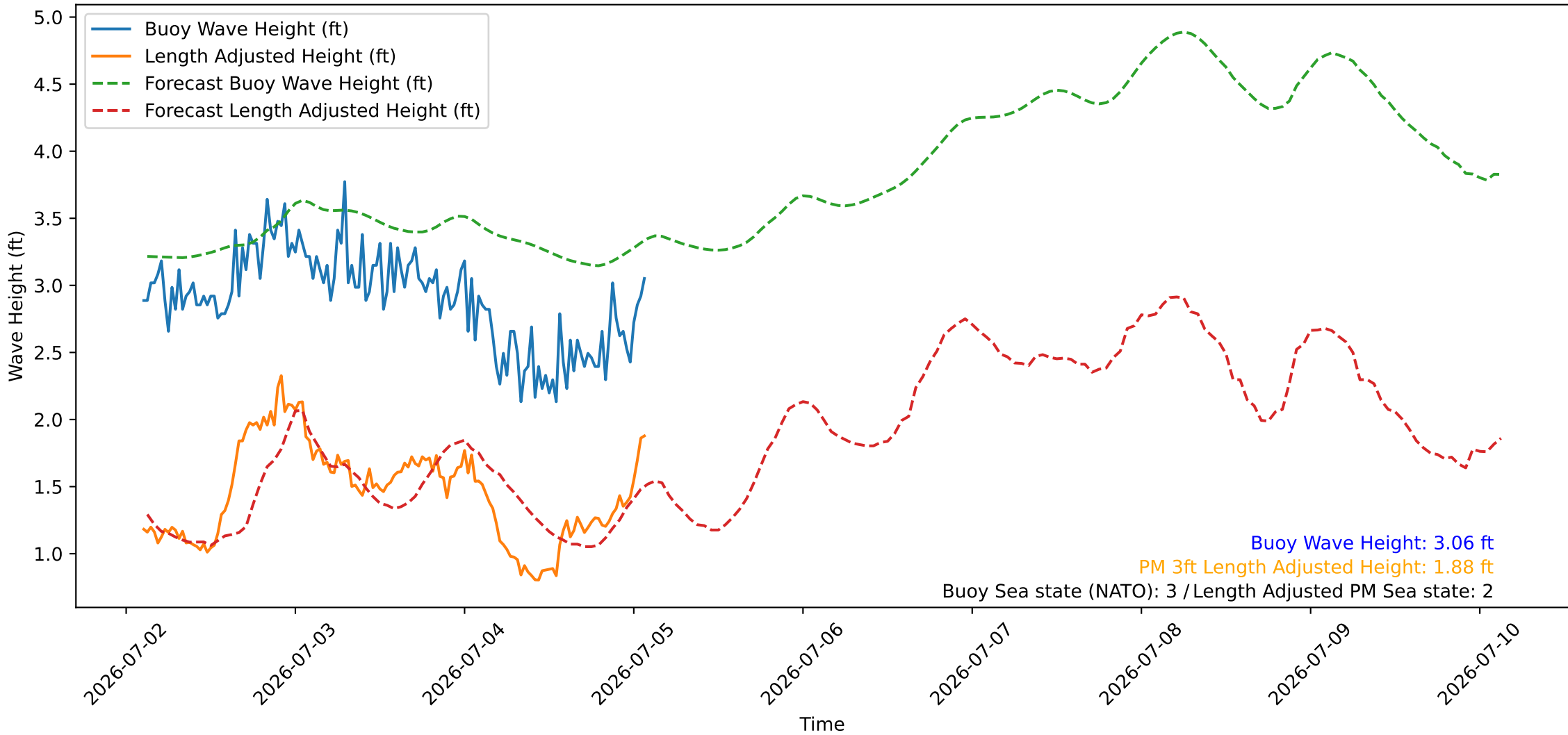
Wave Heights over Time for Oceanside Harbor at 2026-07-05 02:30:26
