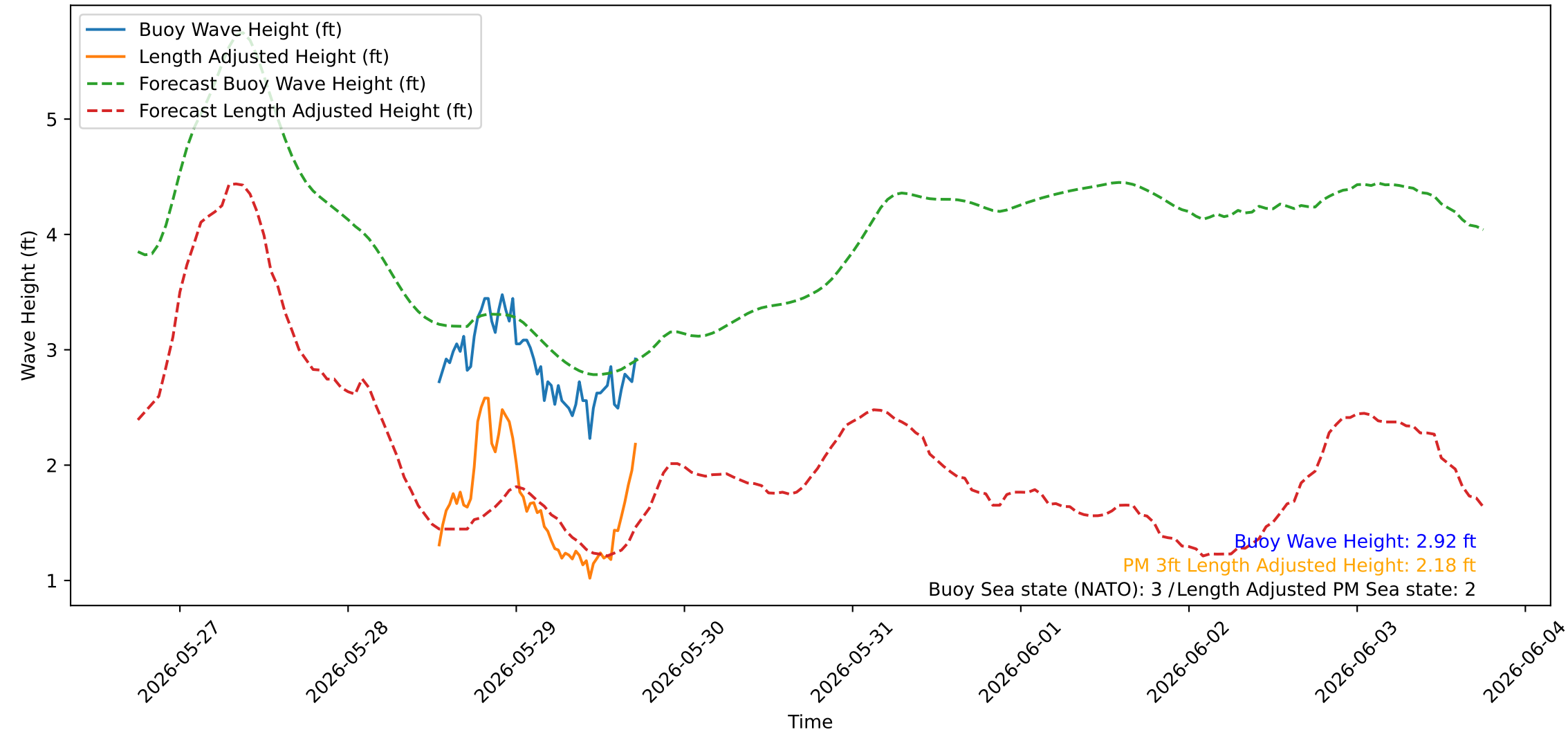
Wave Heights over Time for Oceanside Harbor at 2026-05-29 17:50:22
