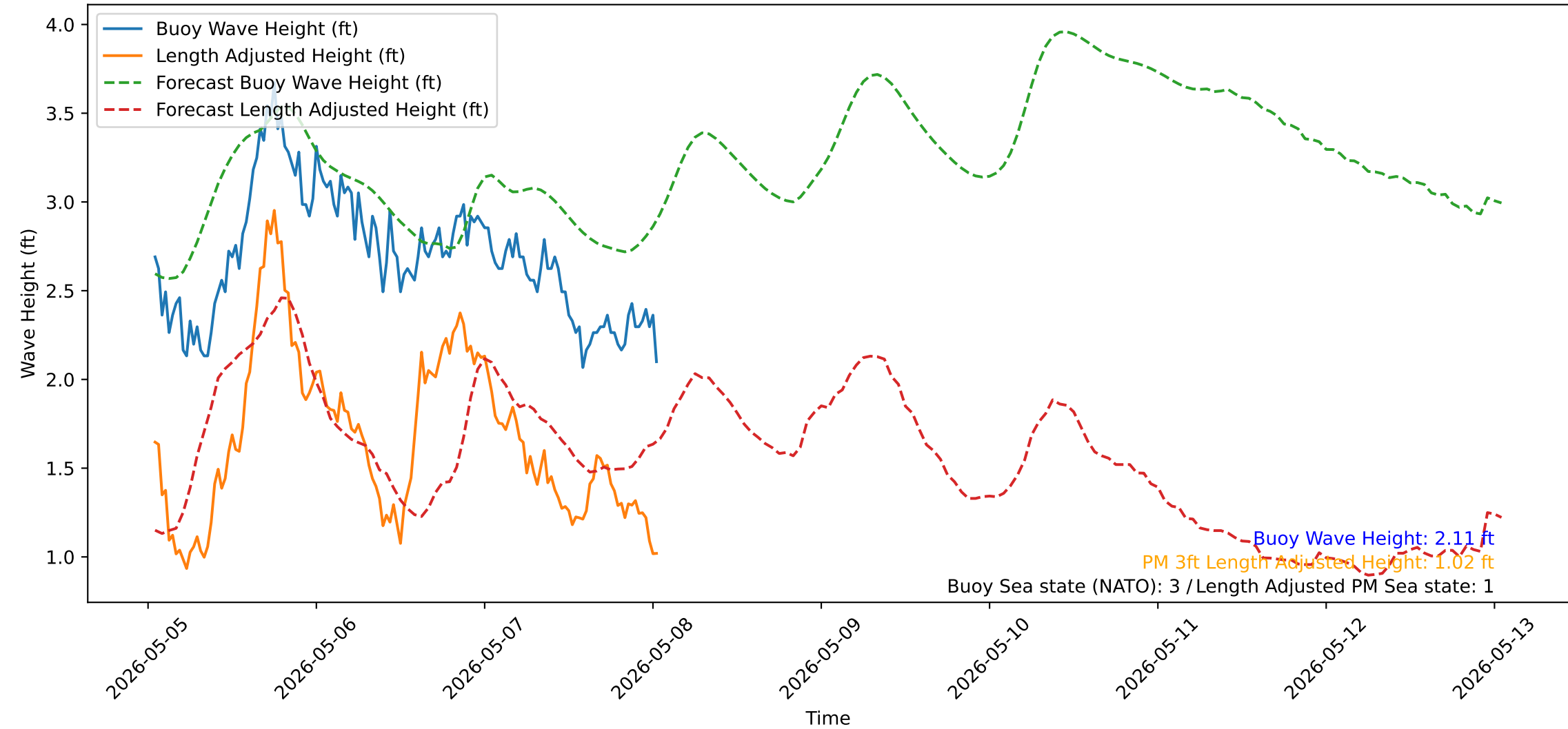
Wave Heights over Time for Green Beach at 2026-05-08 01:11:13
