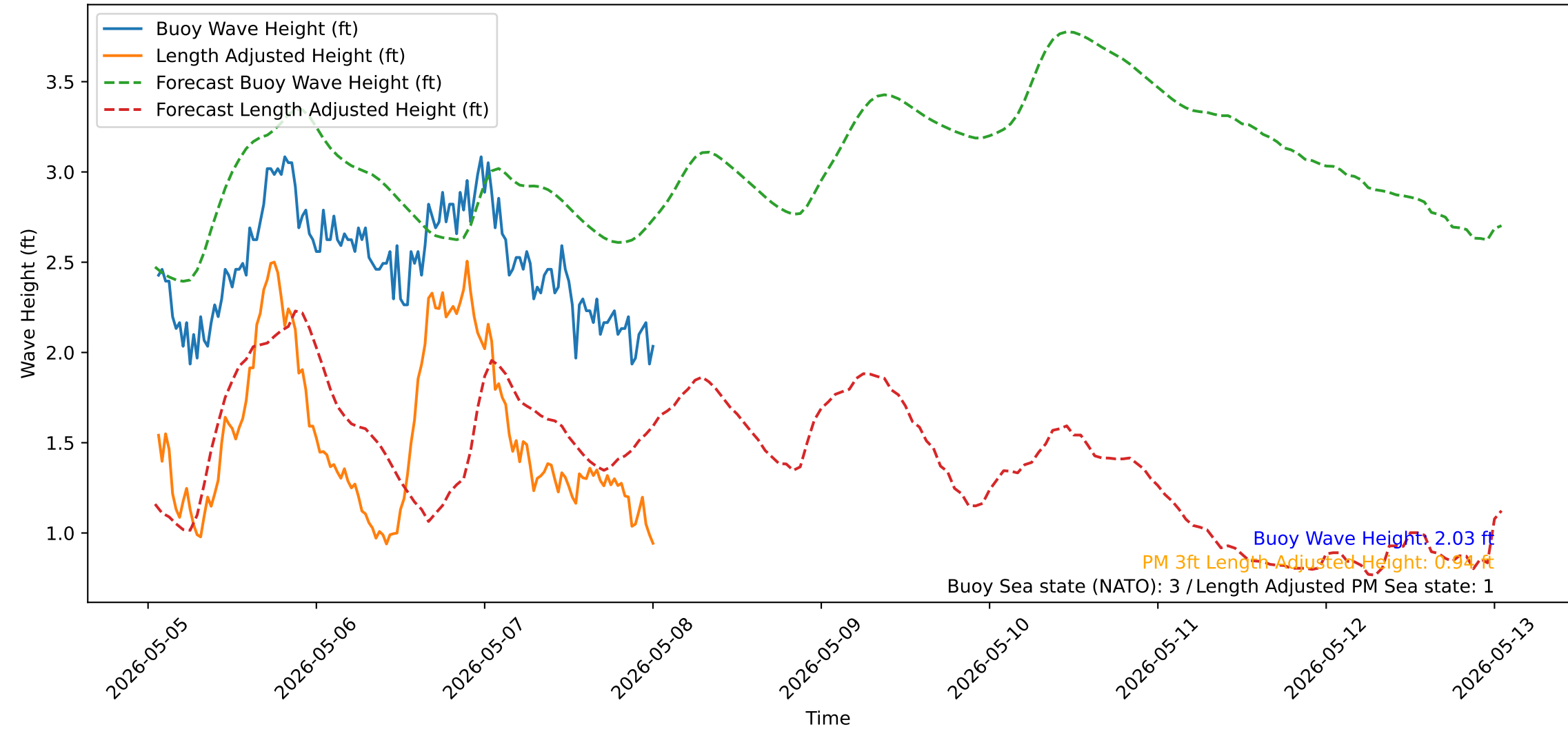
Wave Heights over Time for Red Beach at 2026-05-08 01:10:50
