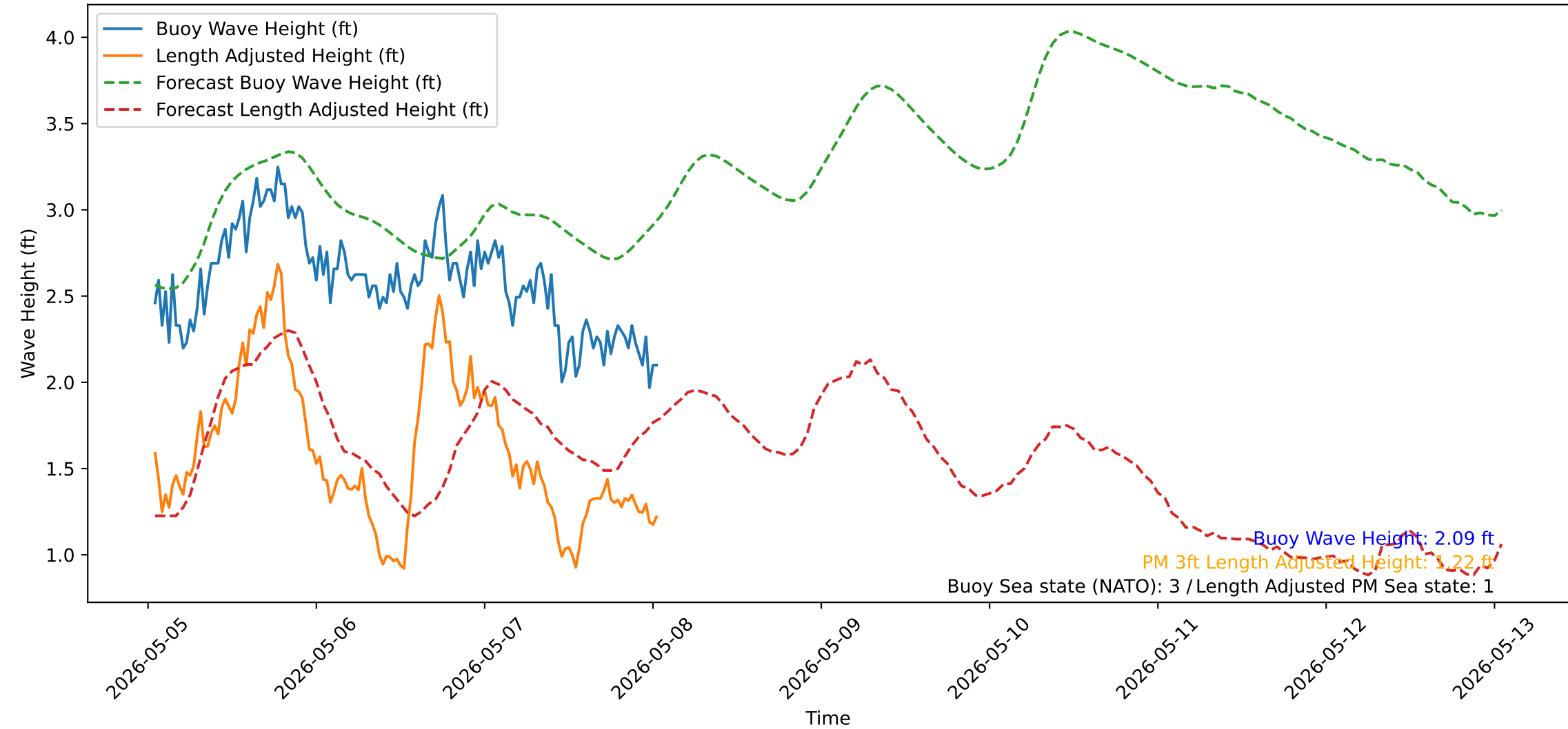
Wave Heights over Time for Oceanside Harbor at 2026-05-08 01:10:31
