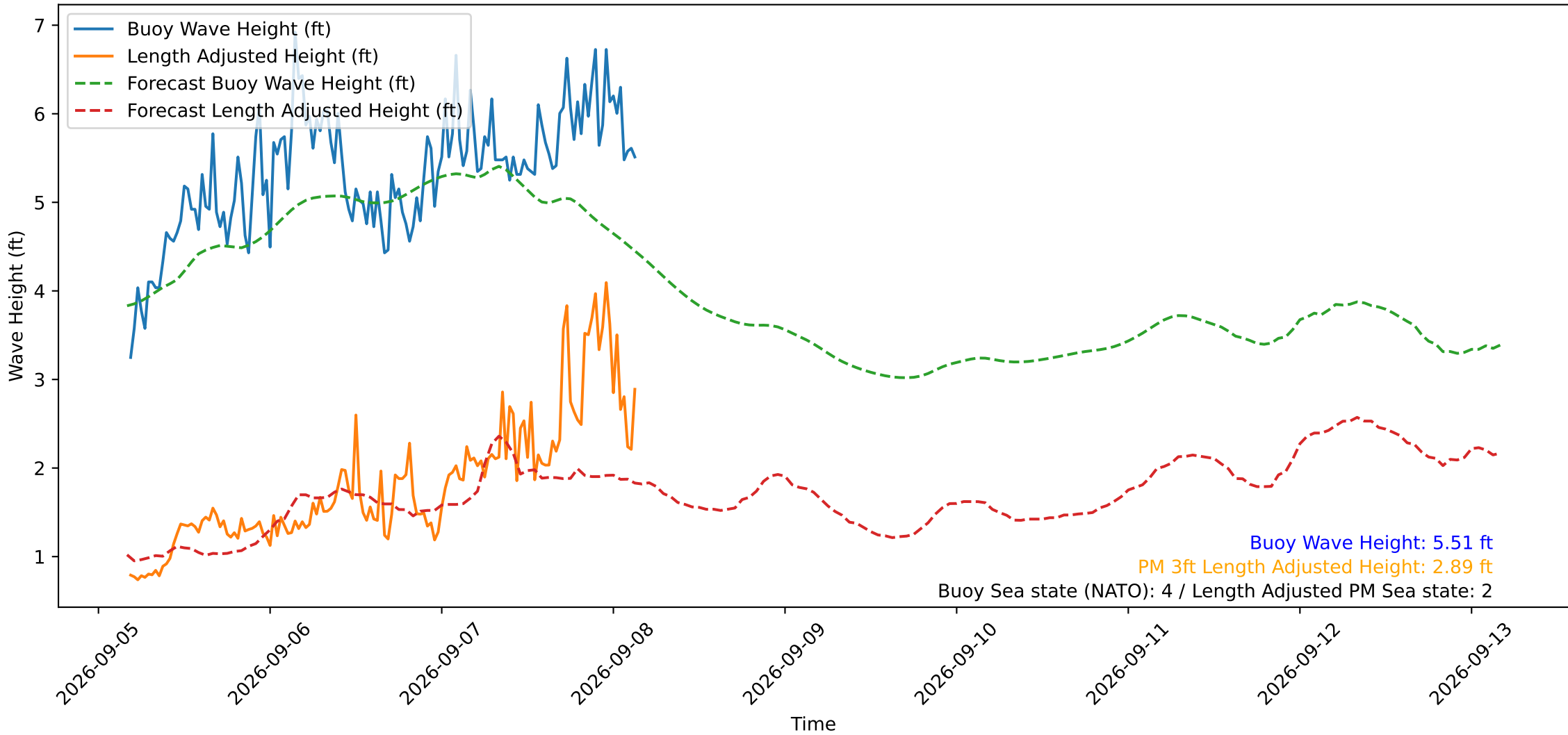
Wave Heights over Time for Red Beach at 2026-09-08 04:00:49
