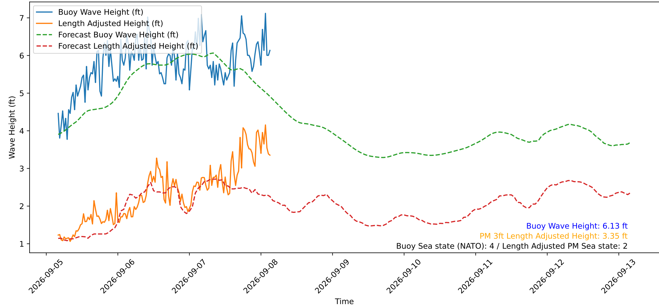
Wave Heights over Time for Oceanside Harbor at 2026-09-08 04:00:29
