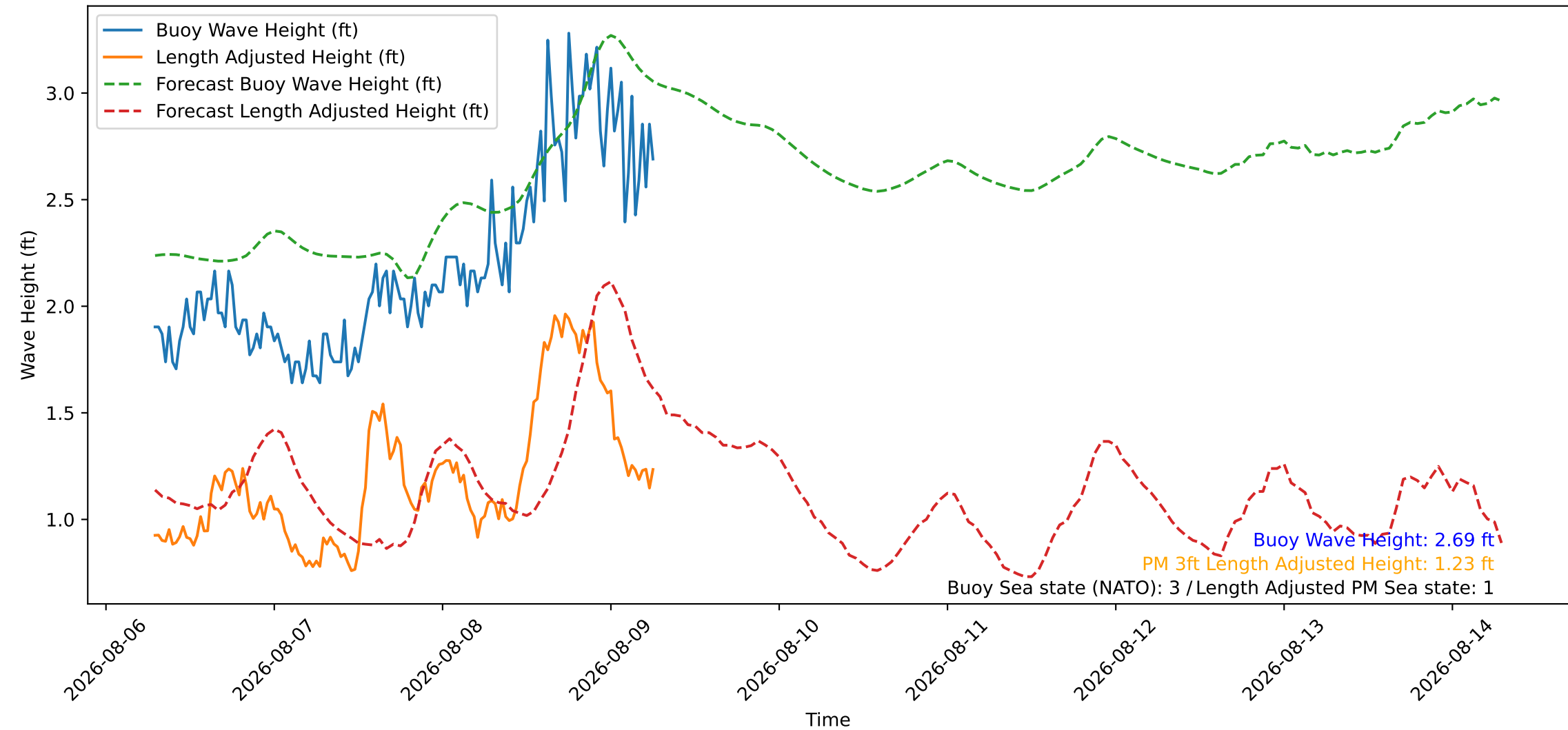
Wave Heights over Time for Oceanside Harbor at 2026-08-09 06:50:26
