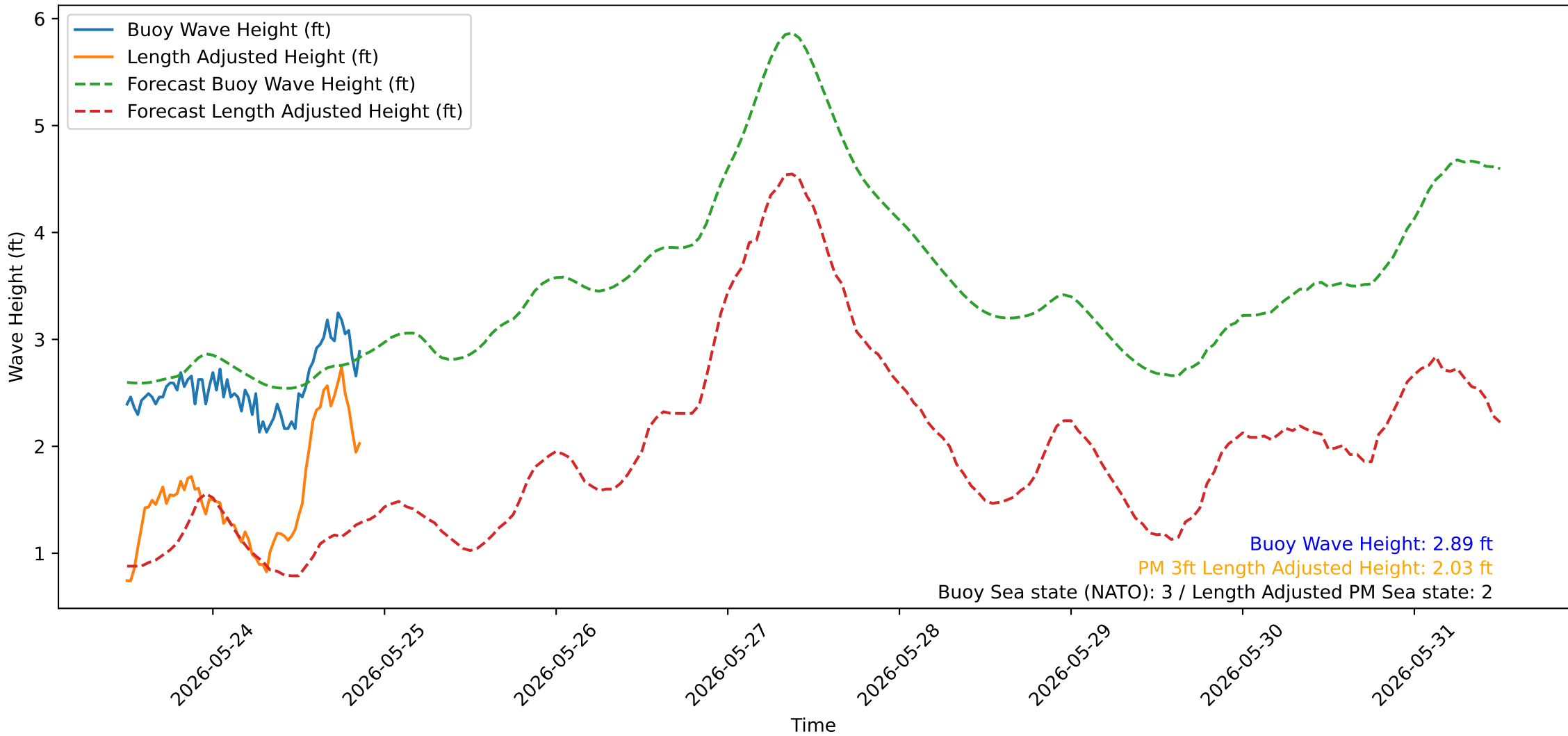
Wave Heights over Time for Oceanside Harbor at 2026-05-26 11:50:27
