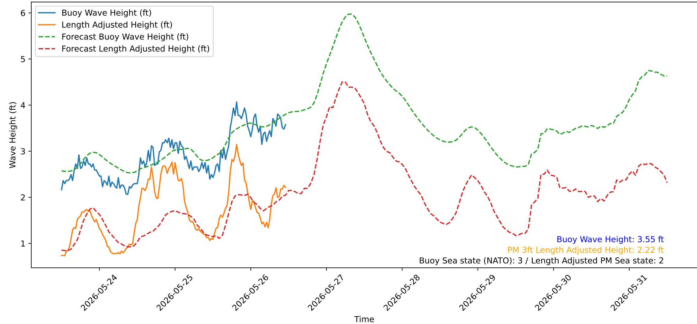
Wave Heights over Time for Green Beach at 2026-05-26 11:51:10
