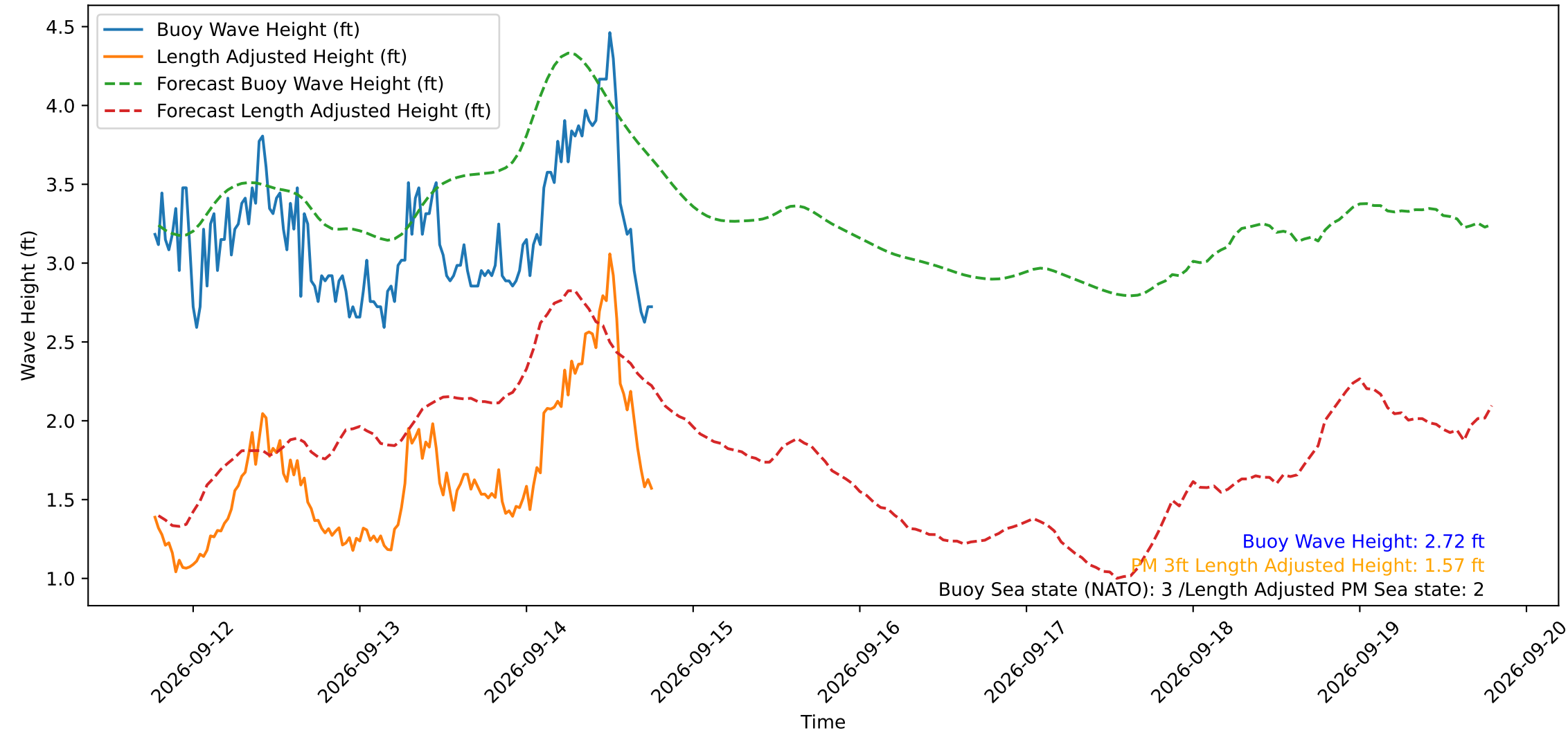
Wave Heights over Time for Oceanside Harbor at 2026-09-14 18:40:29
