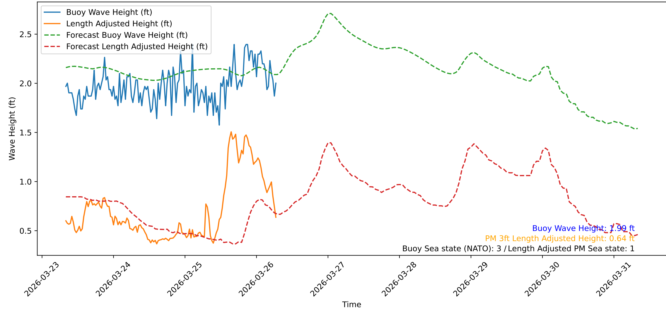
Wave Heights over Time for Red Beach at 2026-03-26 07:30:47
