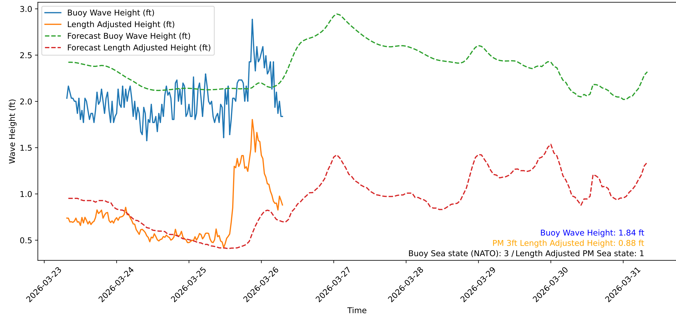
Wave Heights over Time for Oceanside Harbor at 2026-03-26 07:30:31
