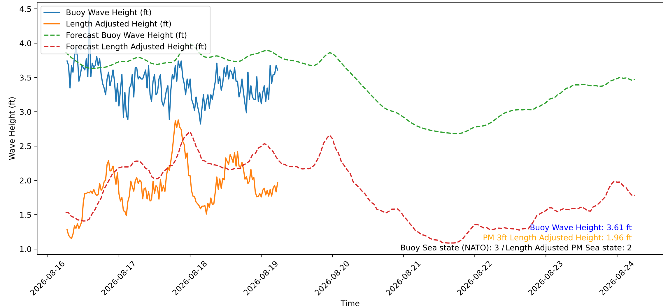
Wave Heights over Time for Oceanside Harbor at 2026-08-19 06:20:26
