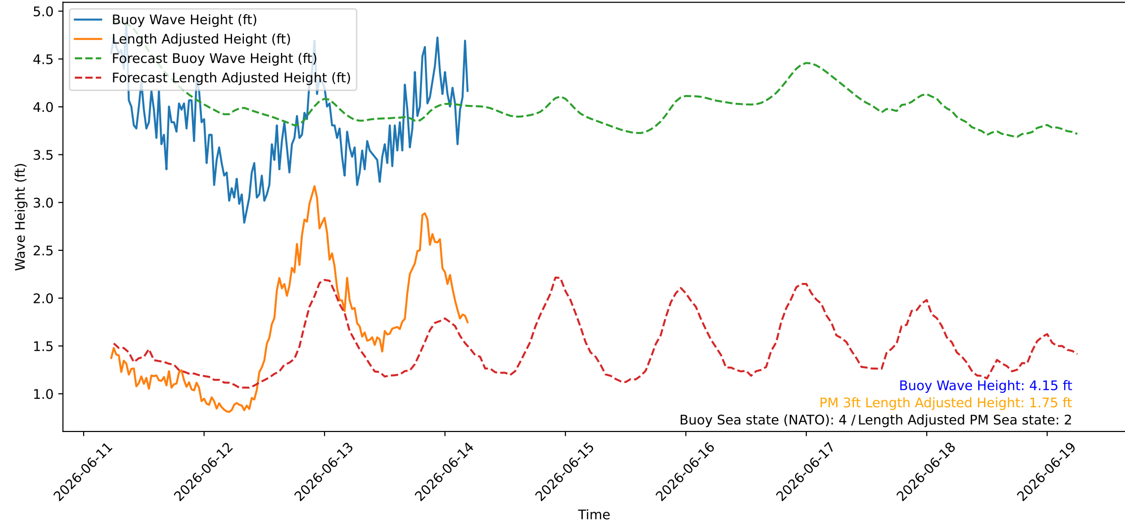
Wave Heights over Time for Oceanside Harbor at 2026-06-14 05:30:26
