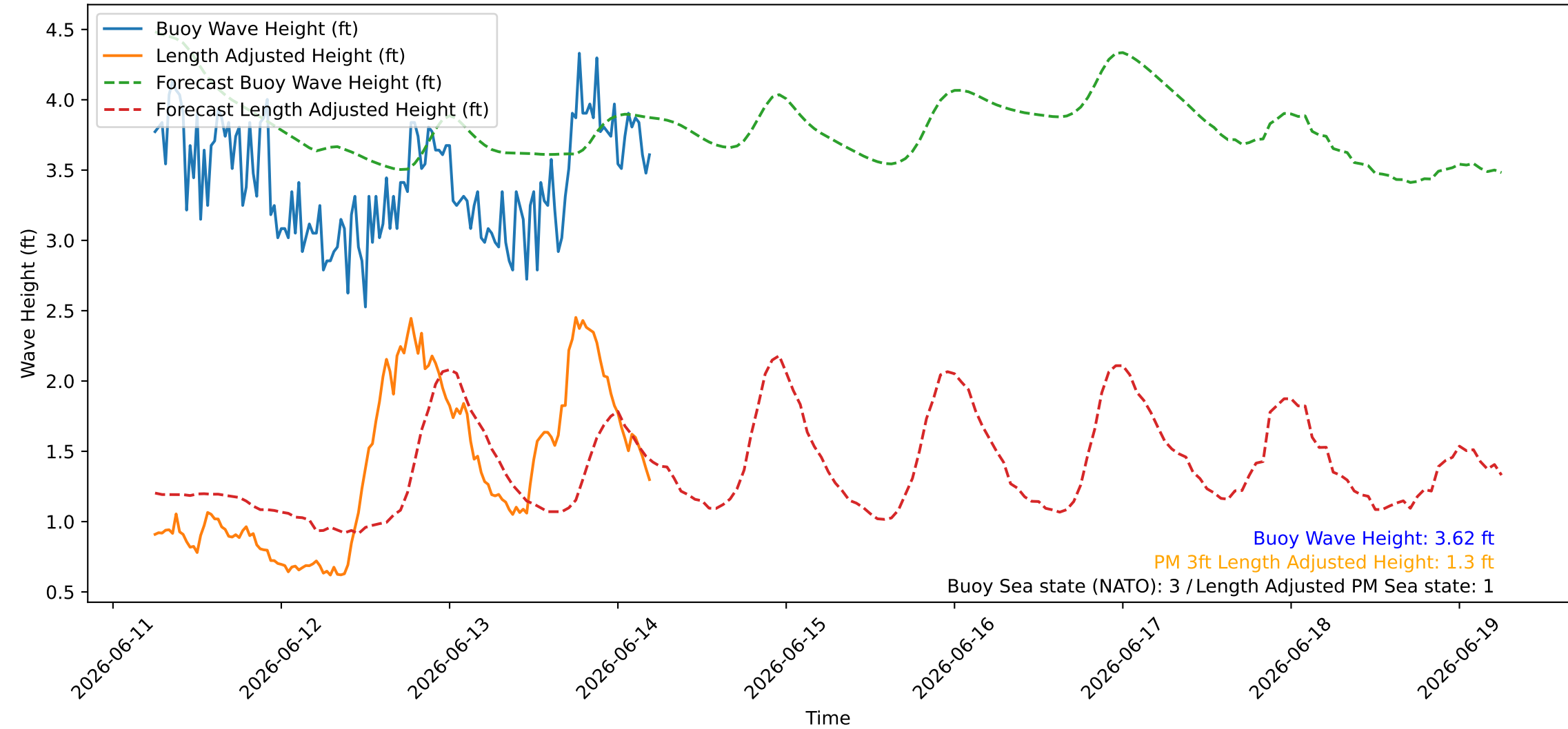
Wave Heights over Time for Red Beach at 2026-06-14 05:30:46
