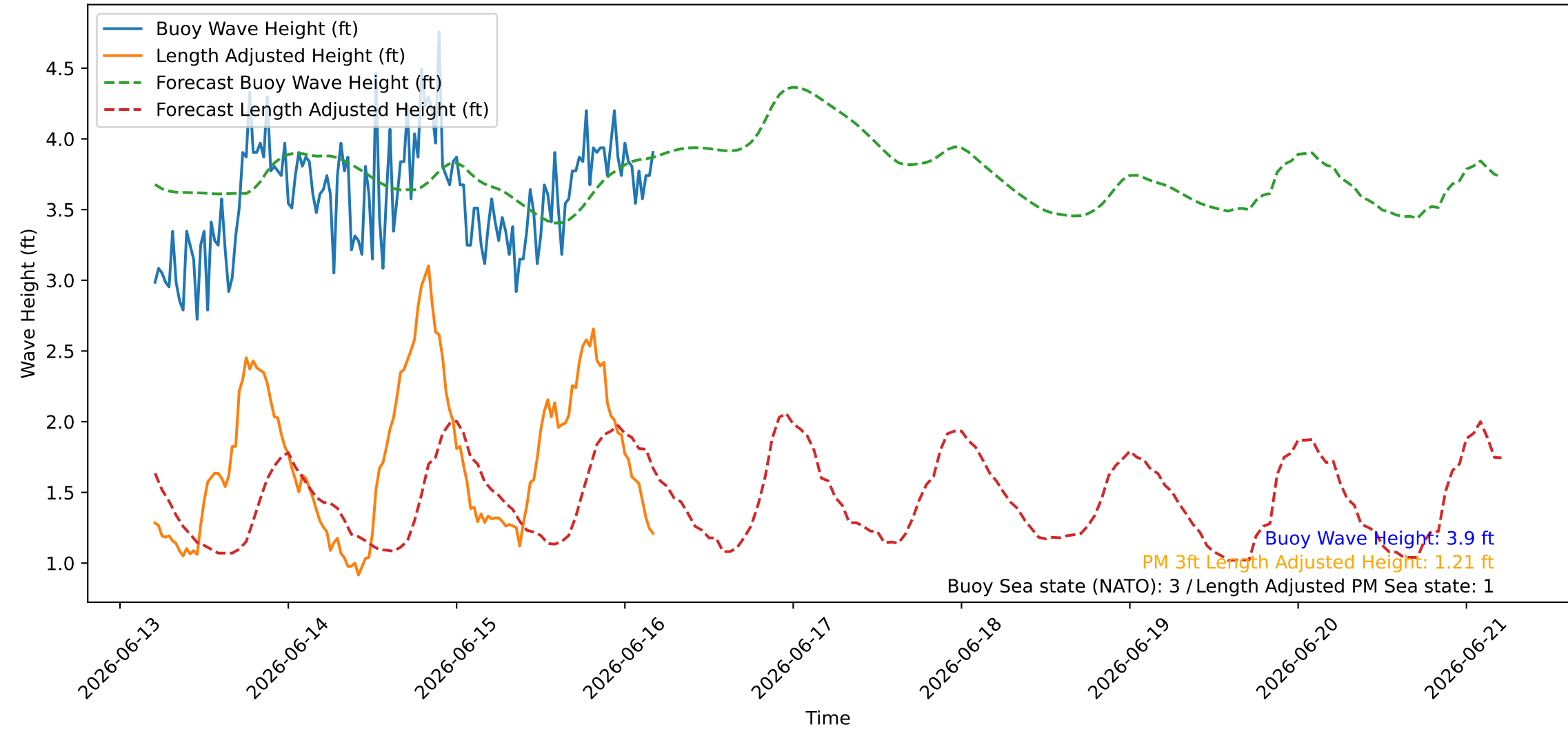
Wave Heights over Time for Red Beach at 2026-06-16 04:40:45
