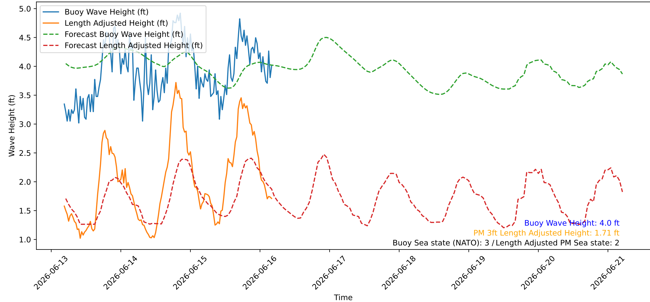
Wave Heights over Time for Green Beach at 2026-06-16 04:41:08
