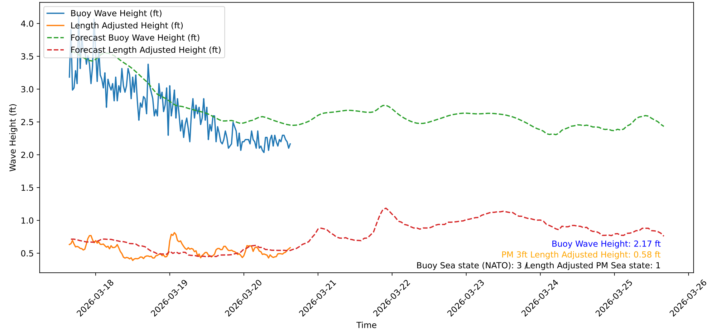
Wave Heights over Time for Green Beach at 2026-03-20 15:41:10
