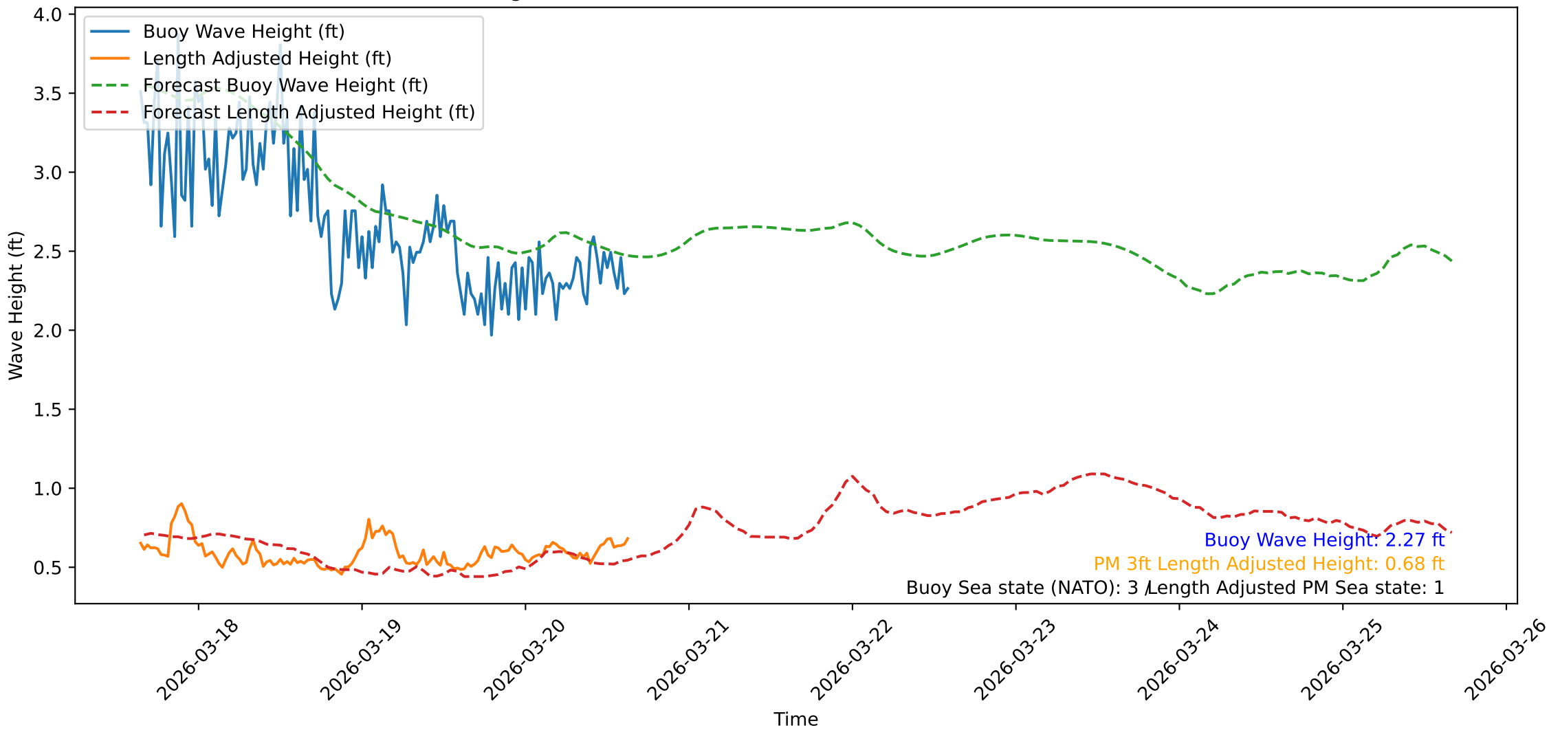
Wave Heights over Time for Oceanside Harbor at 2026-03-20 15:40:31
