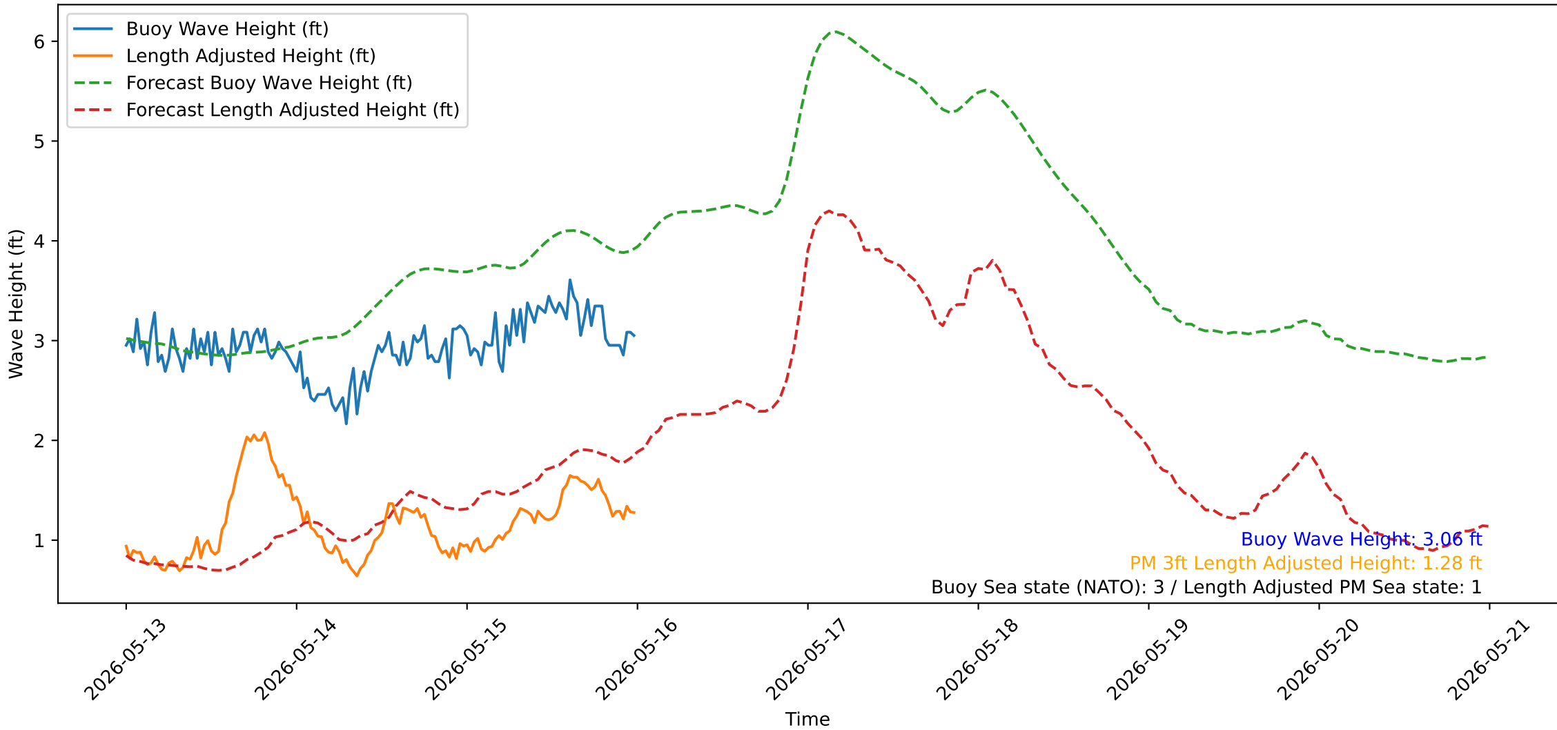
Wave Heights over Time for Oceanside Harbor at 2026-05-16 00:00:31
