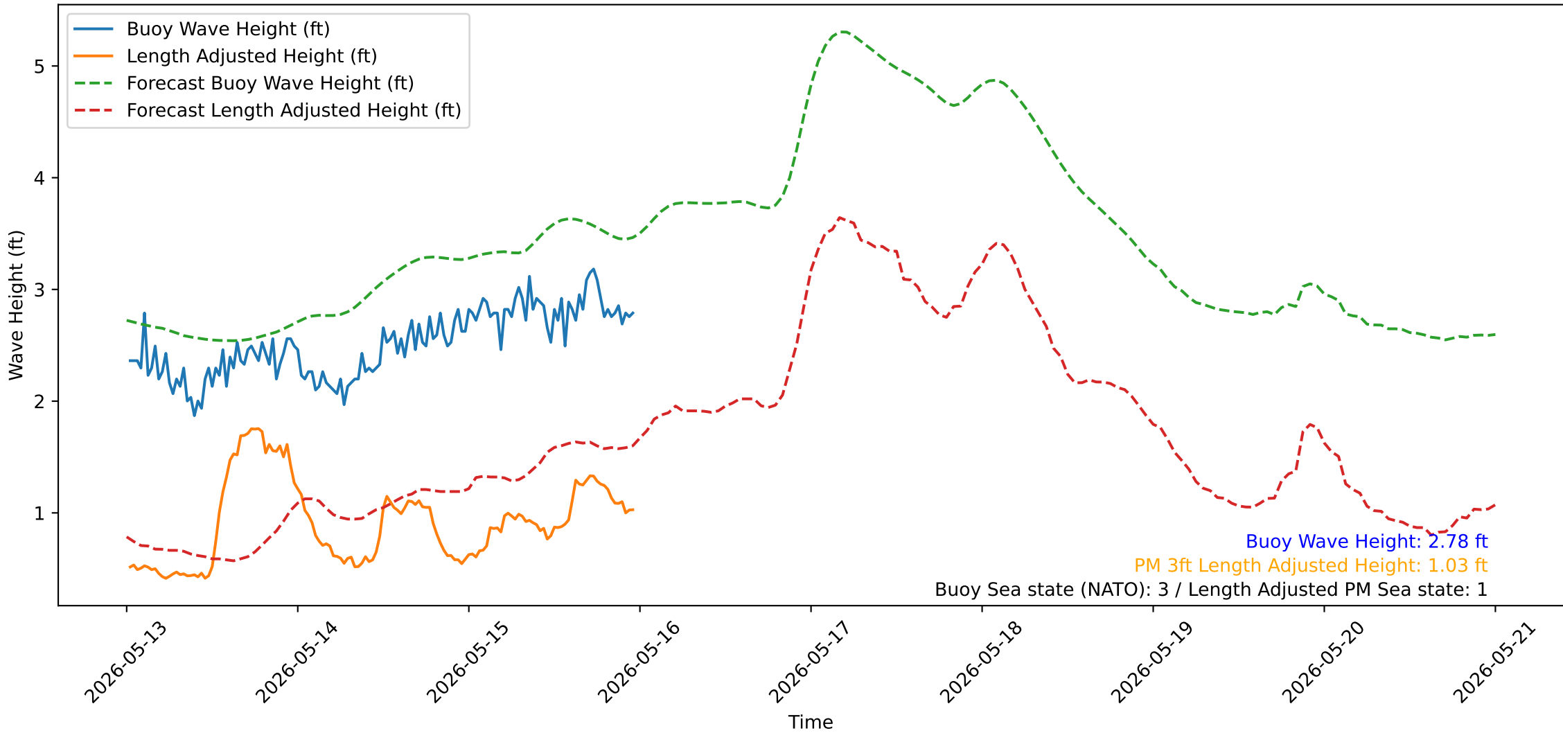
Wave Heights over Time for Red Beach at 2026-05-16 00:00:50
