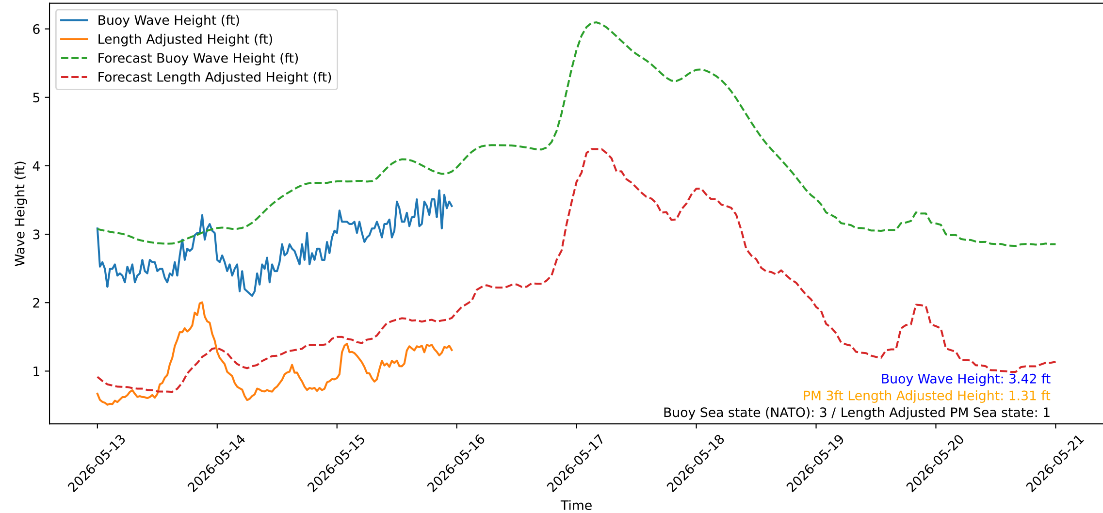
Wave Heights over Time for Green Beach at 2026-05-16 00:01:13
