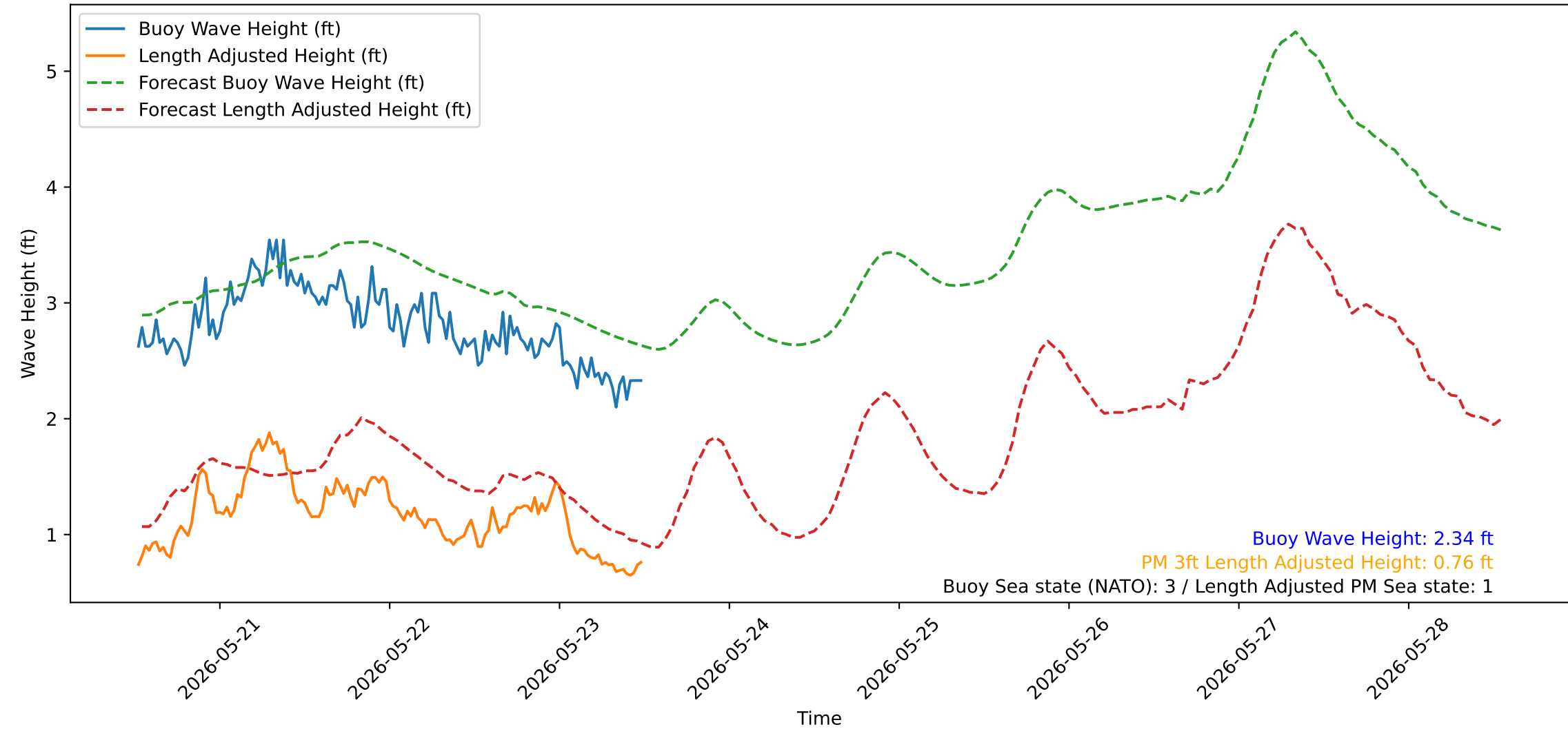
Wave Heights over Time for Green Beach at 2026-05-23 12:31:13
