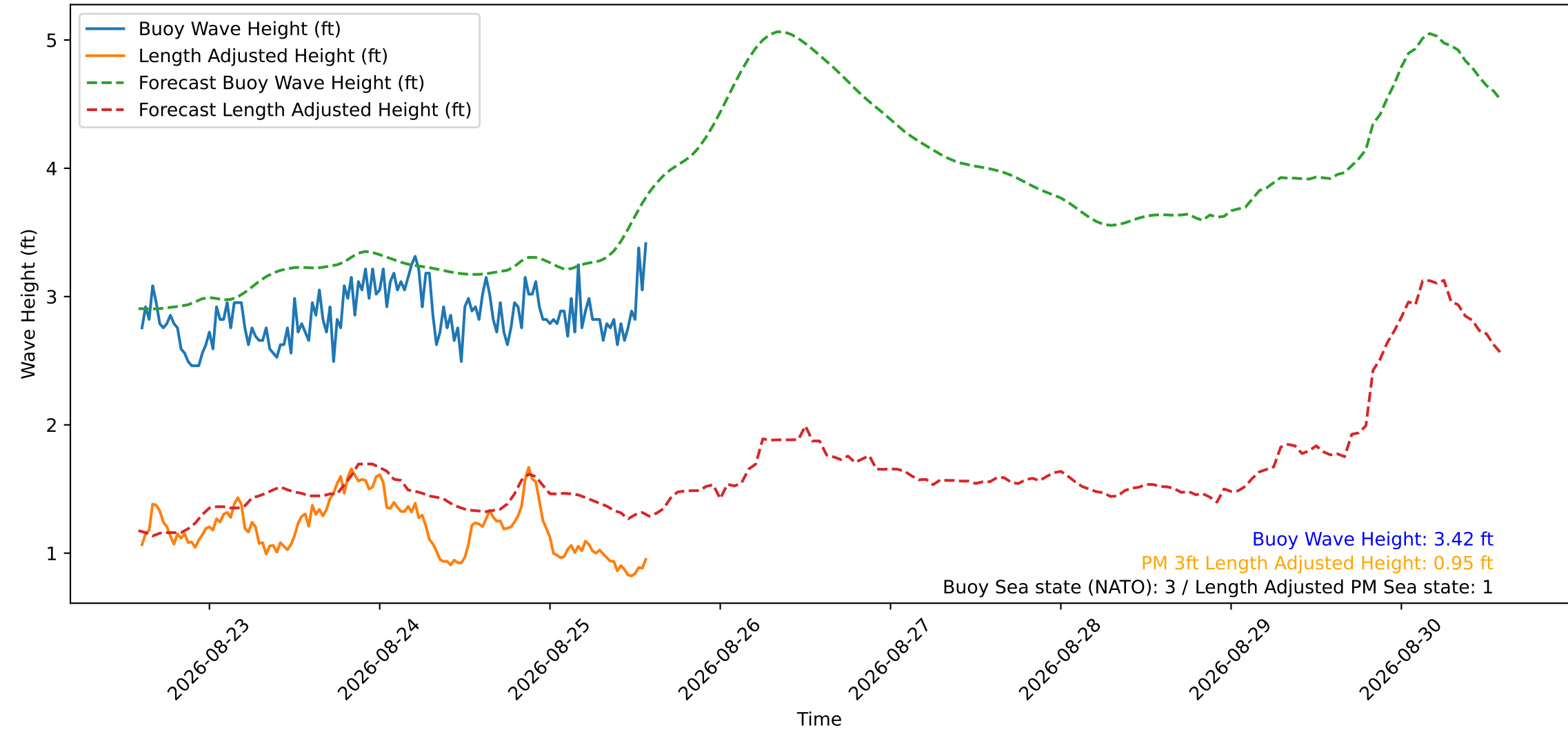
Wave Heights over Time for Green Beach at 2026-08-25 14:21:15
