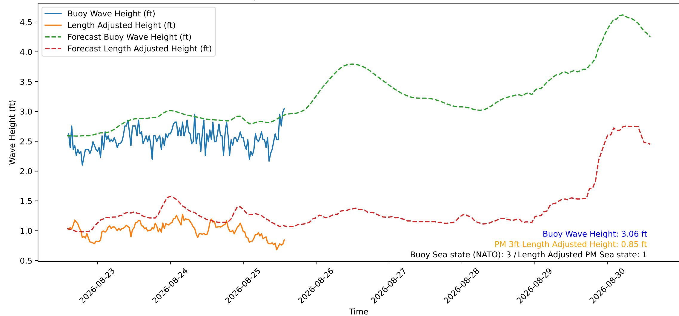
Wave Heights over Time for Red Beach at 2026-08-25 14:20:50
