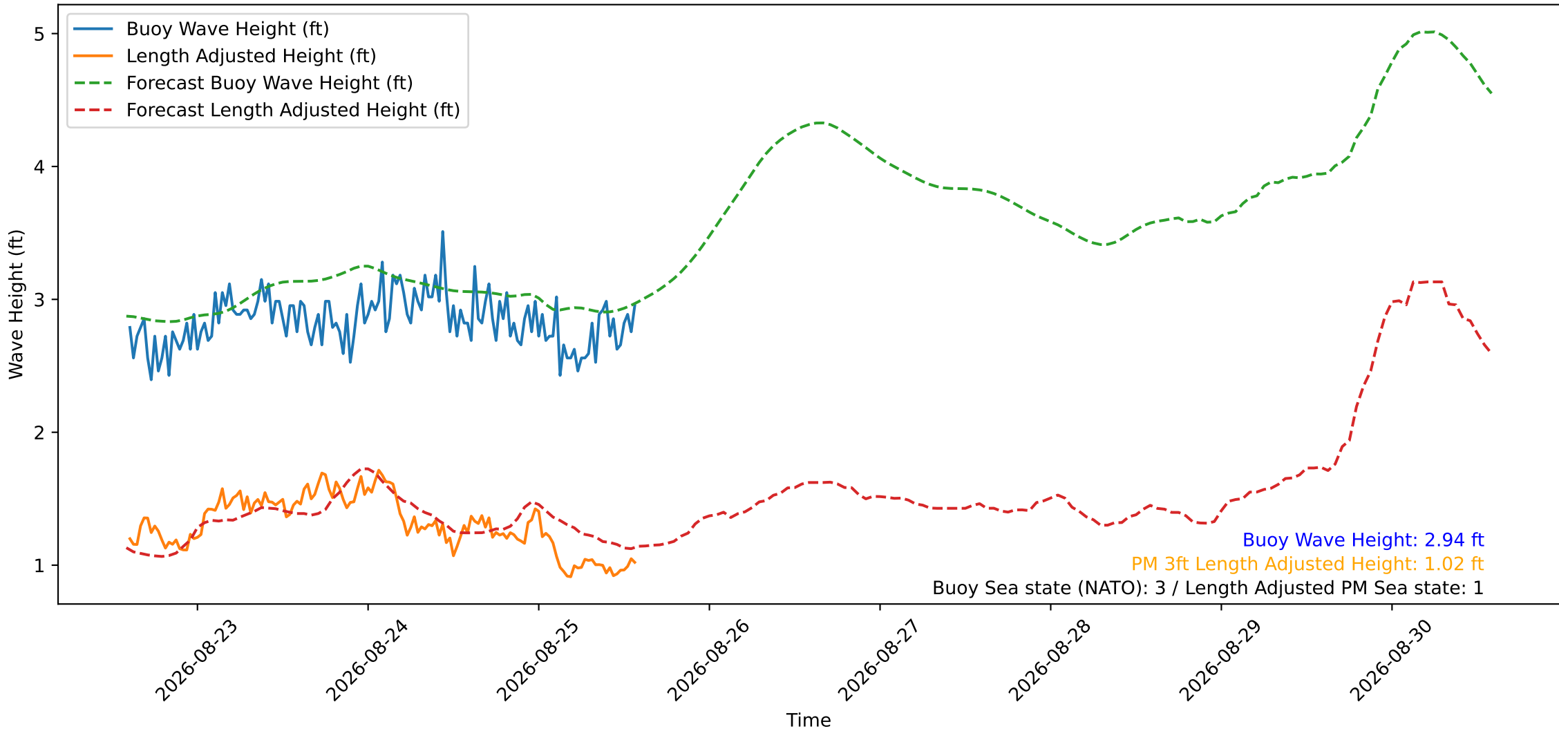
Wave Heights over Time for Oceanside Harbor at 2026-08-25 14:20:30
