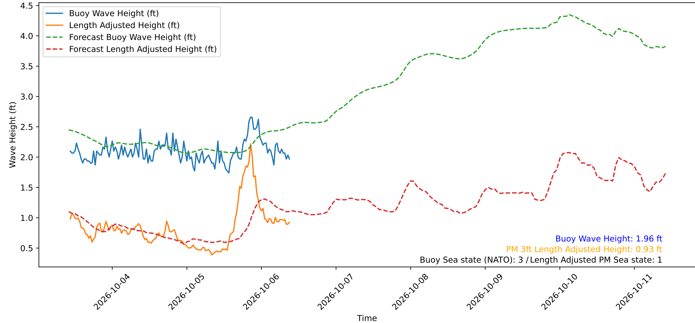
Wave Heights over Time for Red Beach at 2026-10-06 10:00:49
