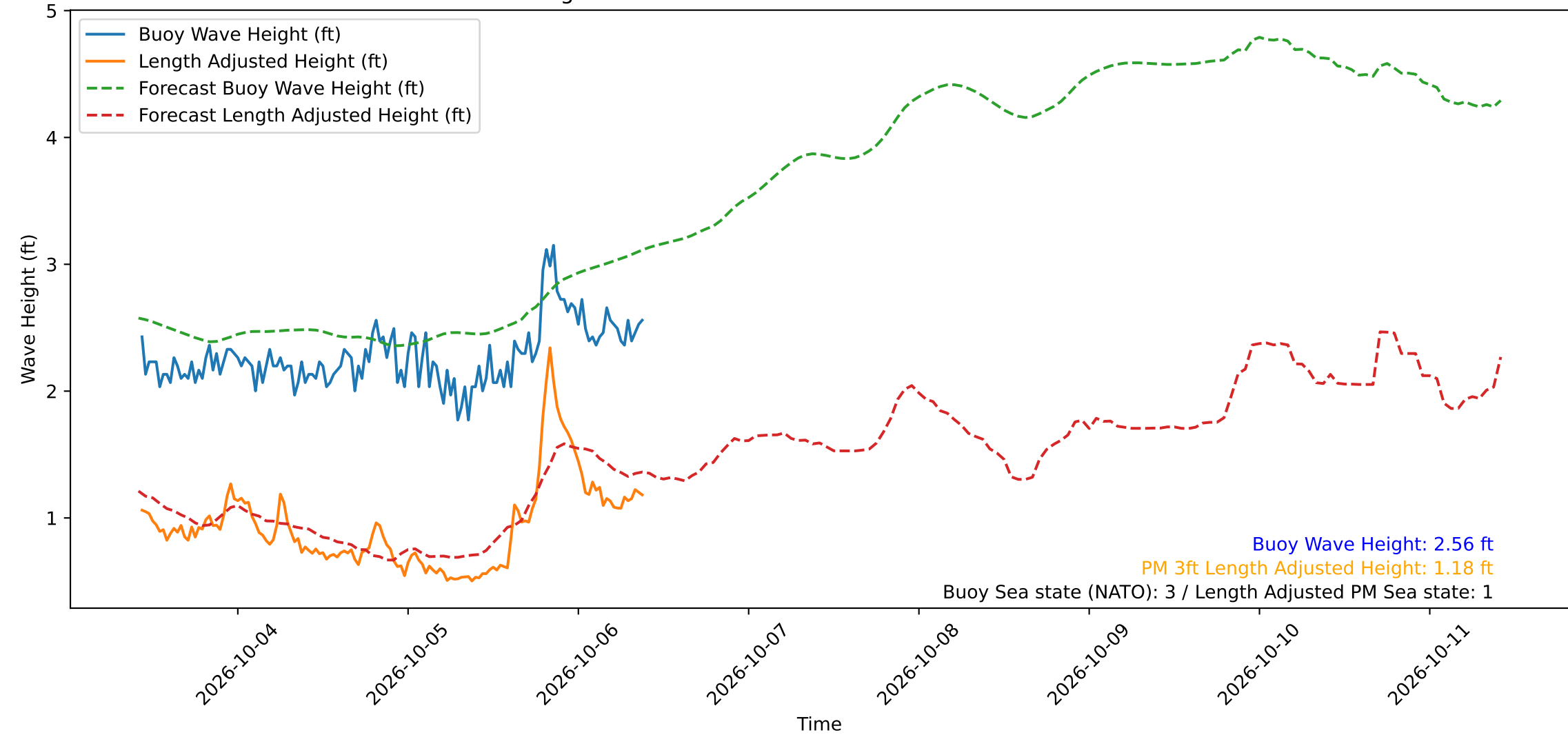
Wave Heights over Time for Green Beach at 2026-10-06 10:01:11
