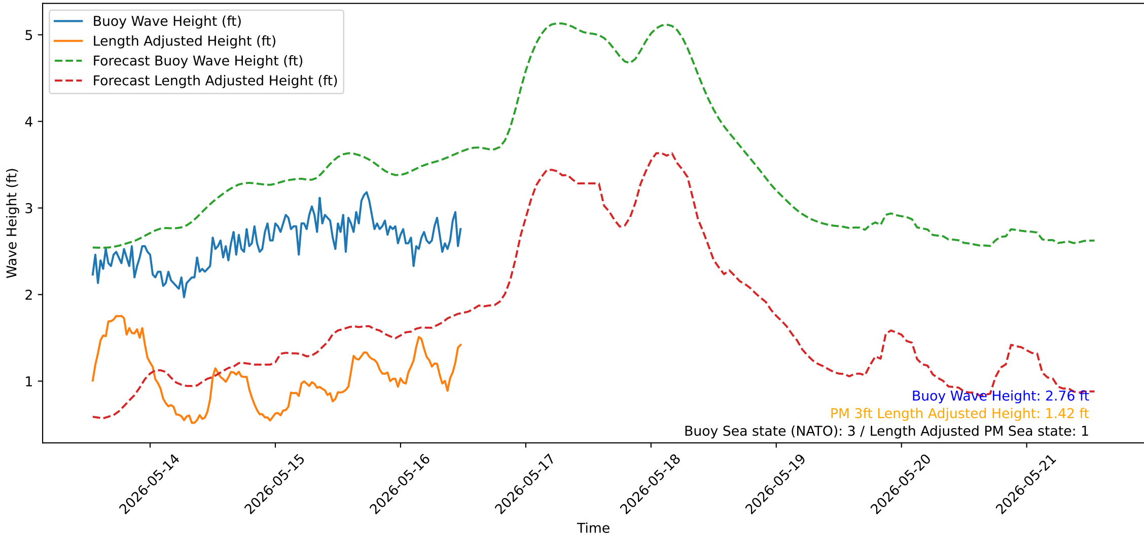
Wave Heights over Time for Red Beach at 2026-05-16 12:30:51
