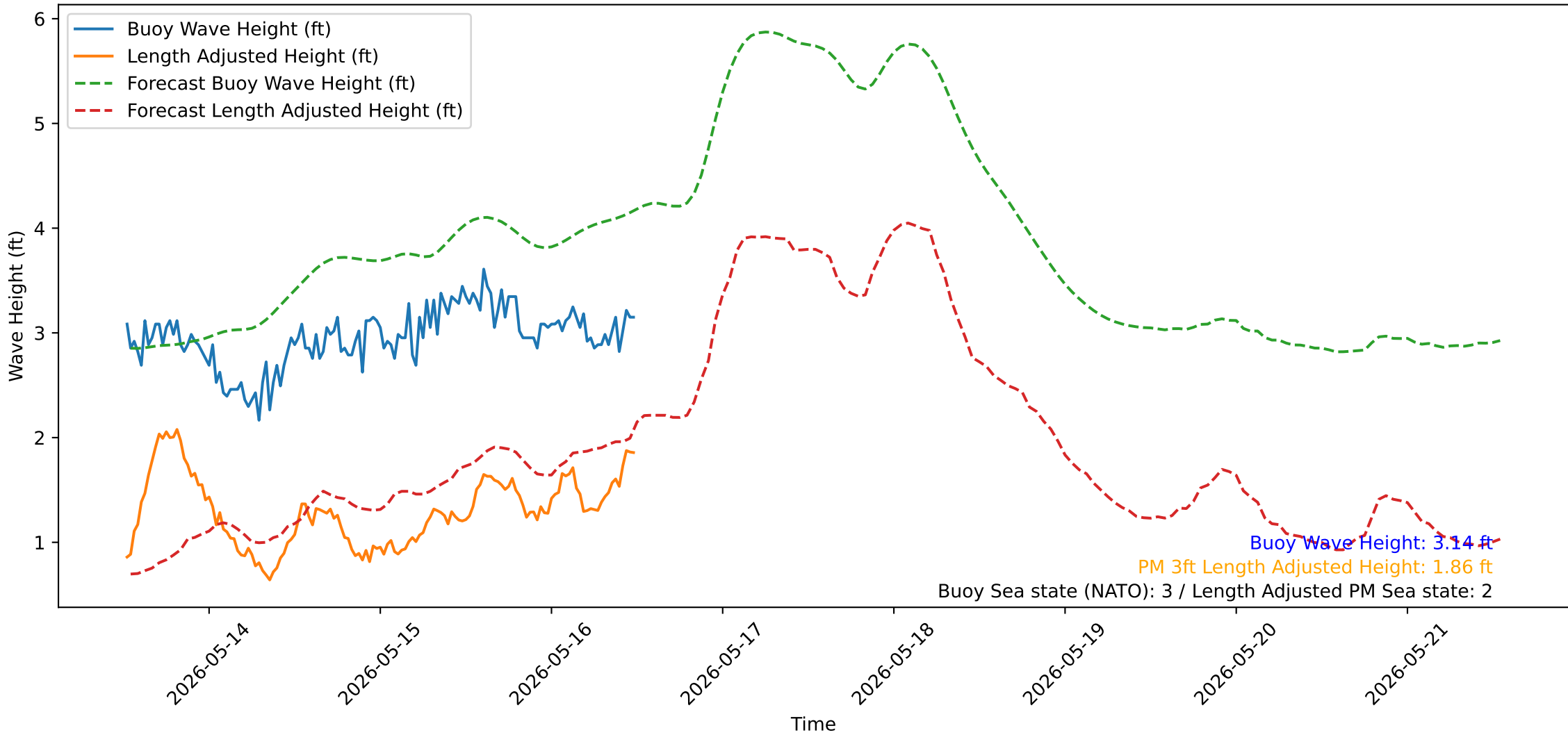
Wave Heights over Time for Oceanside Harbor at 2026-05-16 12:30:31
