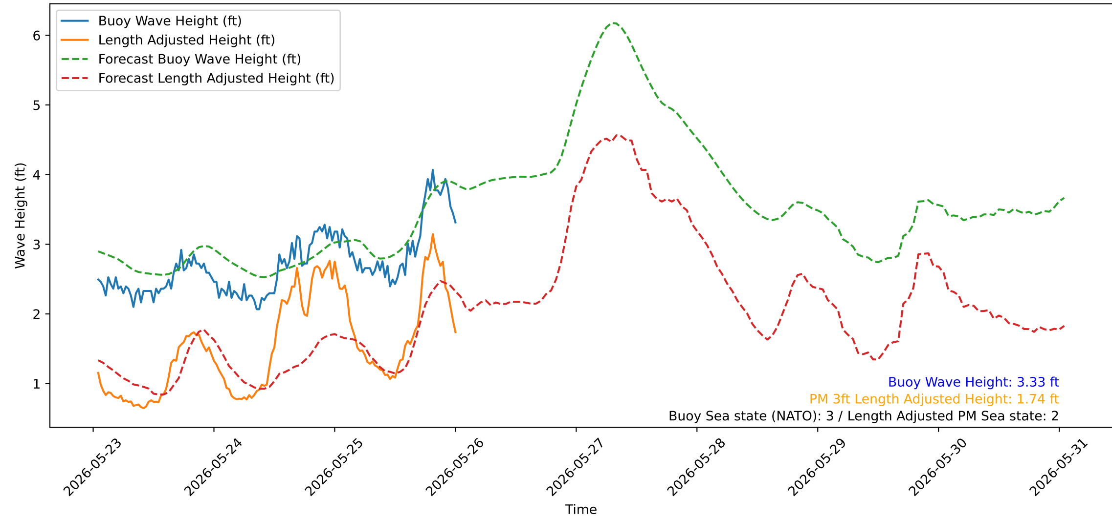
Wave Heights over Time for Green Beach at 2026-05-26 00:51:12
