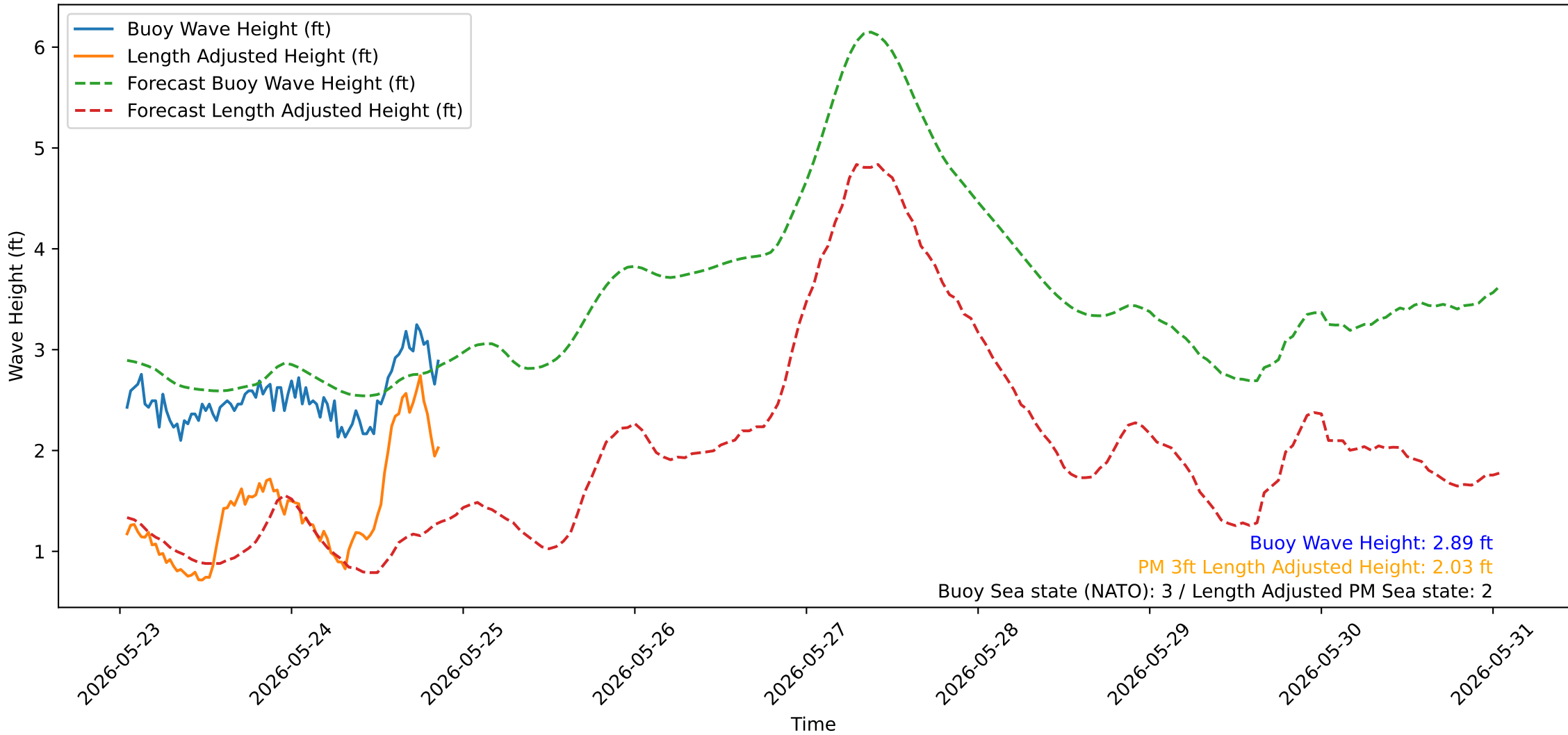
Wave Heights over Time for Oceanside Harbor at 2026-05-26 00:50:29
