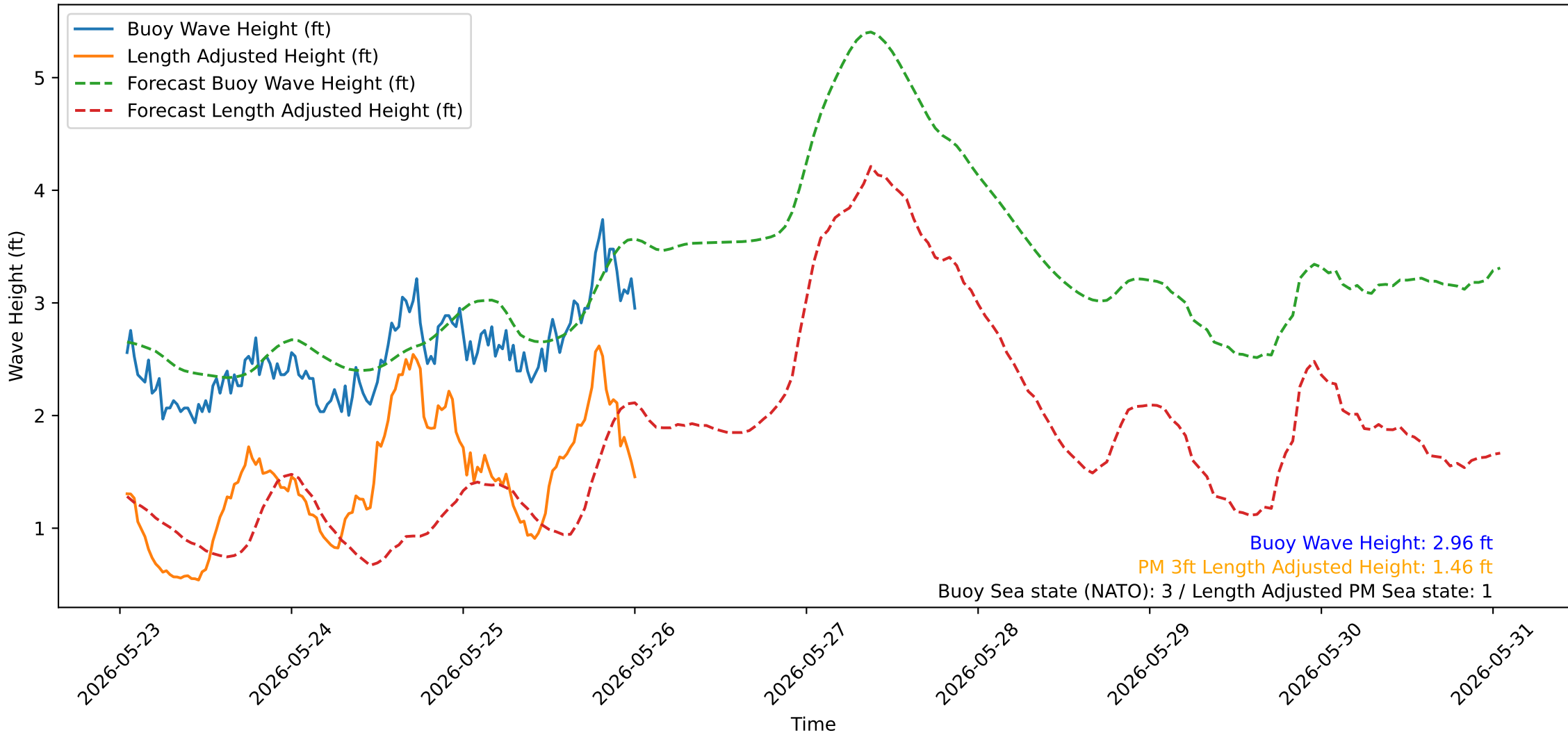
Wave Heights over Time for Red Beach at 2026-05-26 00:50:50
