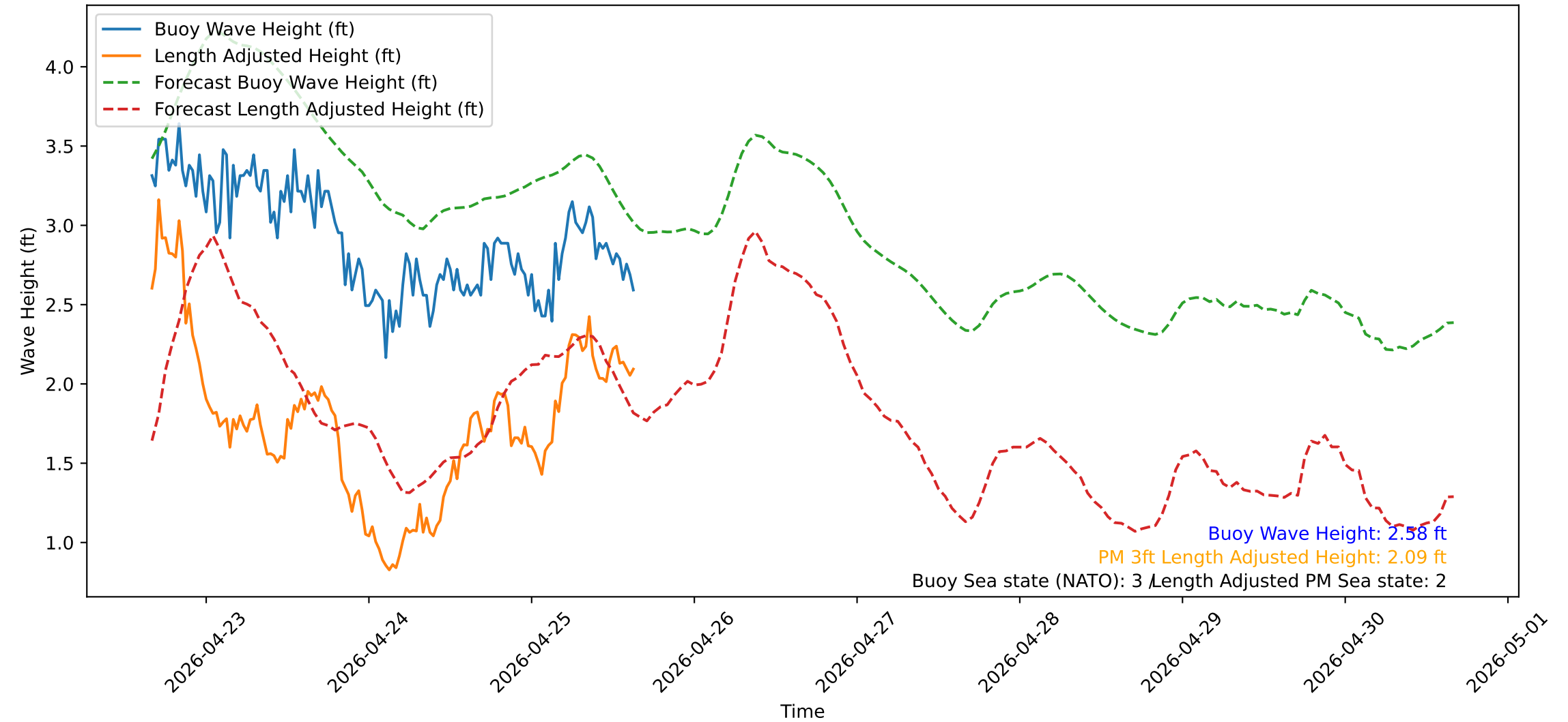
Wave Heights over Time for Red Beach at 2026-04-25 15:50:51
