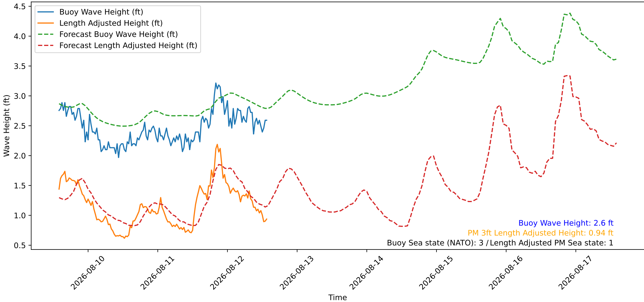
Wave Heights over Time for Green Beach at 2026-08-12 14:11:08
