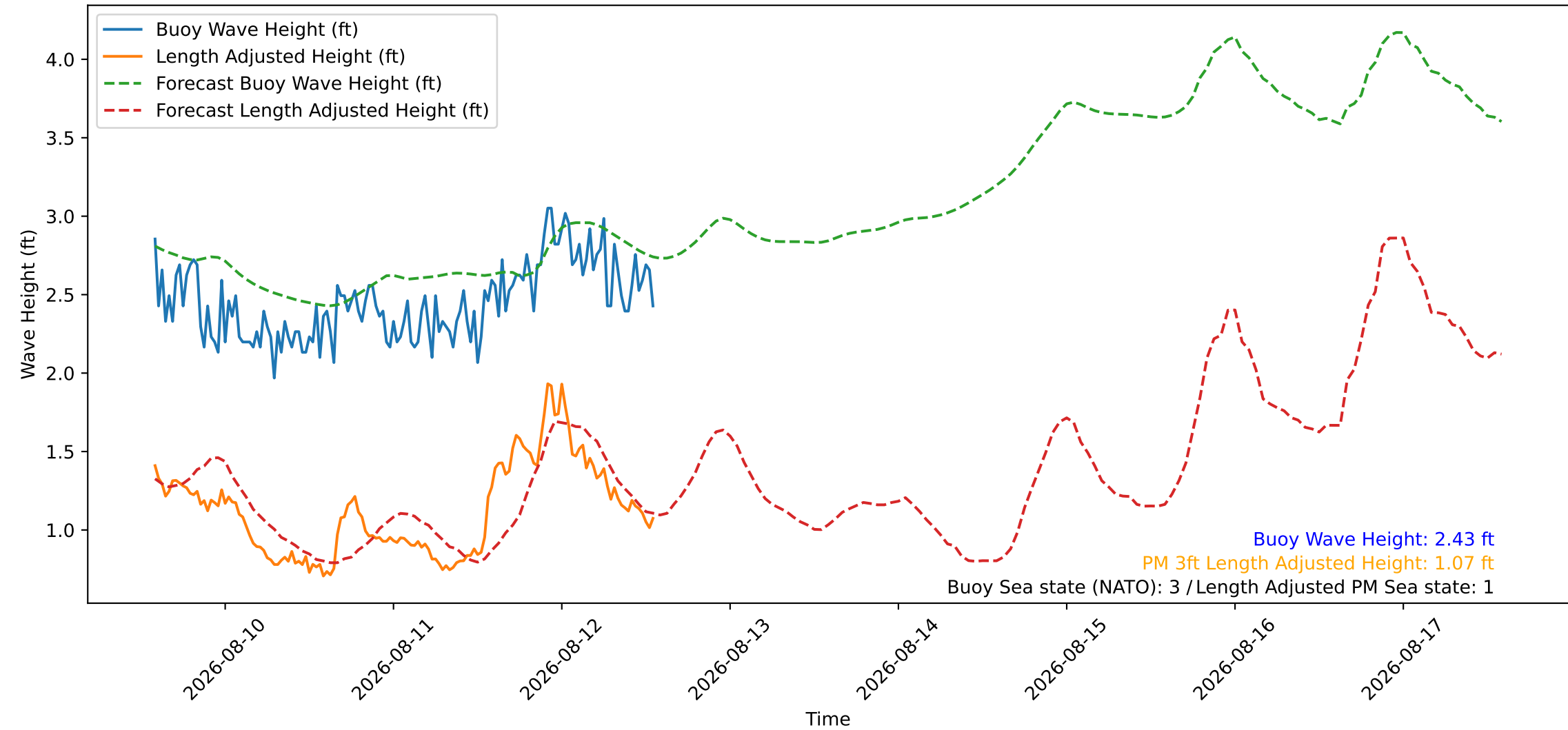
Wave Heights over Time for Oceanside Harbor at 2026-08-12 14:10:26
