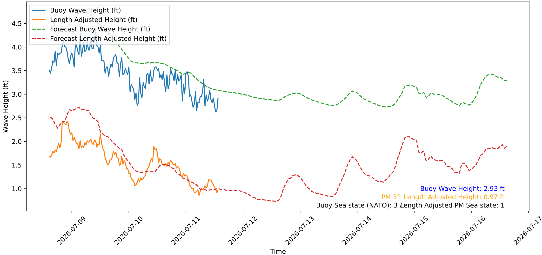
Wave Heights over Time for Green Beach at 2026-07-11 14:31:09
