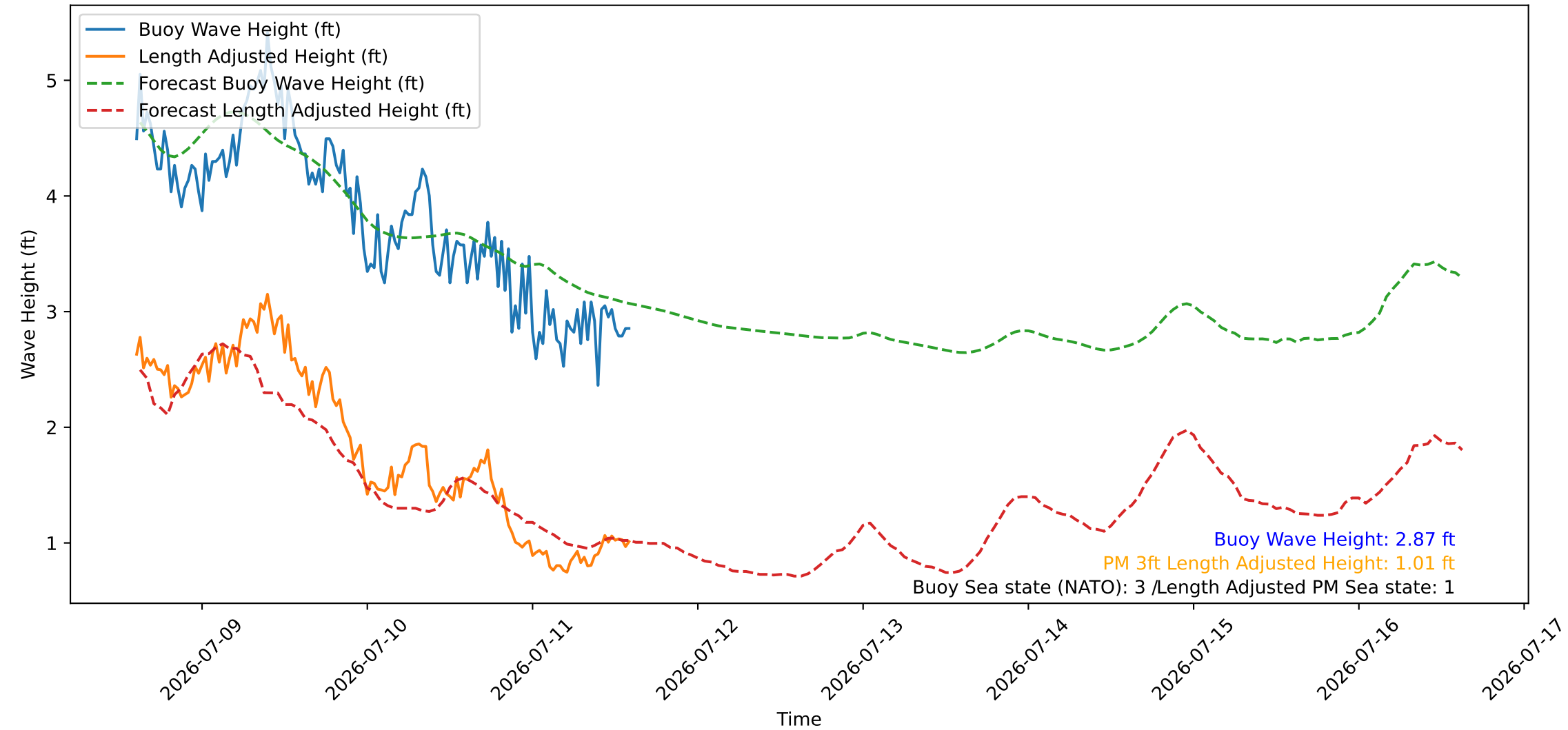
Wave Heights over Time for Oceanside Harbor at 2026-07-11 14:30:27
