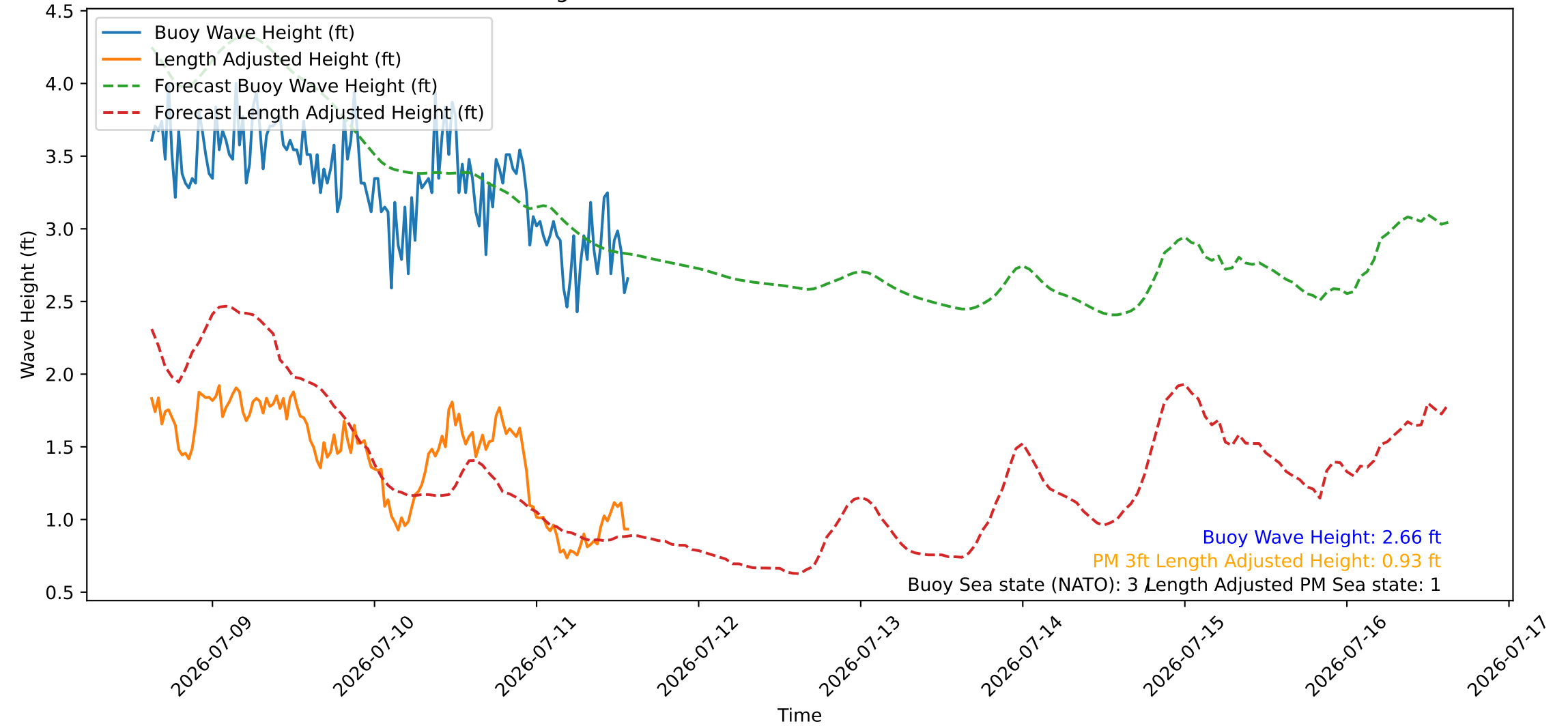
Wave Heights over Time for Red Beach at 2026-07-11 14:30:47
