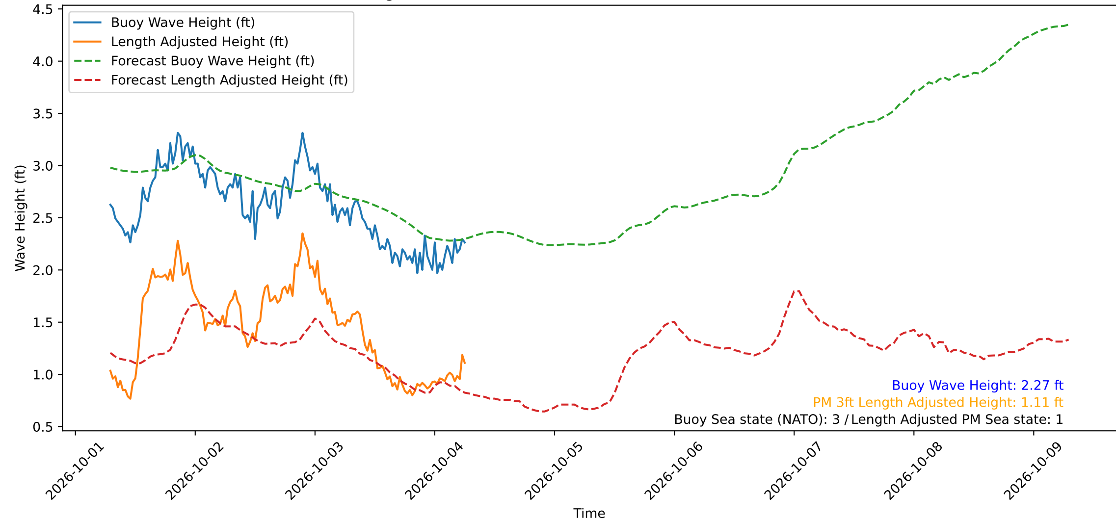
Wave Heights over Time for Oceanside Harbor at 2026-10-04 06:50:30
