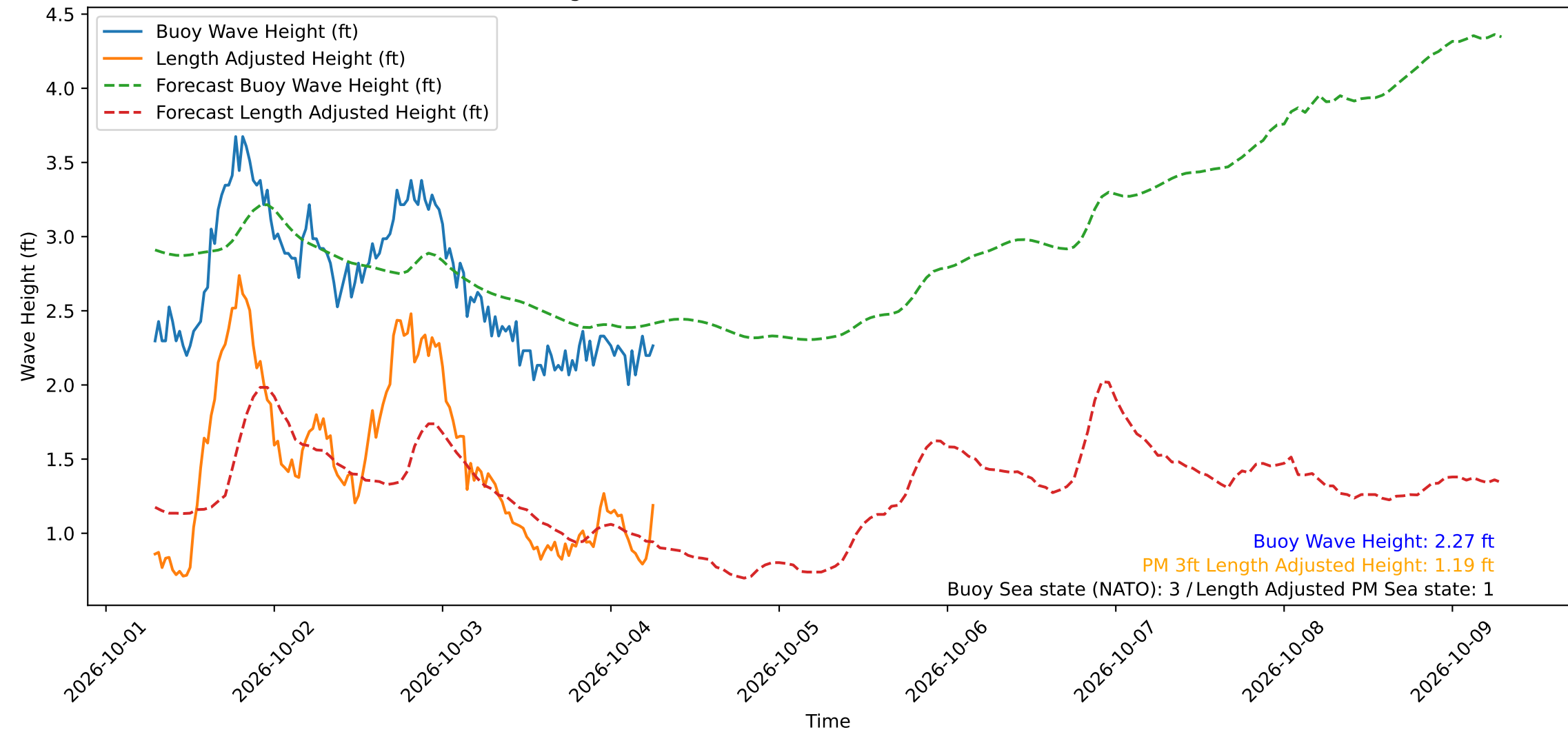
Wave Heights over Time for Green Beach at 2026-10-04 06:51:14
