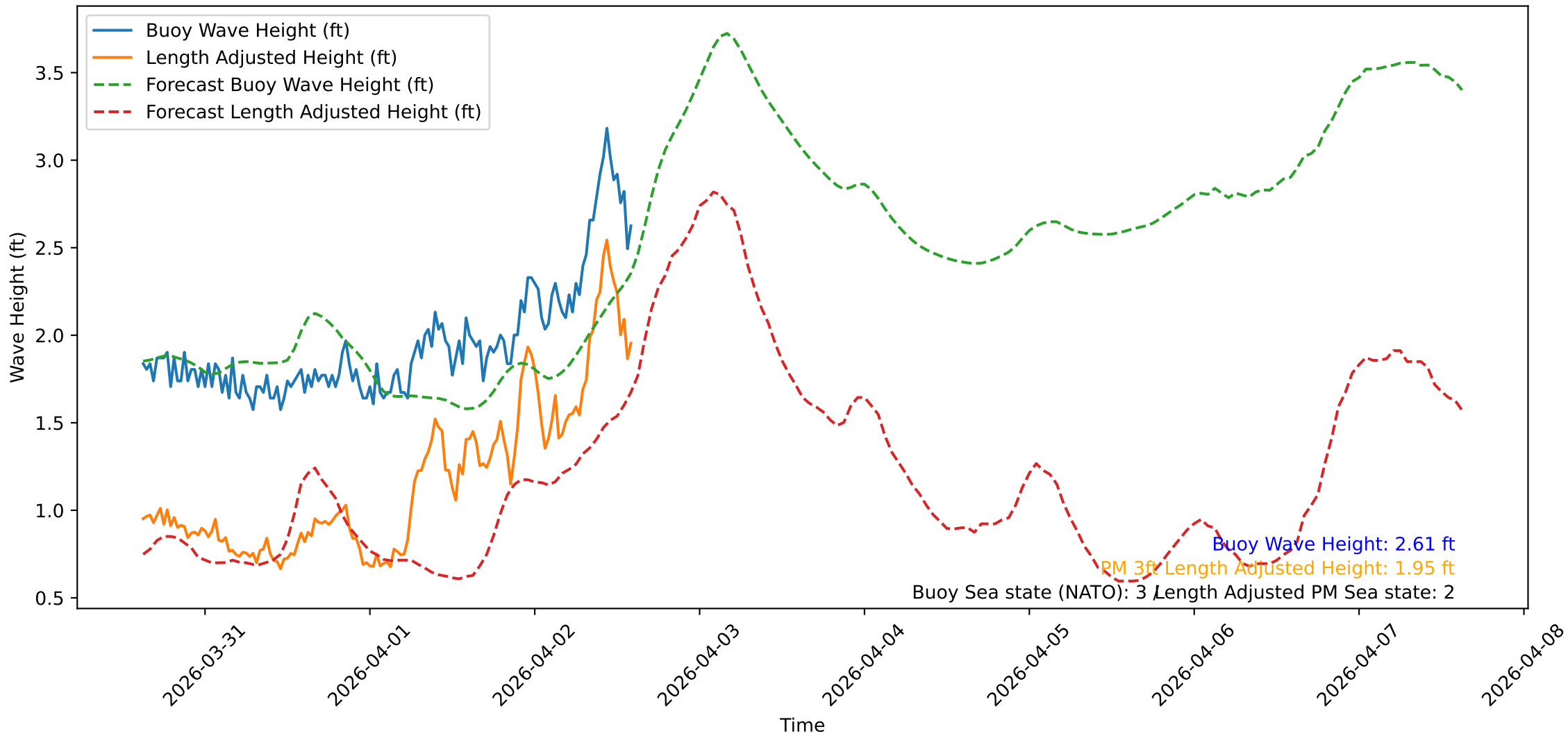
Wave Heights over Time for Oceanside Harbor at 2026-04-02 15:00:31
