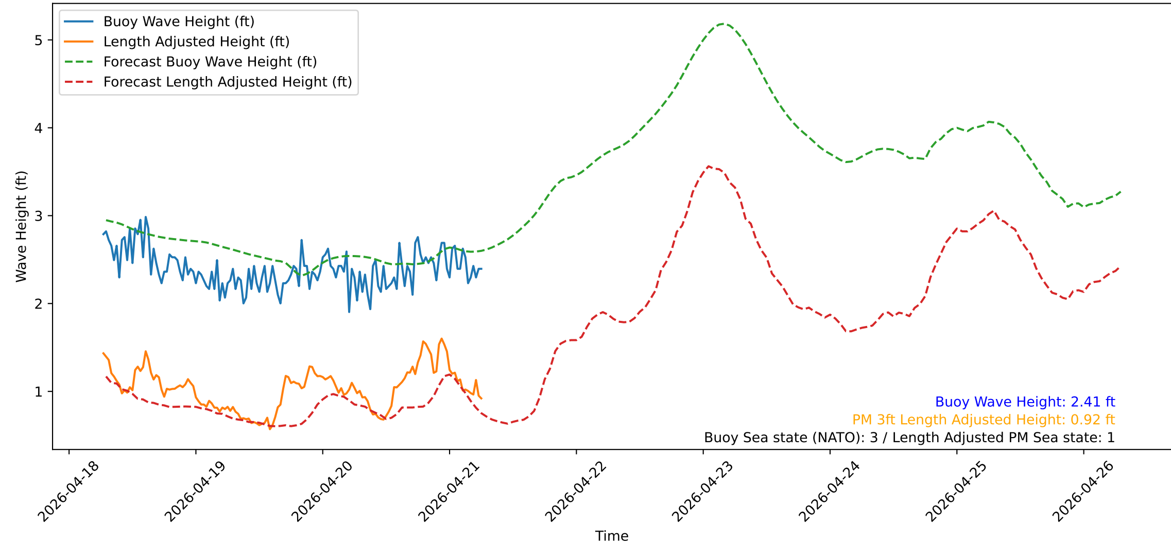
Wave Heights over Time for Oceanside Harbor at 2026-04-21 06:30:32
