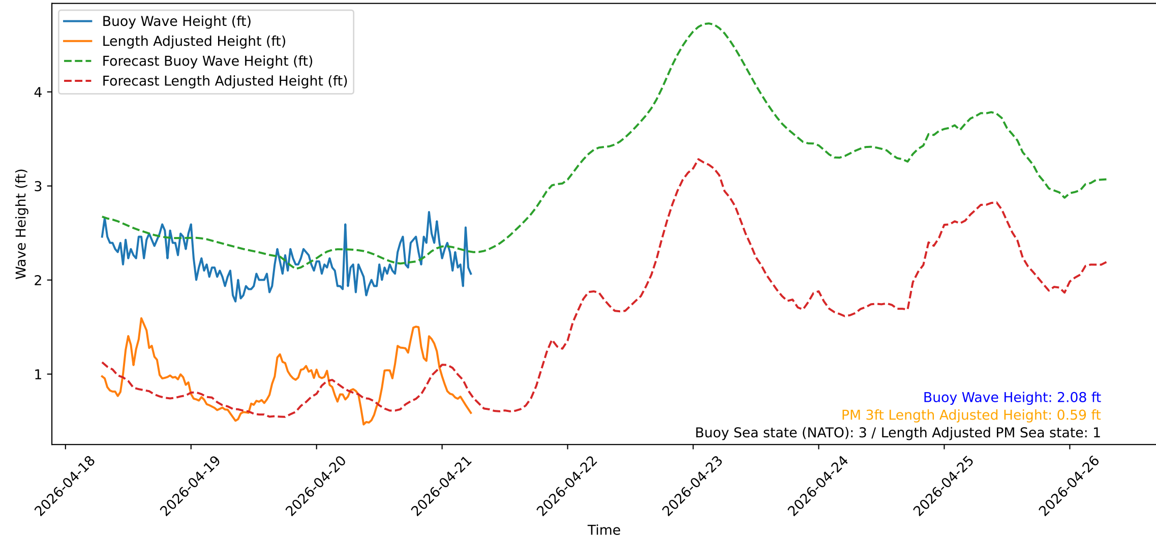
Wave Heights over Time for Red Beach at 2026-04-21 06:30:52
