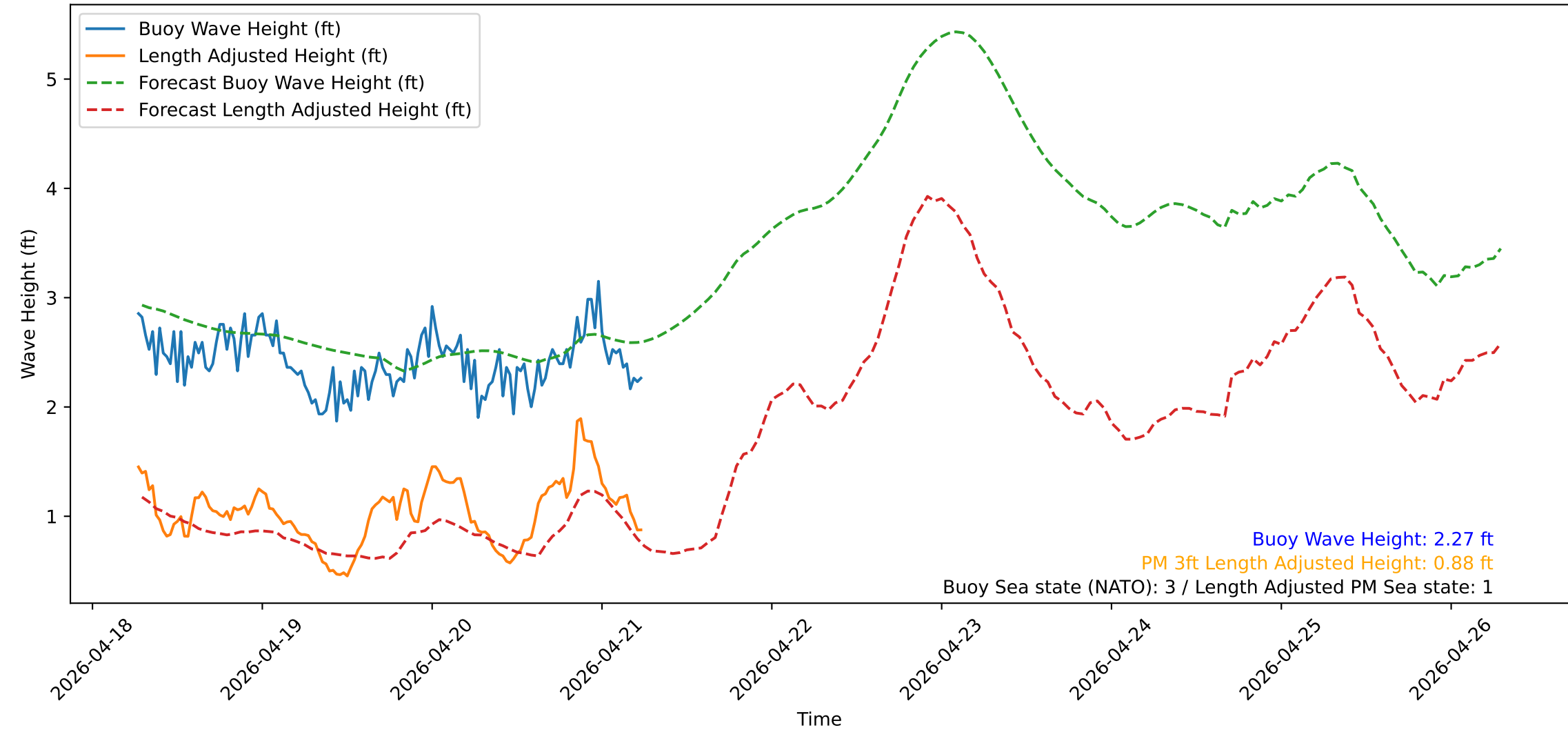
Wave Heights over Time for Green Beach at 2026-04-21 06:31:14
