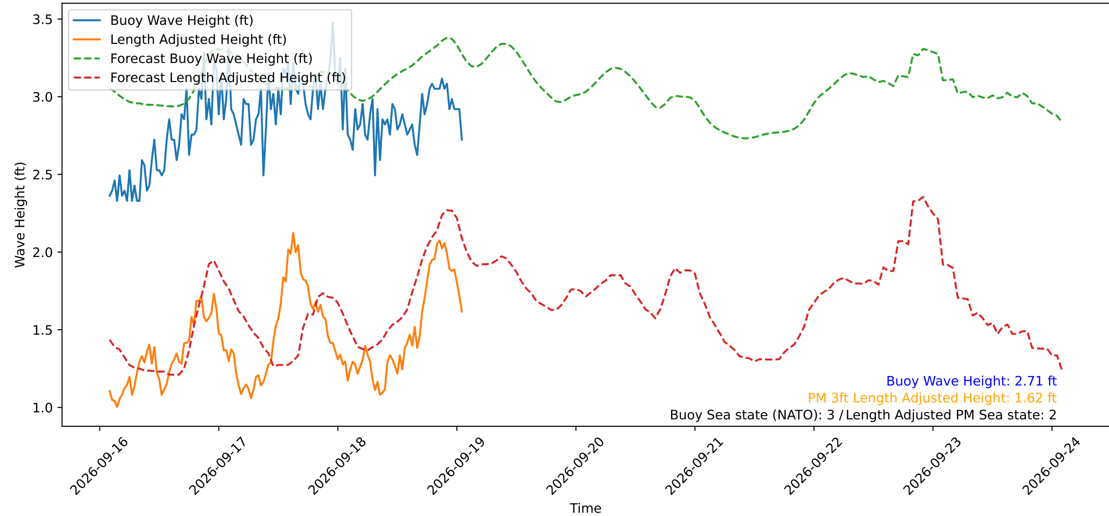
Wave Heights over Time for Green Beach at 2026-09-19 01:51:13
