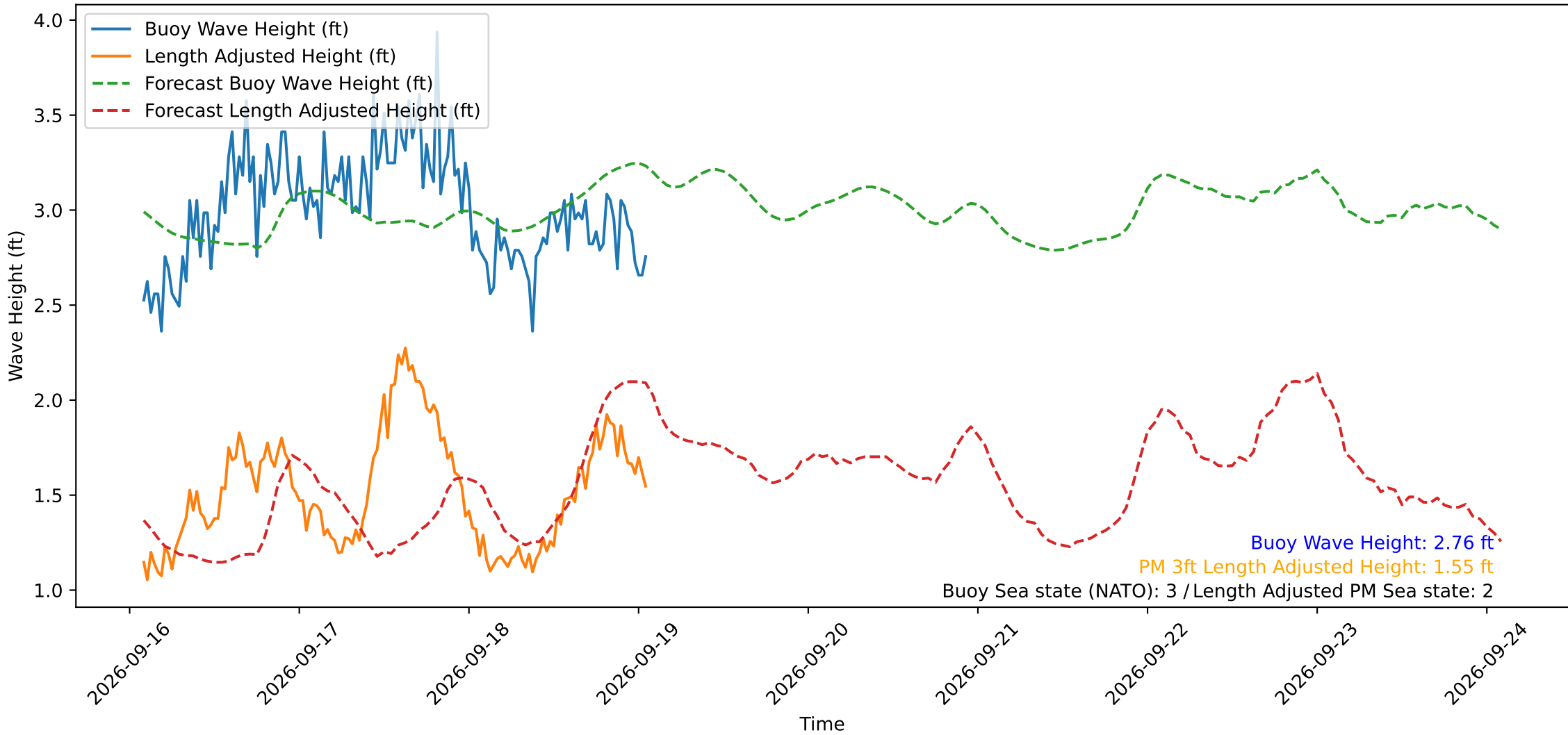
Wave Heights over Time for Oceanside Harbor at 2026-09-19 01:50:29
