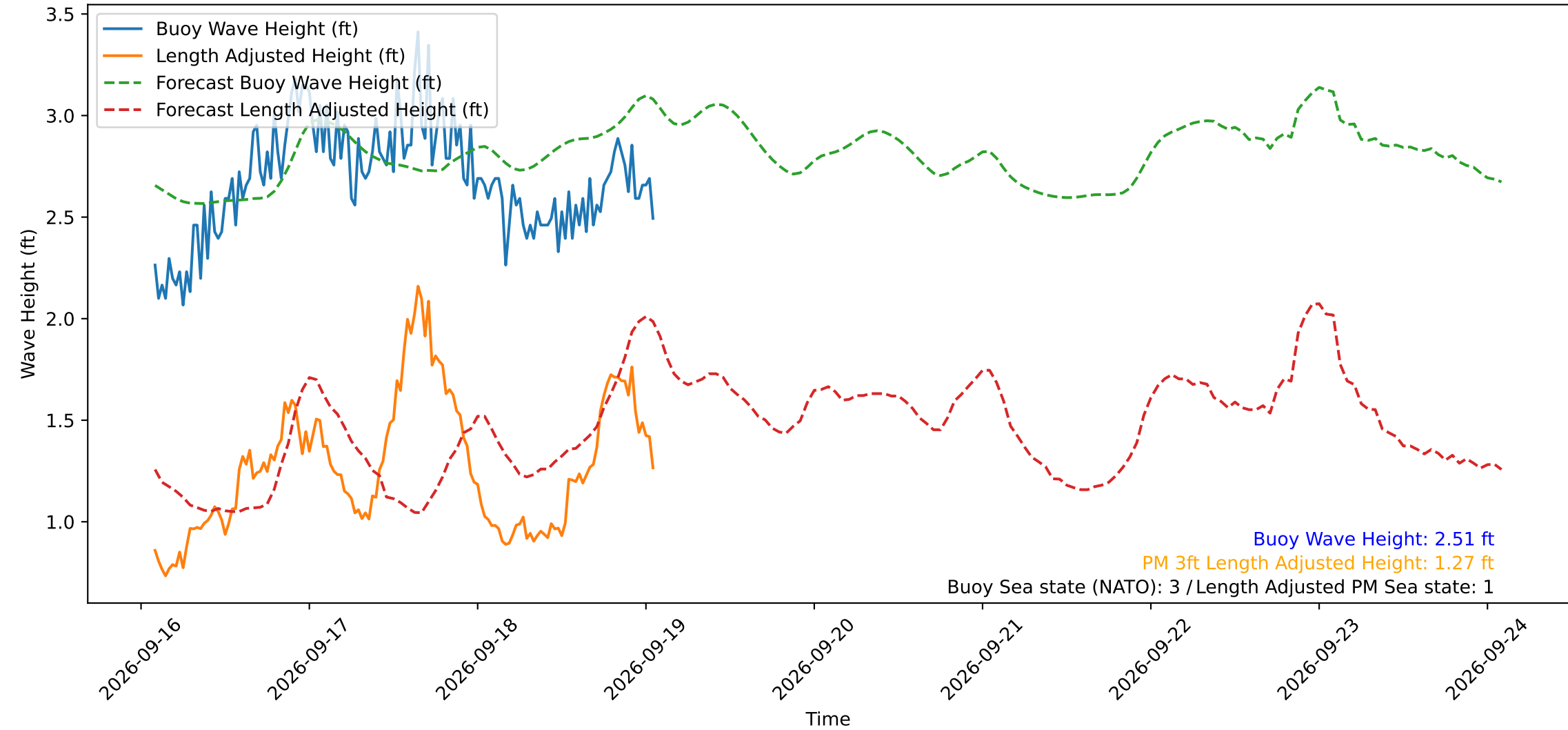
Wave Heights over Time for Red Beach at 2026-09-19 01:50:50
