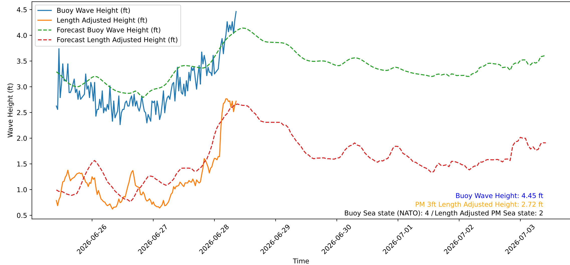
Wave Heights over Time for Red Beach at 2026-06-28 09:30:45
