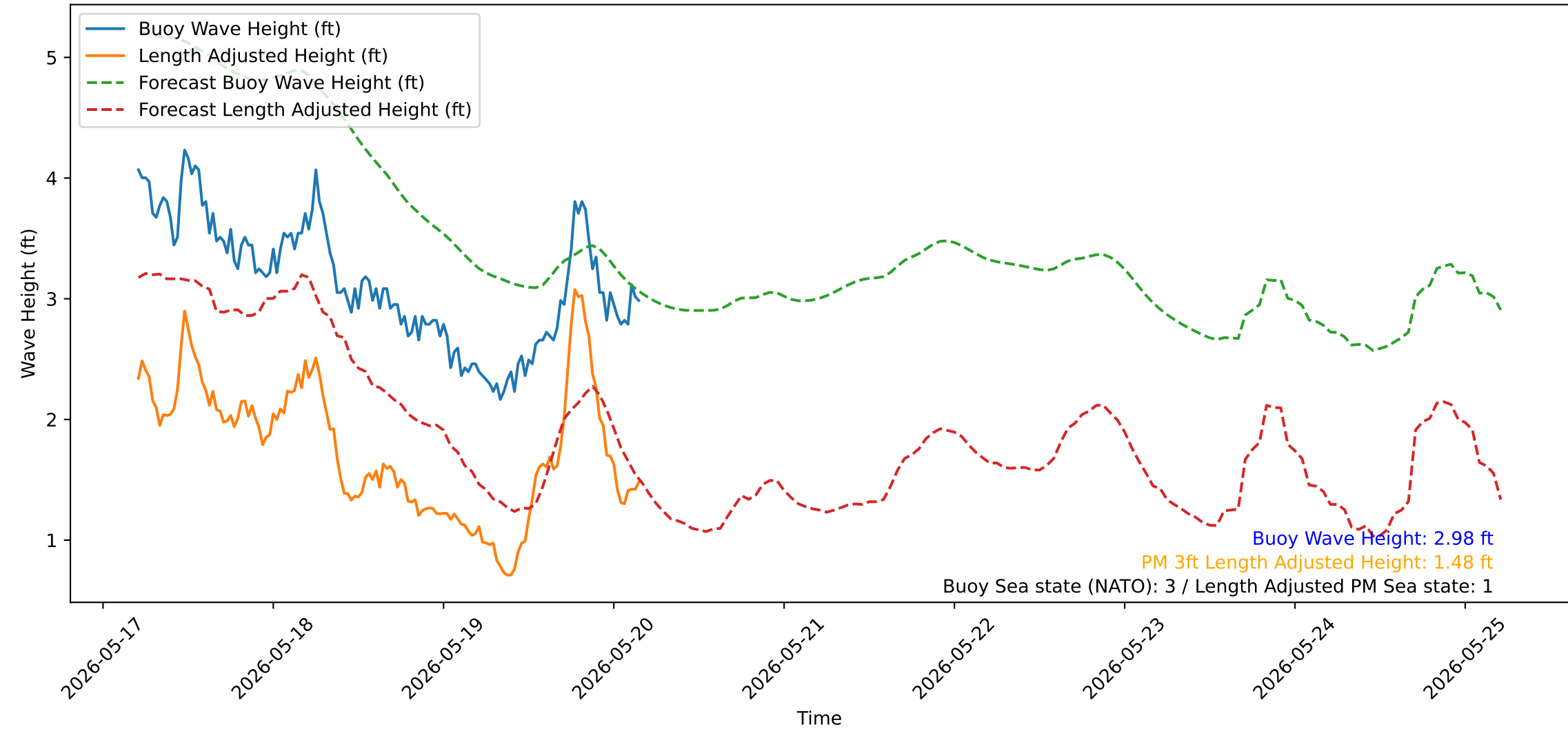
Wave Heights over Time for Green Beach at 2026-05-20 04:51:14
