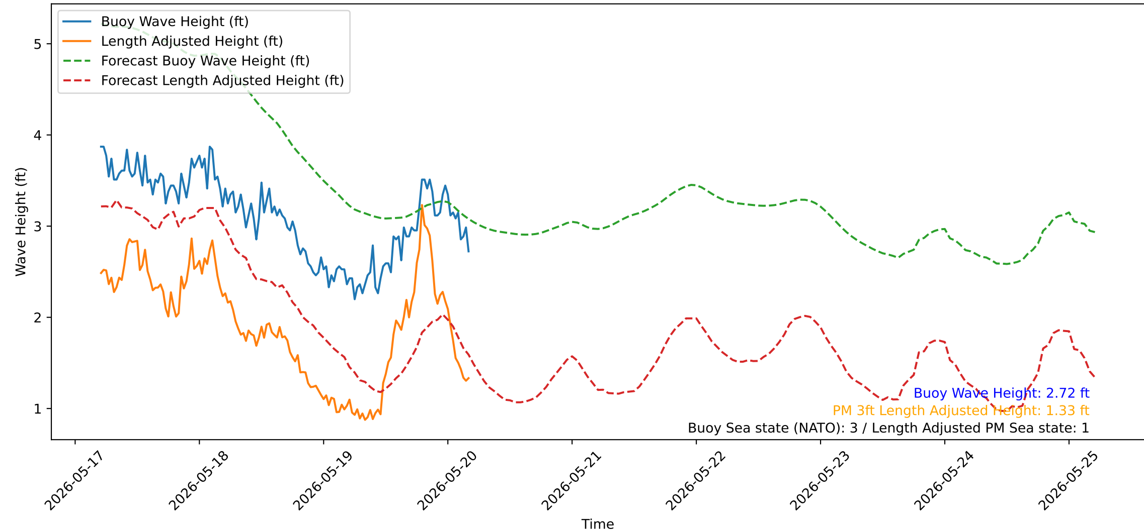
Wave Heights over Time for Oceanside Harbor at 2026-05-20 04:50:31
