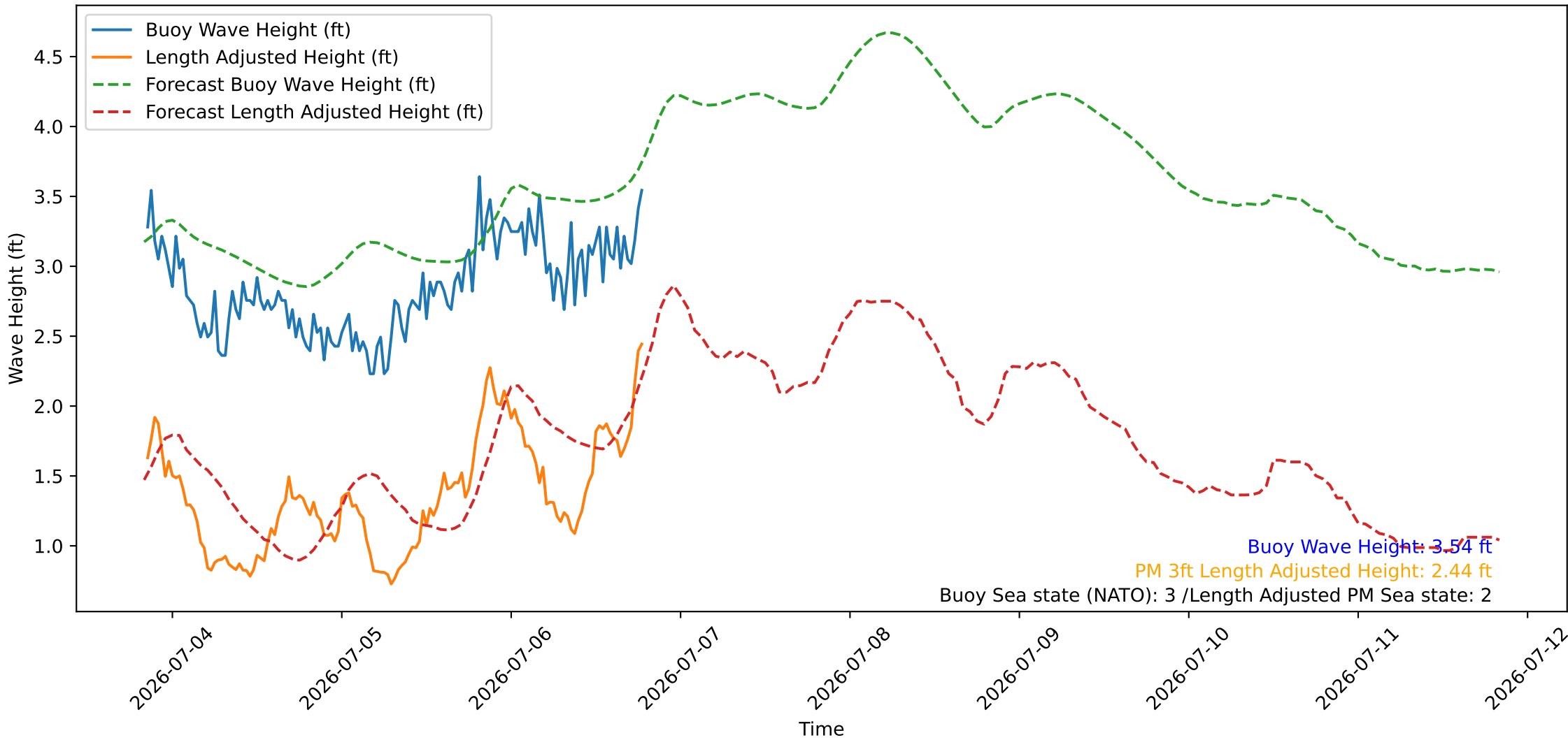
Wave Heights over Time for Red Beach at 2026-07-06 20:00:46
