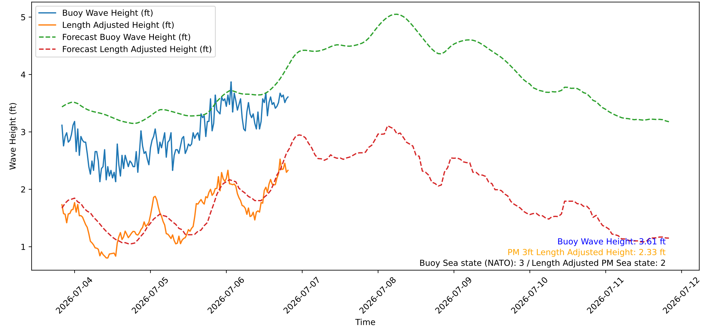
Wave Heights over Time for Oceanside Harbor at 2026-07-06 20:00:27
