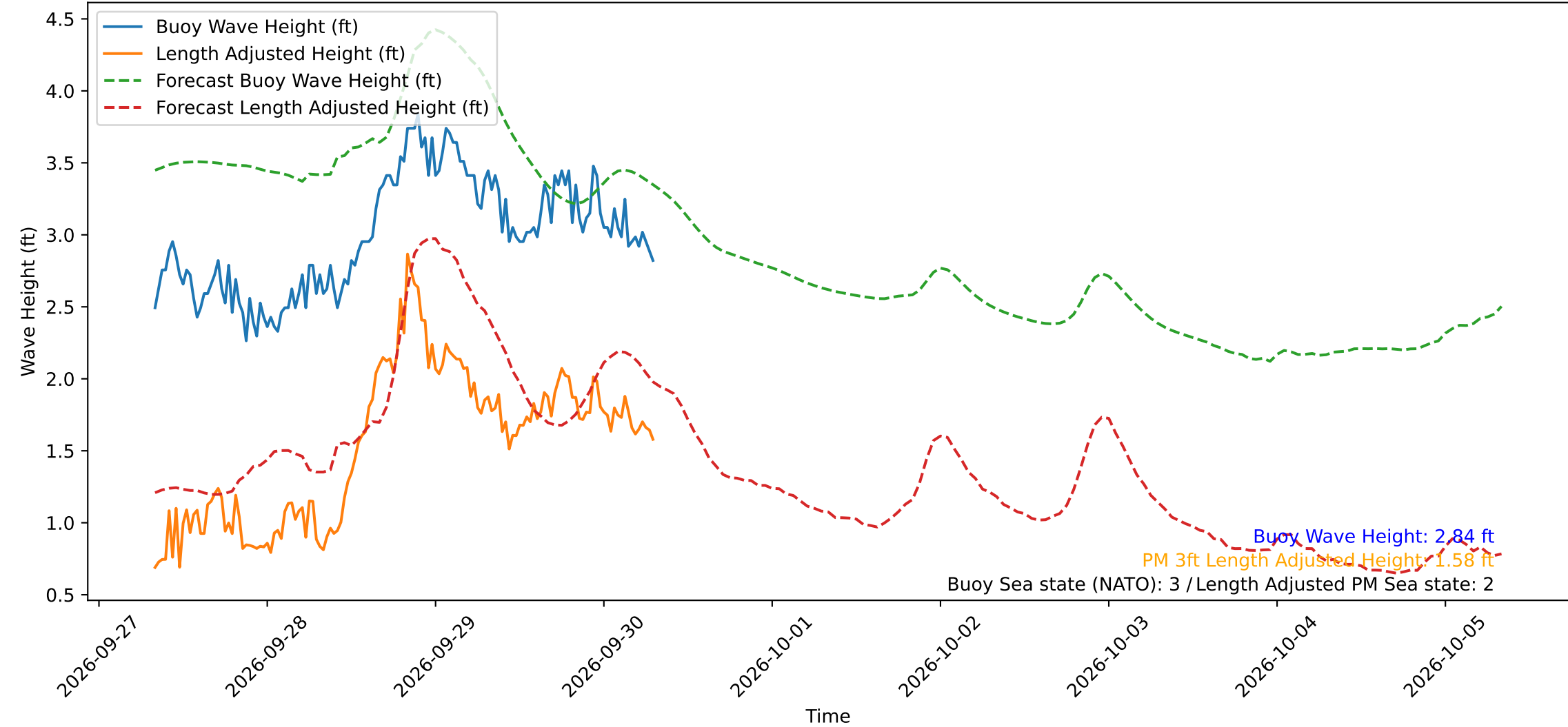
Wave Heights over Time for Red Beach at 2026-09-30 07:40:49
