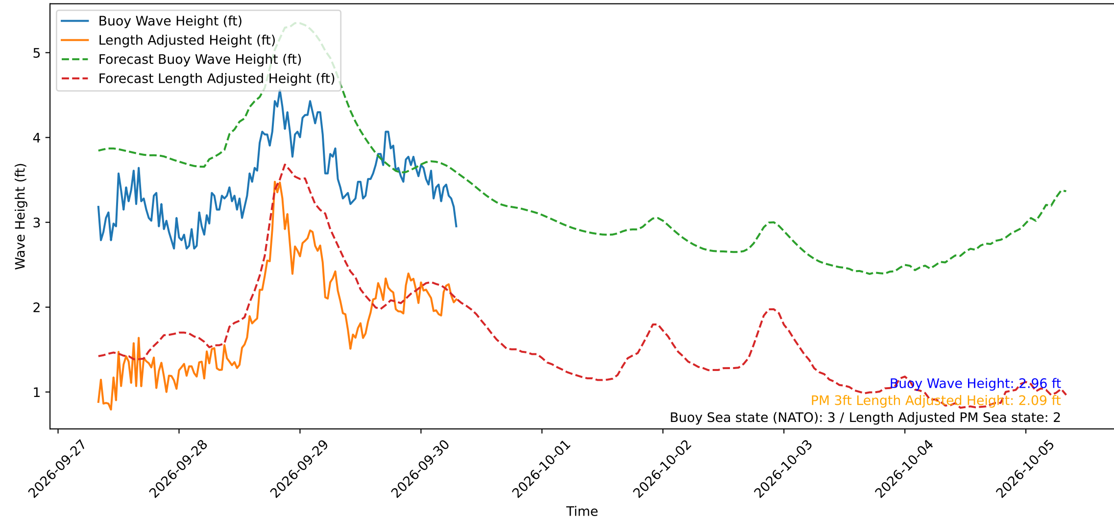
Wave Heights over Time for Green Beach at 2026-09-30 07:41:12
