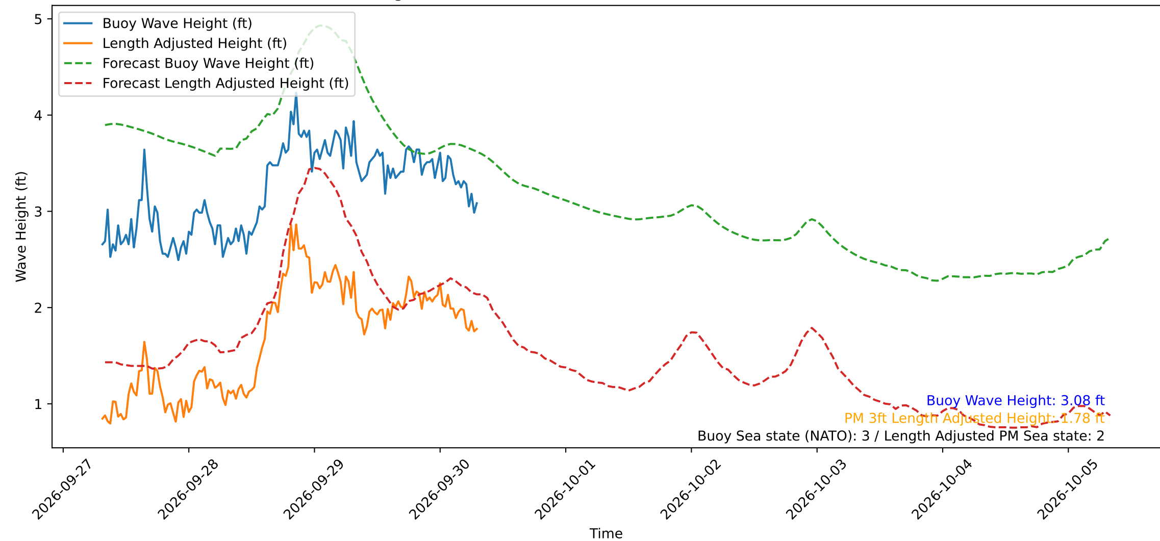
Wave Heights over Time for Oceanside Harbor at 2026-09-30 07:40:29
