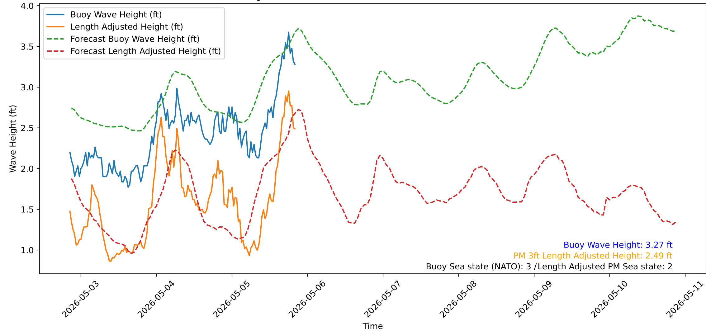
Wave Heights over Time for Green Beach at 2026-05-05 20:41:14
