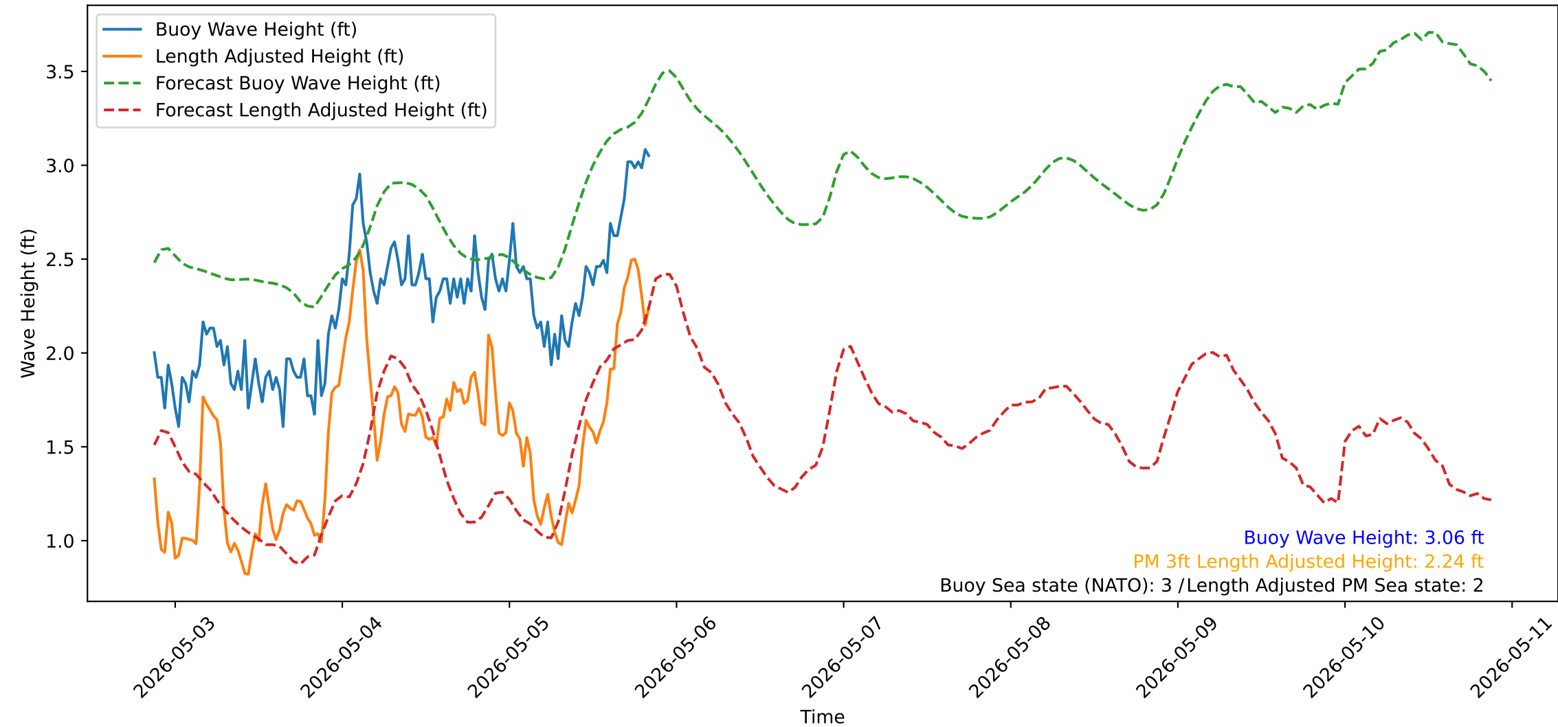
Wave Heights over Time for Red Beach at 2026-05-05 20:40:51
