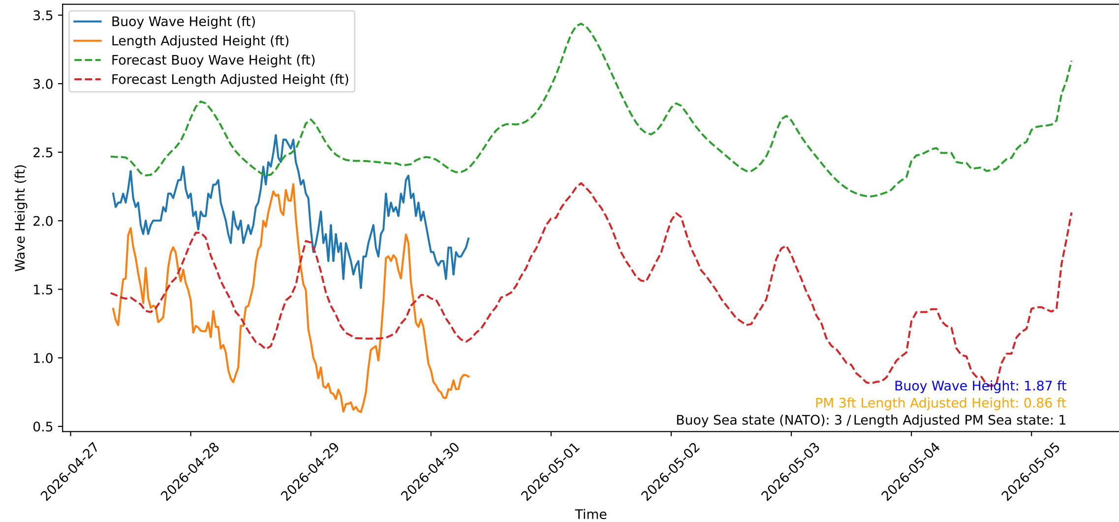
Wave Heights over Time for Red Beach at 2026-04-30 08:10:51
