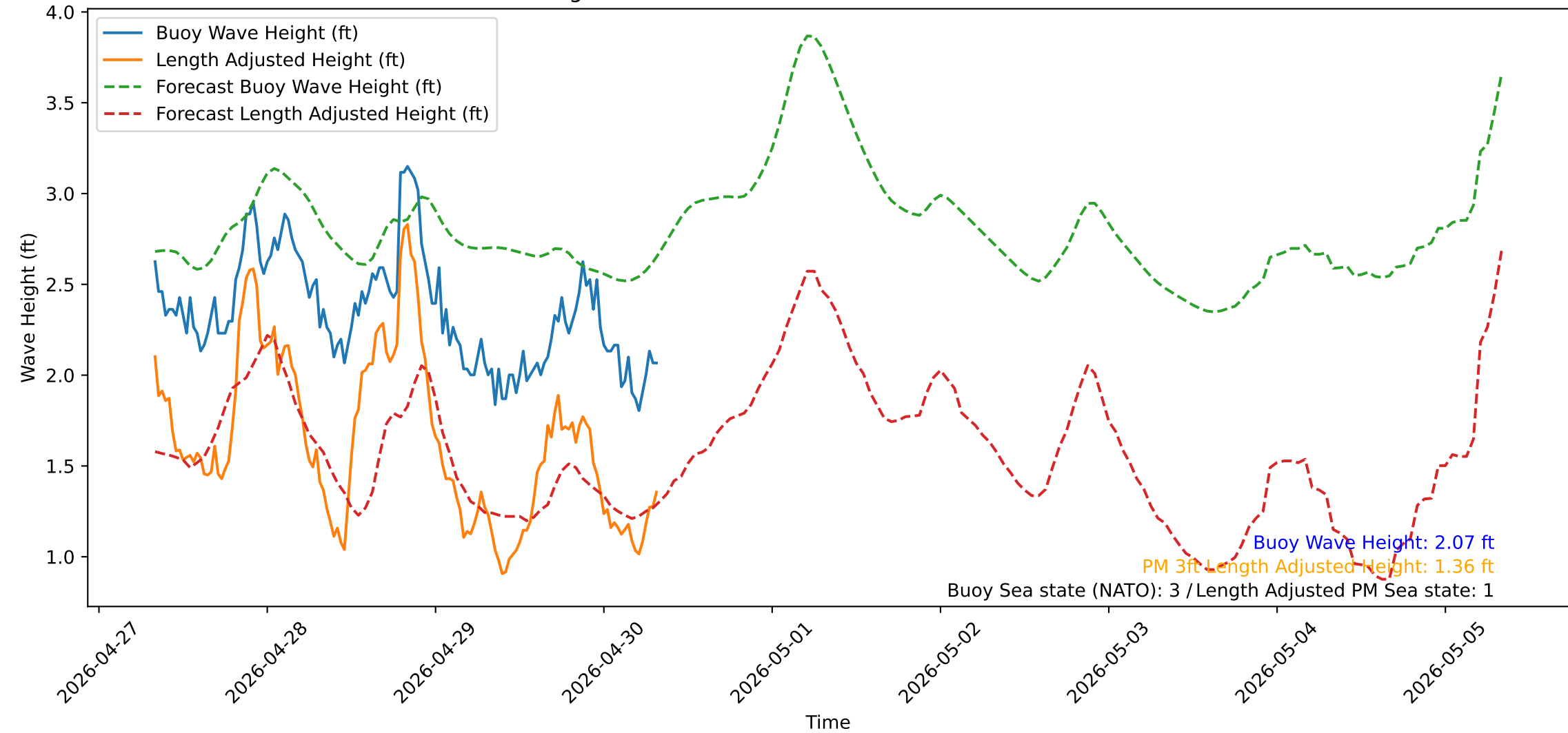
Wave Heights over Time for Green Beach at 2026-04-30 08:11:13
