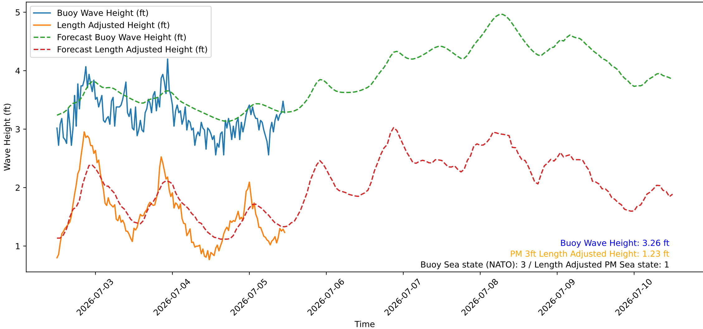
Wave Heights over Time for Green Beach at 2026-07-05 12:01:10
