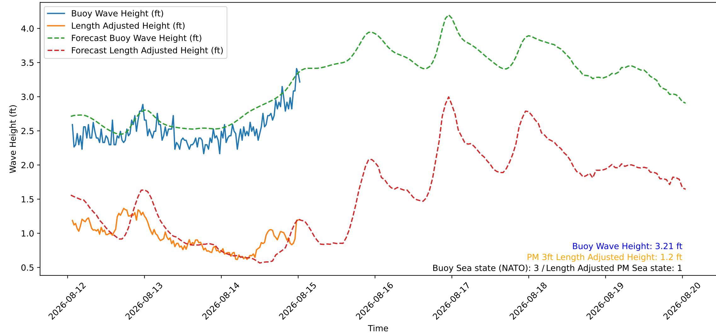
Wave Heights over Time for Red Beach at 2026-08-15 01:20:47
