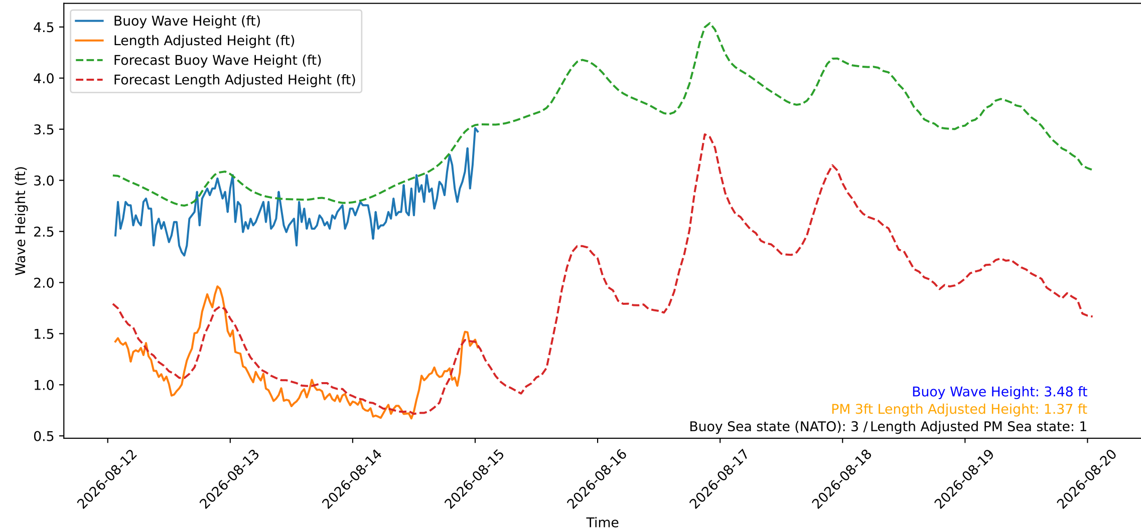
Wave Heights over Time for Green Beach at 2026-08-15 01:21:10
