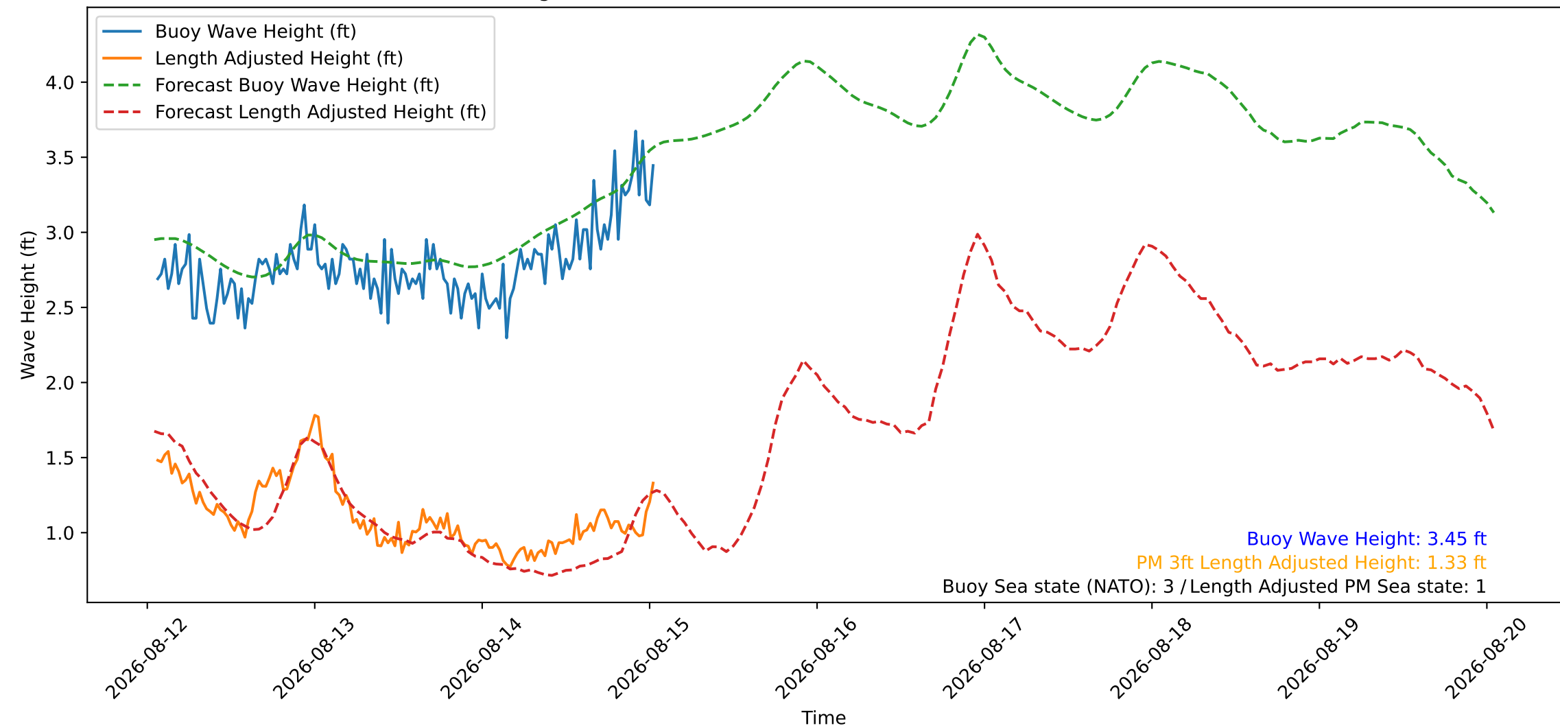
Wave Heights over Time for Oceanside Harbor at 2026-08-15 01:20:27
