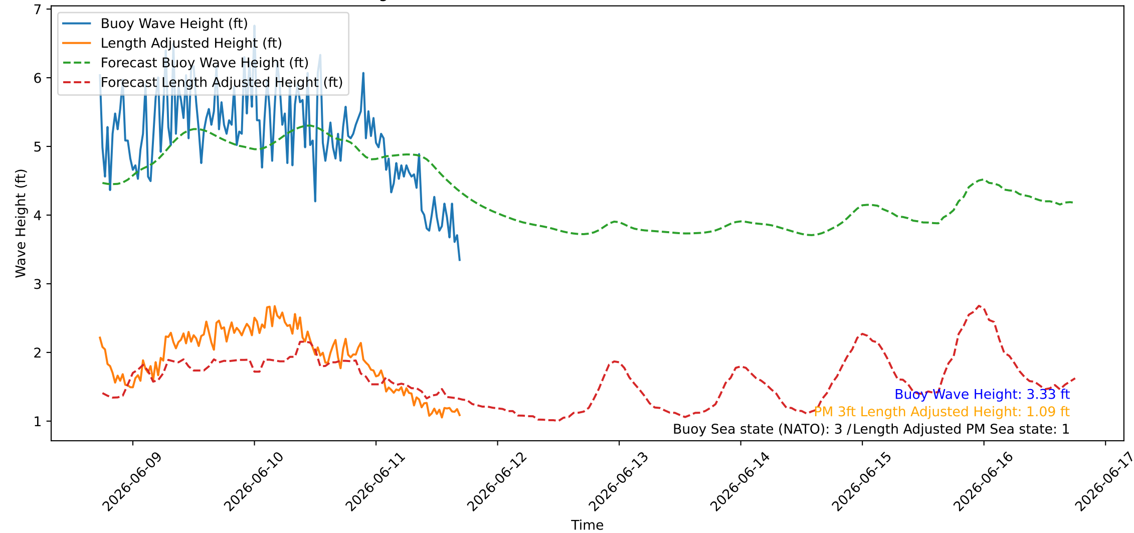
Wave Heights over Time for Oceanside Harbor at 2026-06-11 17:40:26
