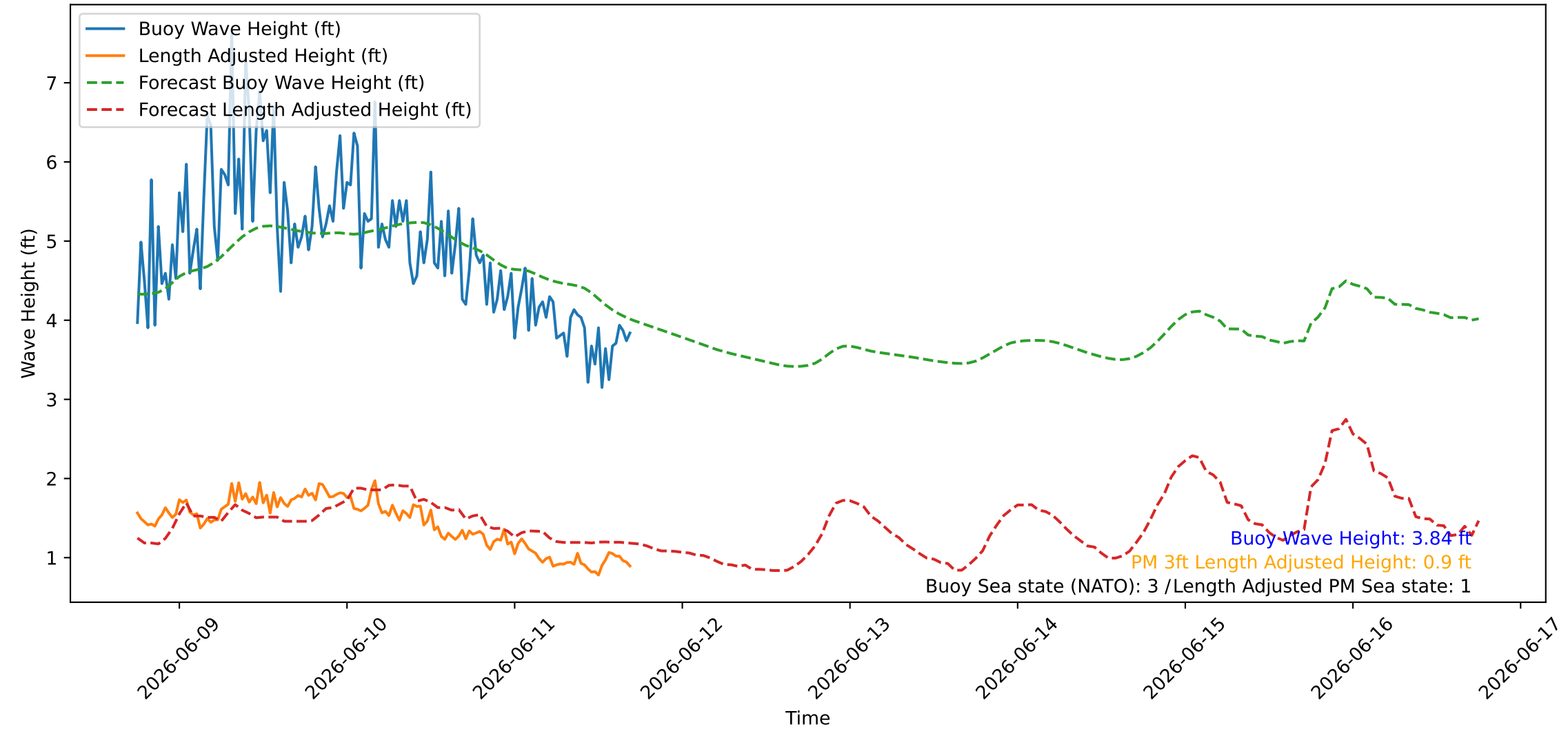
Wave Heights over Time for Red Beach at 2026-06-11 17:40:46
