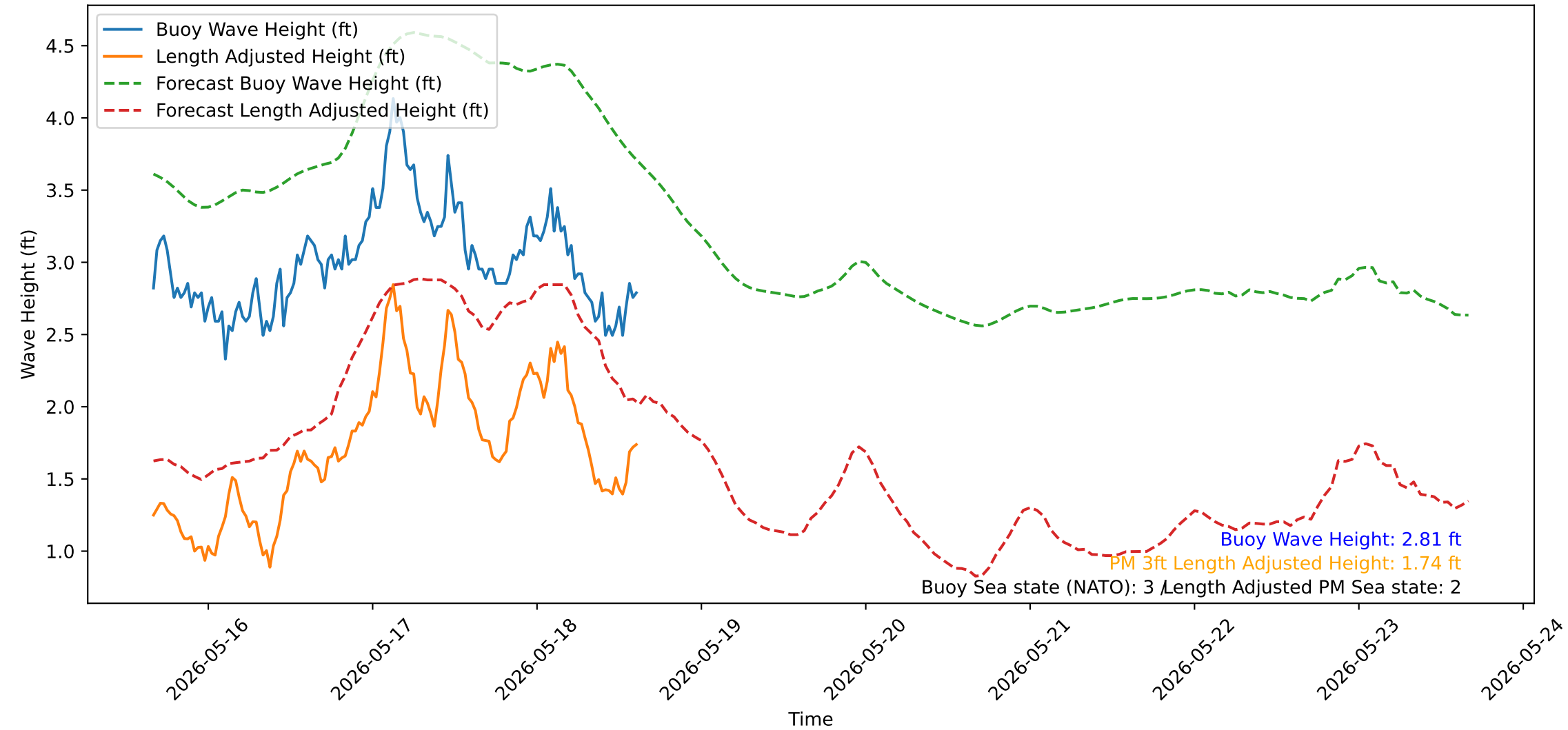
Wave Heights over Time for Red Beach at 2026-05-18 15:40:51
