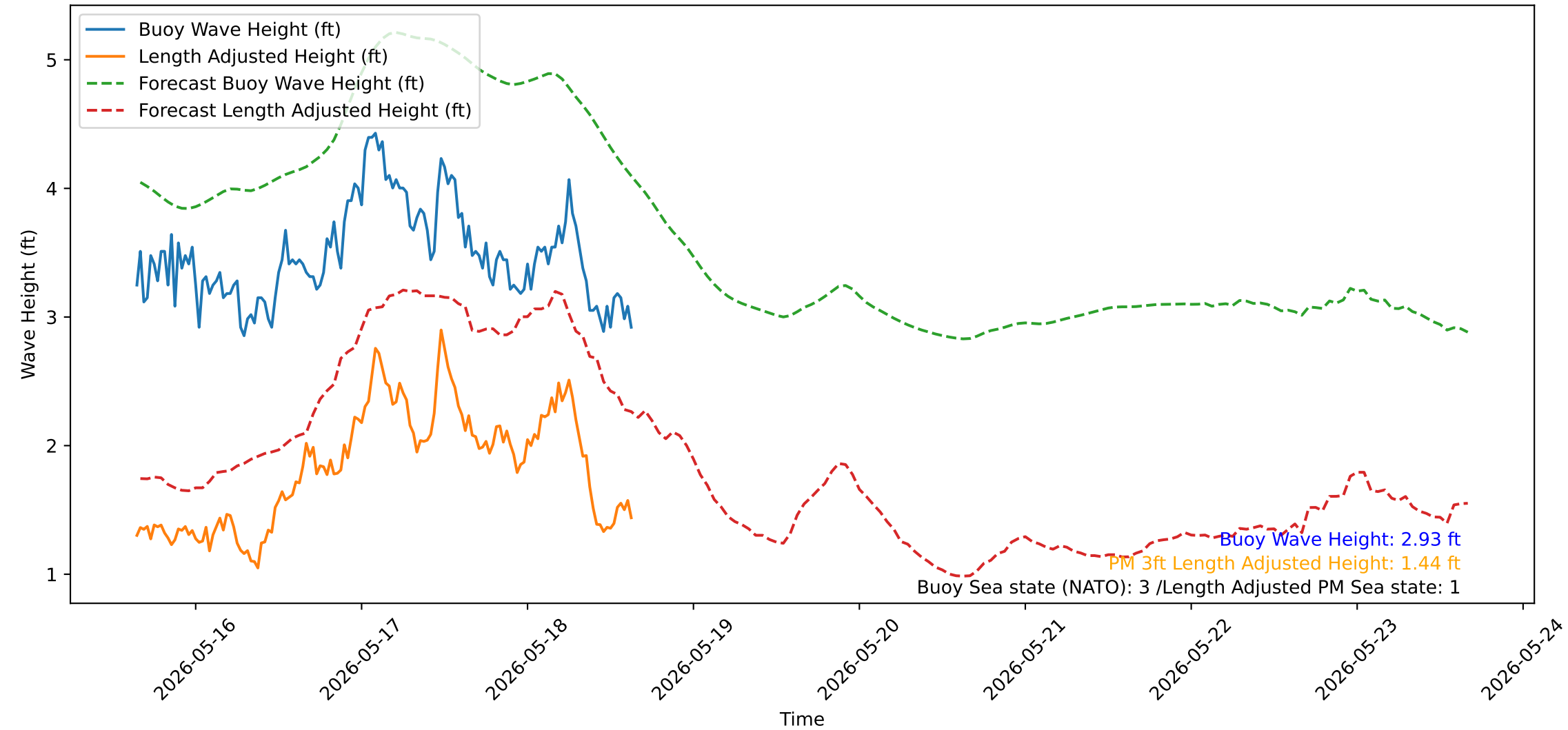
Wave Heights over Time for Green Beach at 2026-05-18 15:41:14
