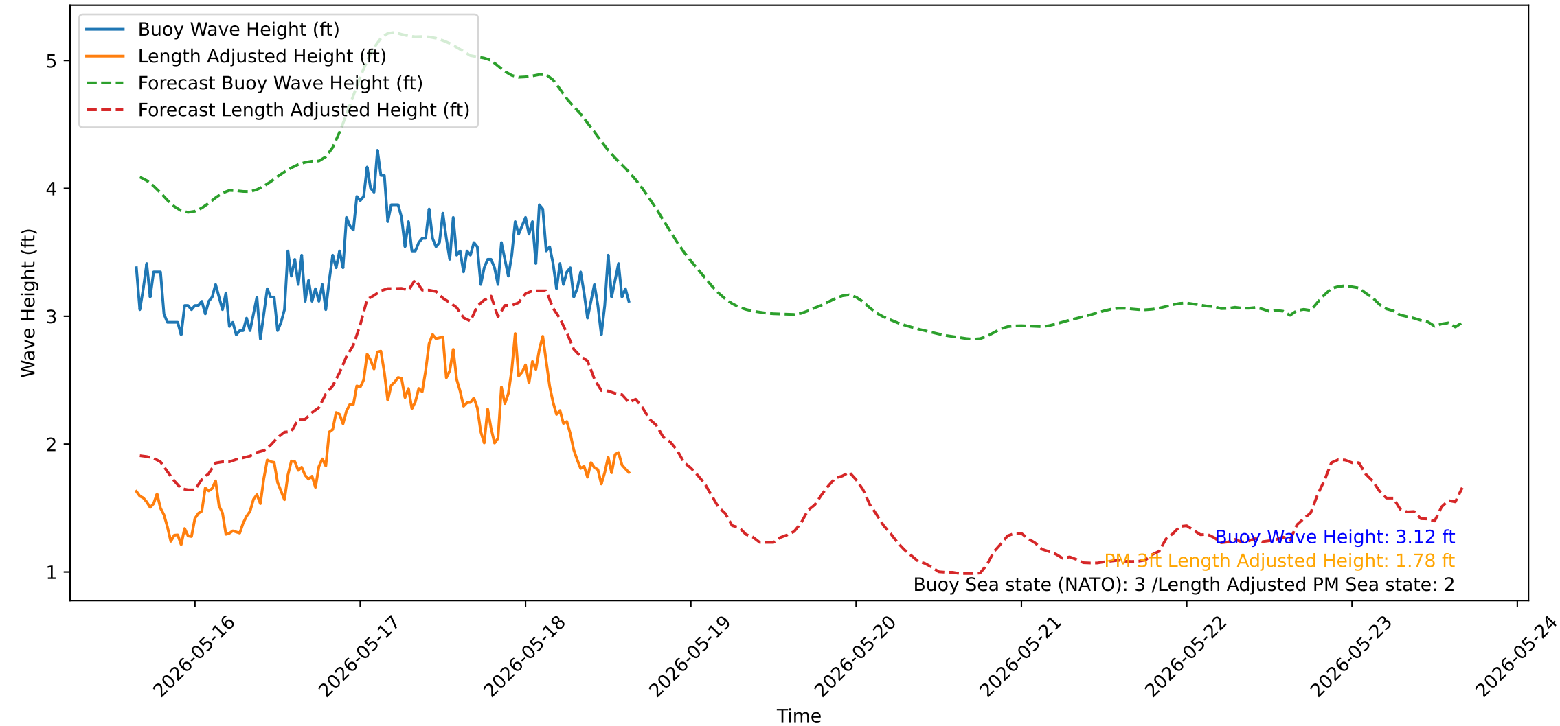
Wave Heights over Time for Oceanside Harbor at 2026-05-18 15:40:32
