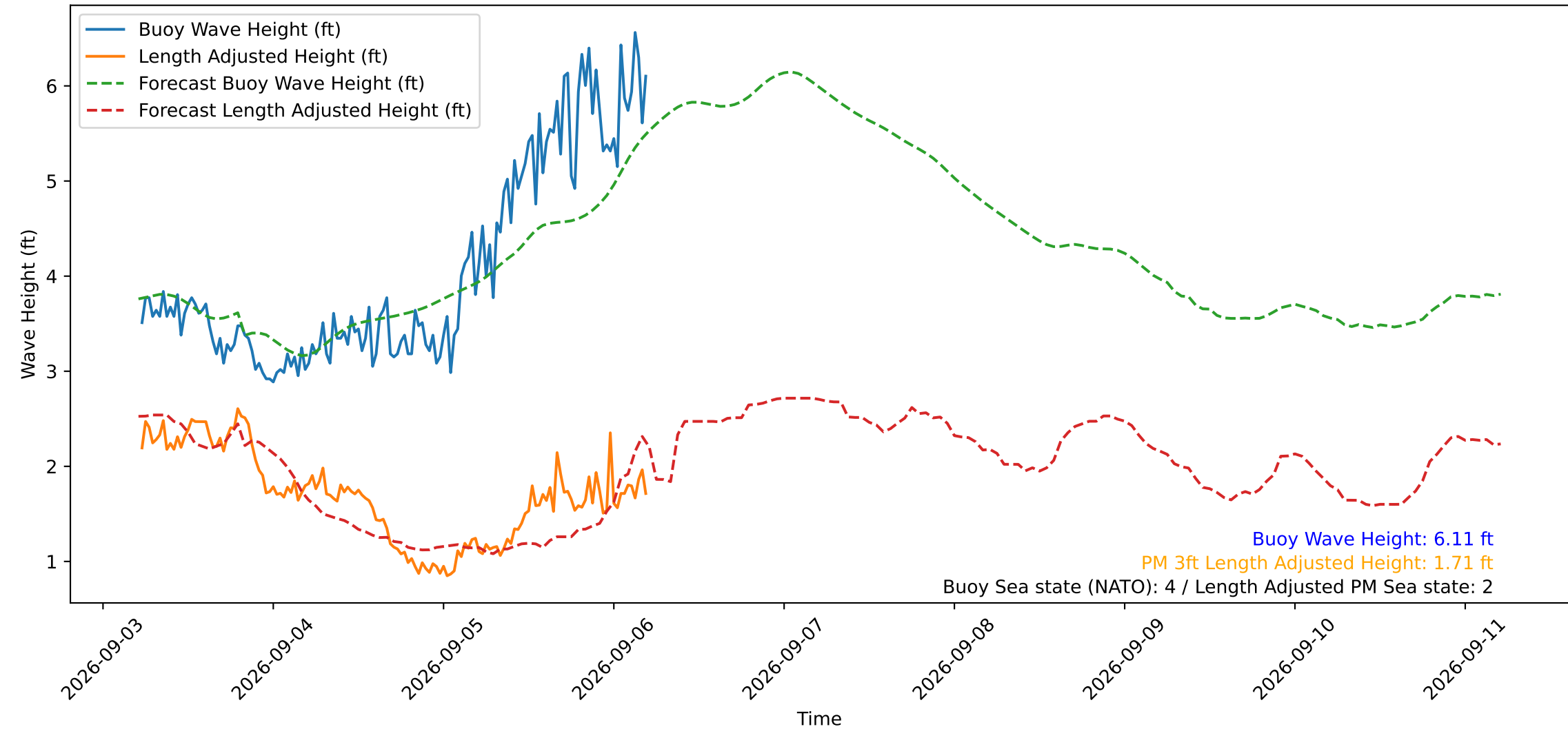
Wave Heights over Time for Oceanside Harbor at 2026-09-06 05:20:30
