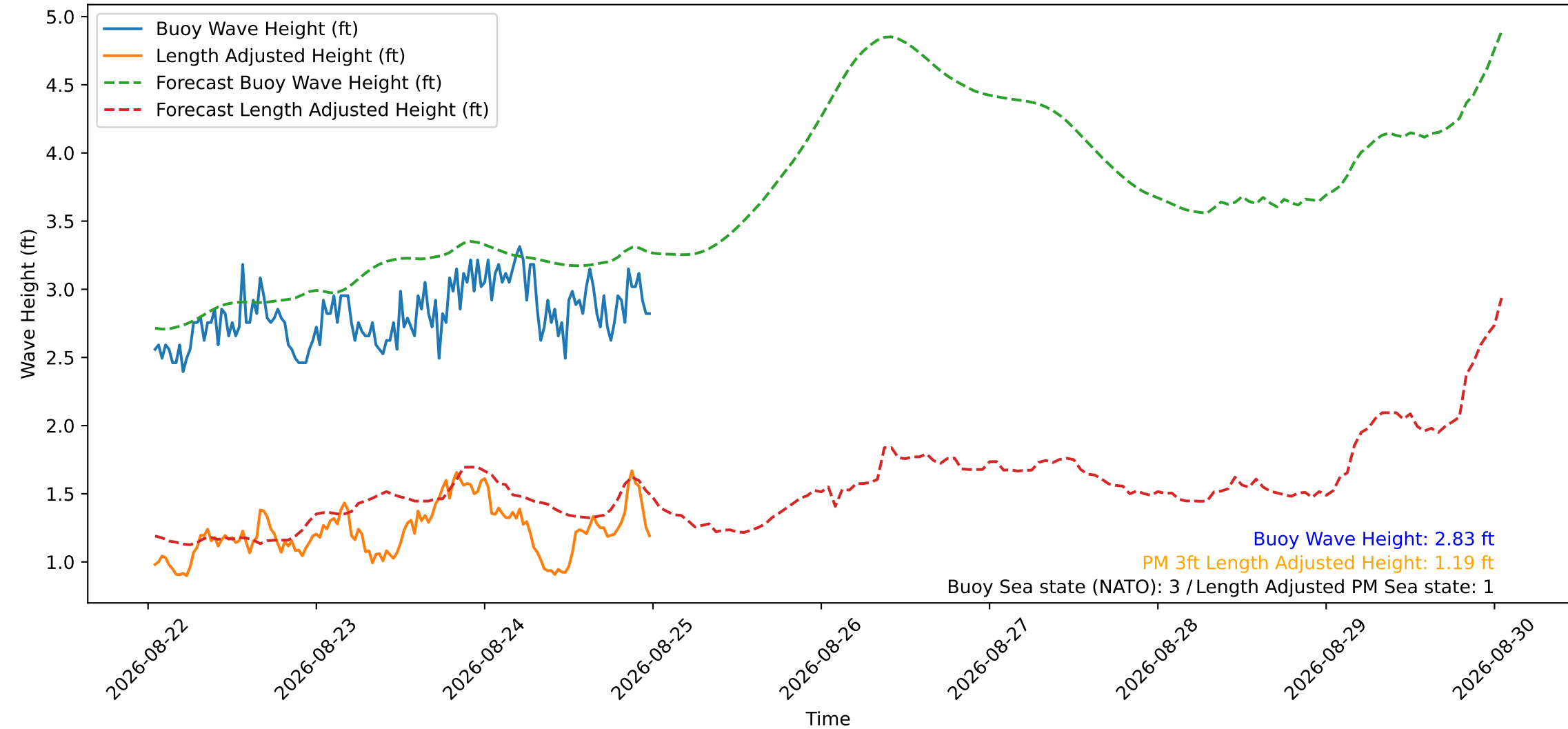
Wave Heights over Time for Green Beach at 2026-08-25 00:51:14
