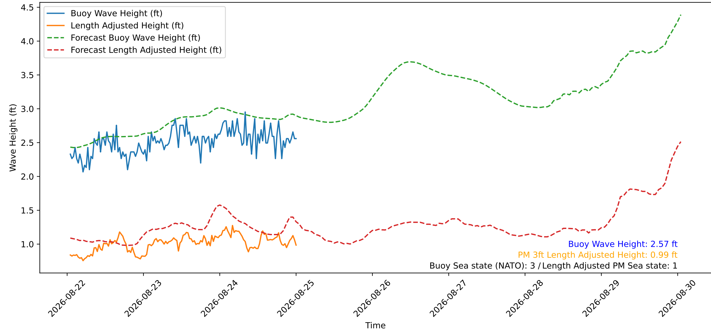
Wave Heights over Time for Red Beach at 2026-08-25 00:50:50
