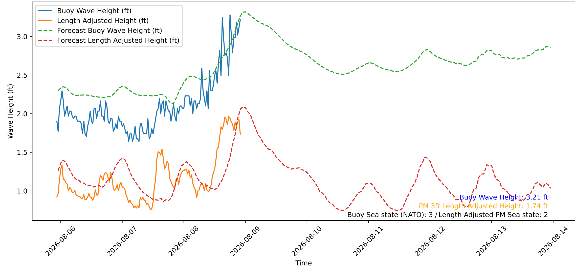
Wave Heights over Time for Oceanside Harbor at 2026-08-08 22:40:27
