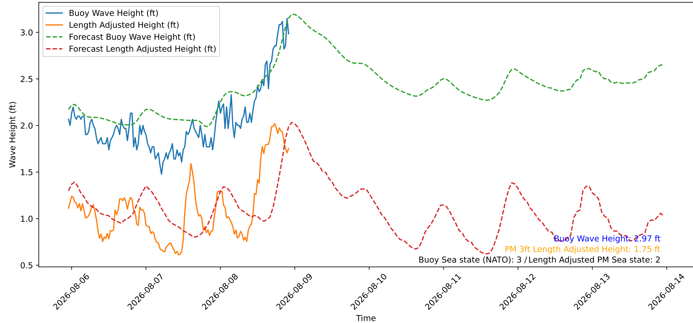
Wave Heights over Time for Red Beach at 2026-08-08 22:40:46
