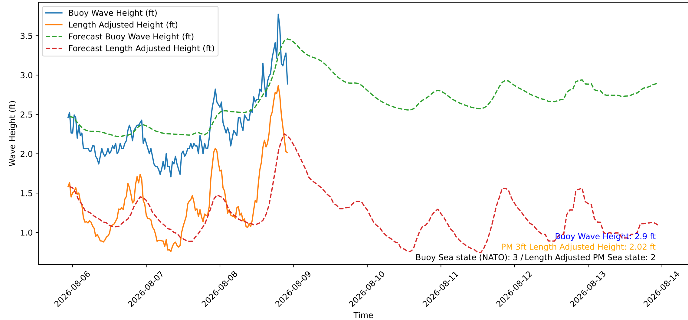
Wave Heights over Time for Green Beach at 2026-08-08 22:41:09
