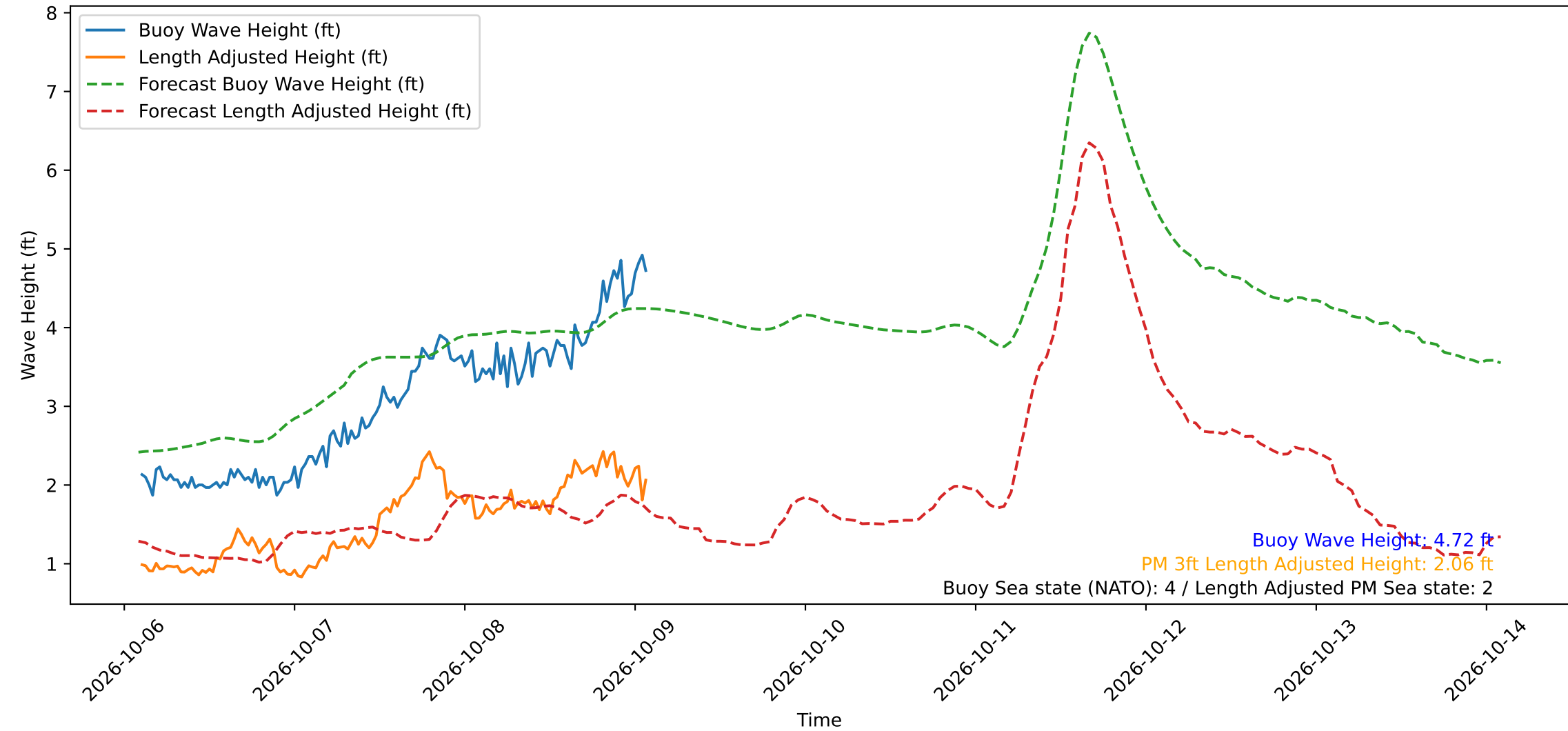
Wave Heights over Time for Red Beach at 2026-10-09 02:10:49
