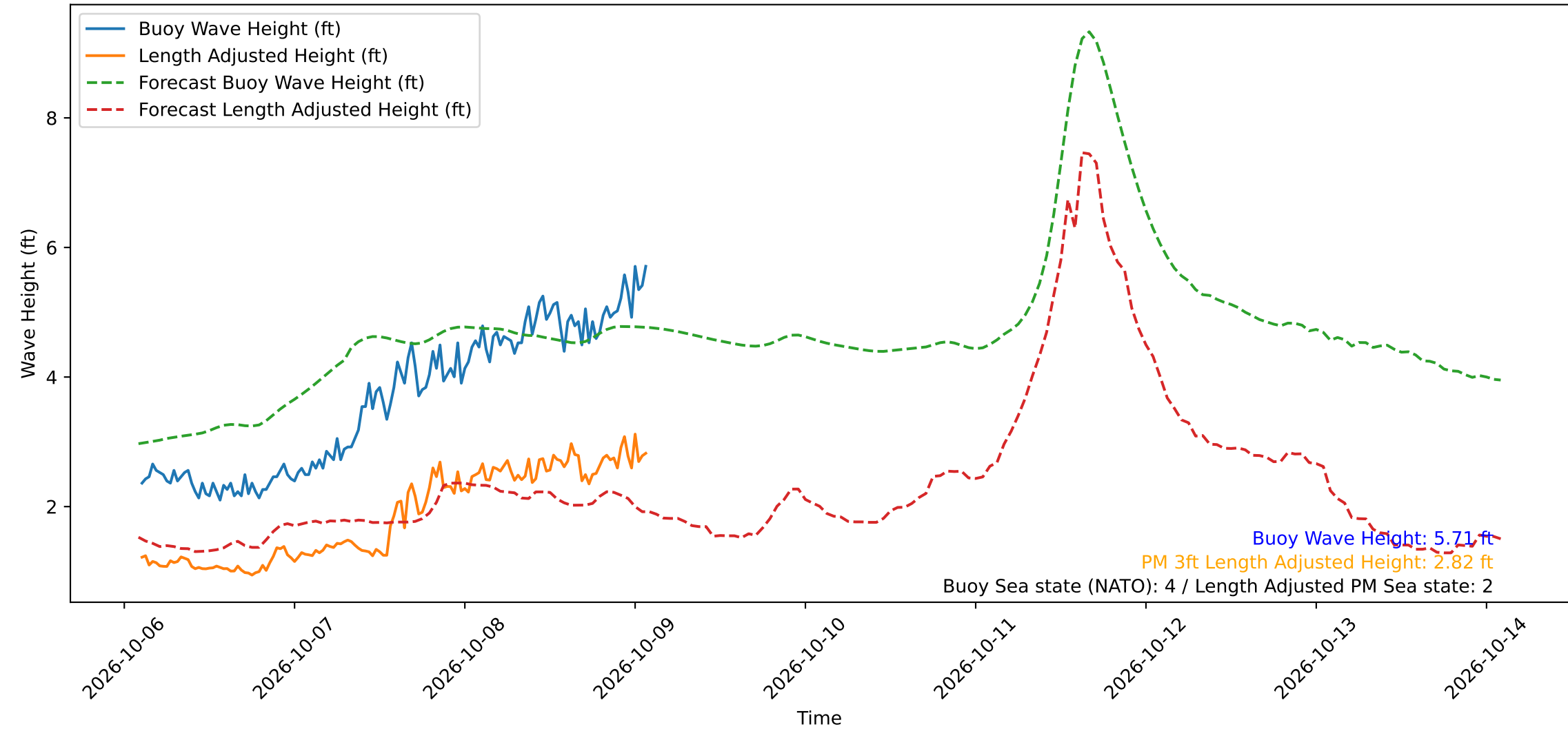
Wave Heights over Time for Green Beach at 2026-10-09 02:11:12
