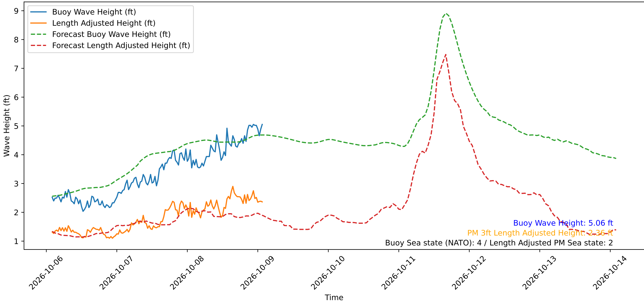
Wave Heights over Time for Oceanside Harbor at 2026-10-09 02:10:30
