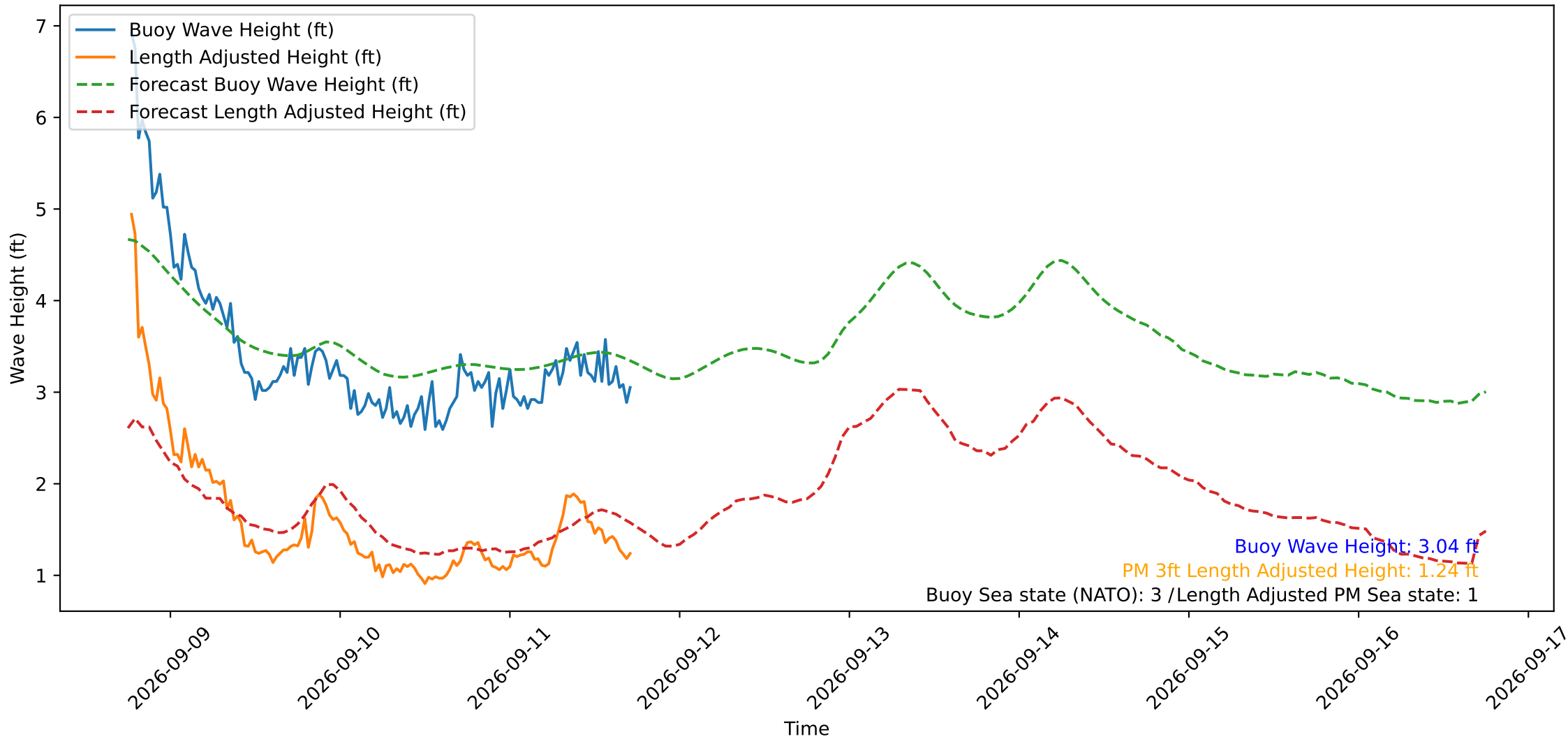
Wave Heights over Time for Green Beach at 2026-09-11 18:01:13
