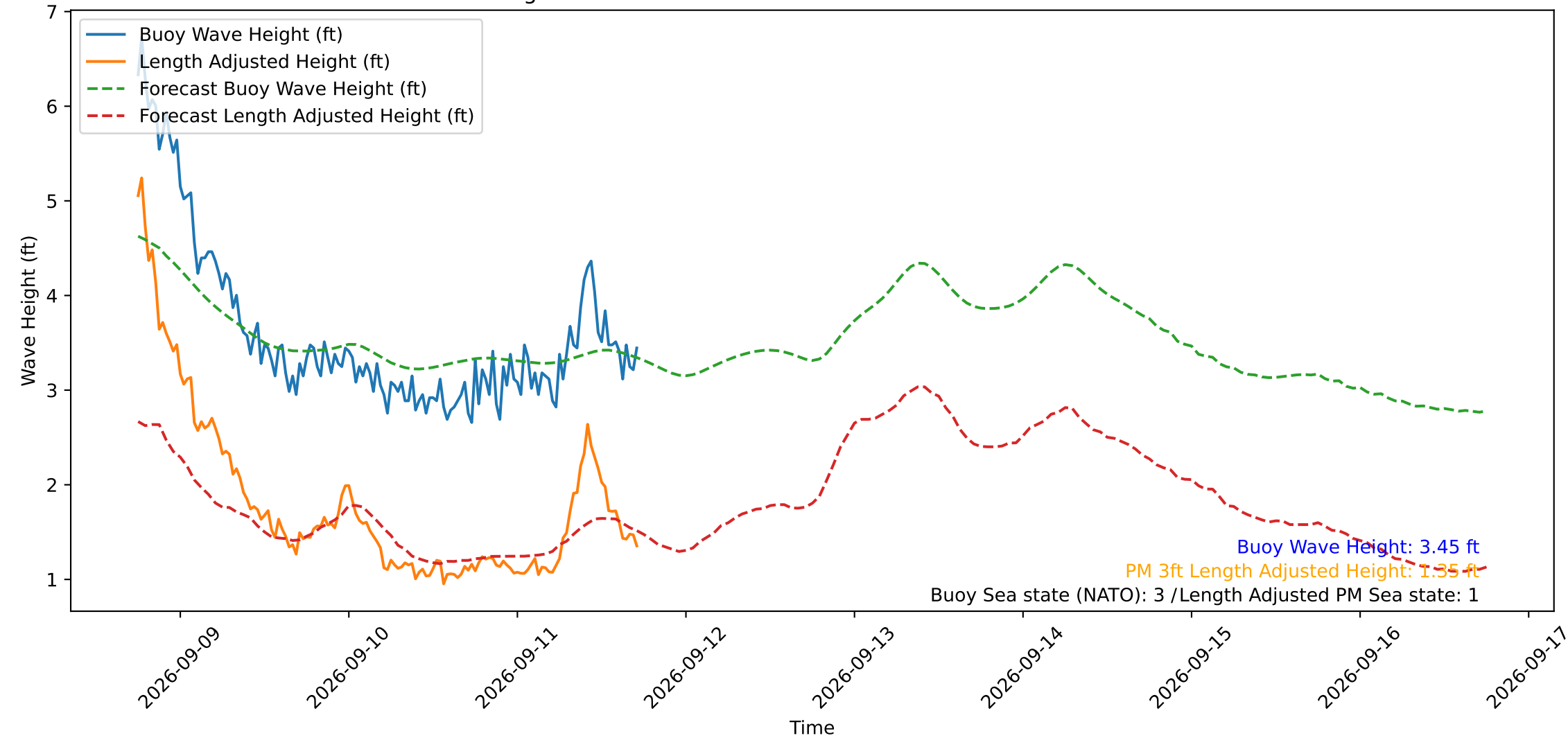
Wave Heights over Time for Oceanside Harbor at 2026-09-11 18:00:30
