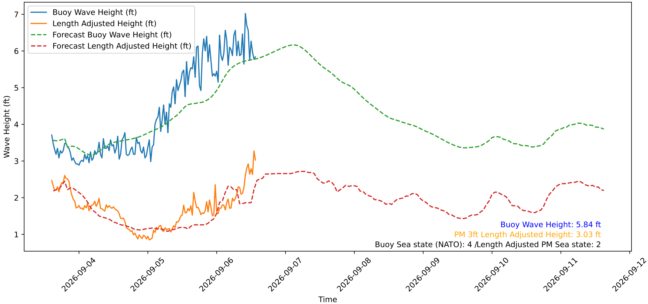
Wave Heights over Time for Oceanside Harbor at 2026-09-06 14:30:29
