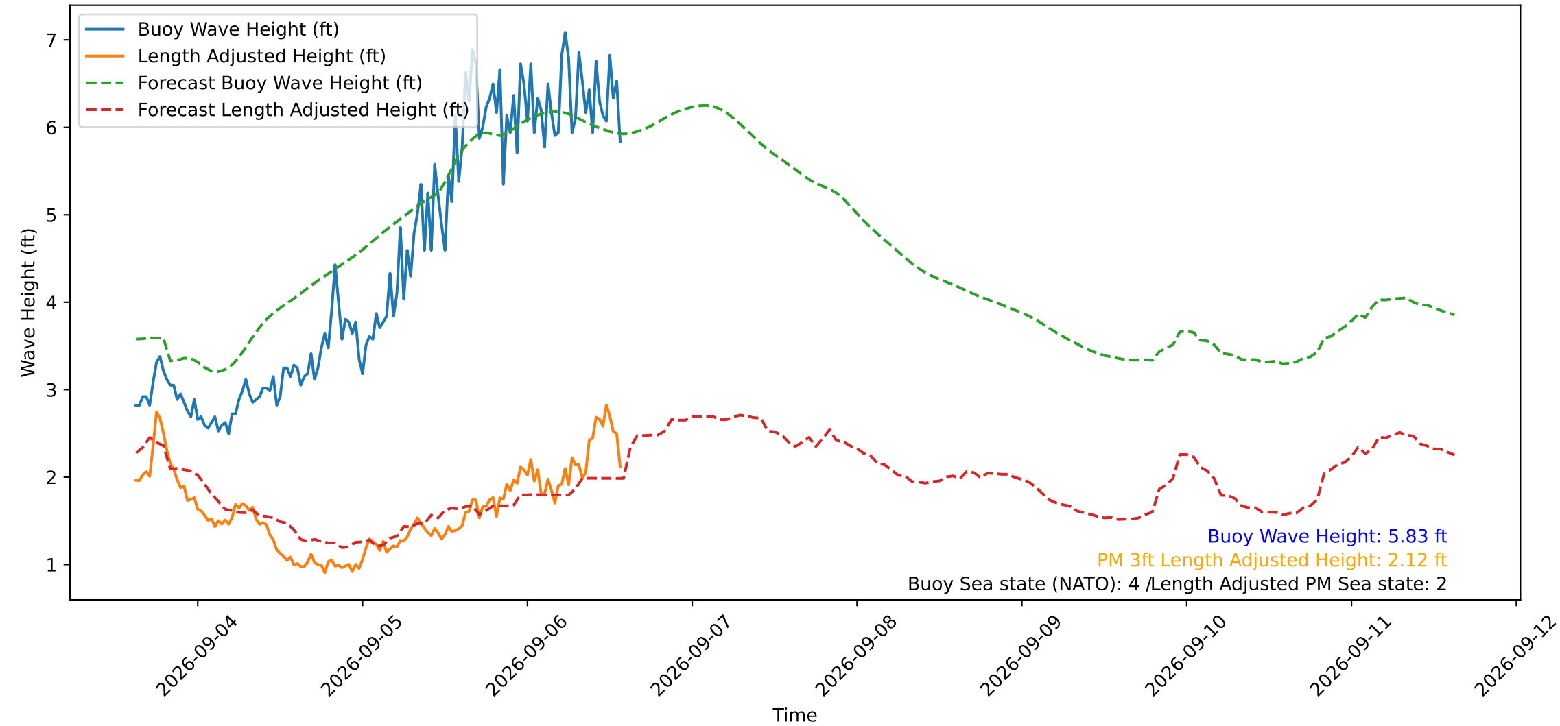
Wave Heights over Time for Green Beach at 2026-09-06 14:31:11
