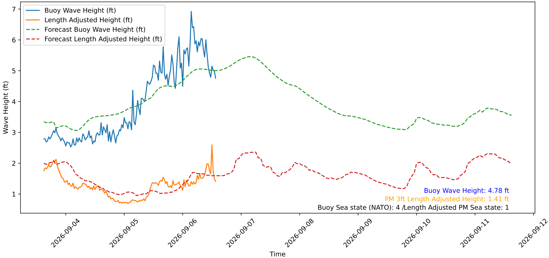
Wave Heights over Time for Red Beach at 2026-09-06 14:30:49
