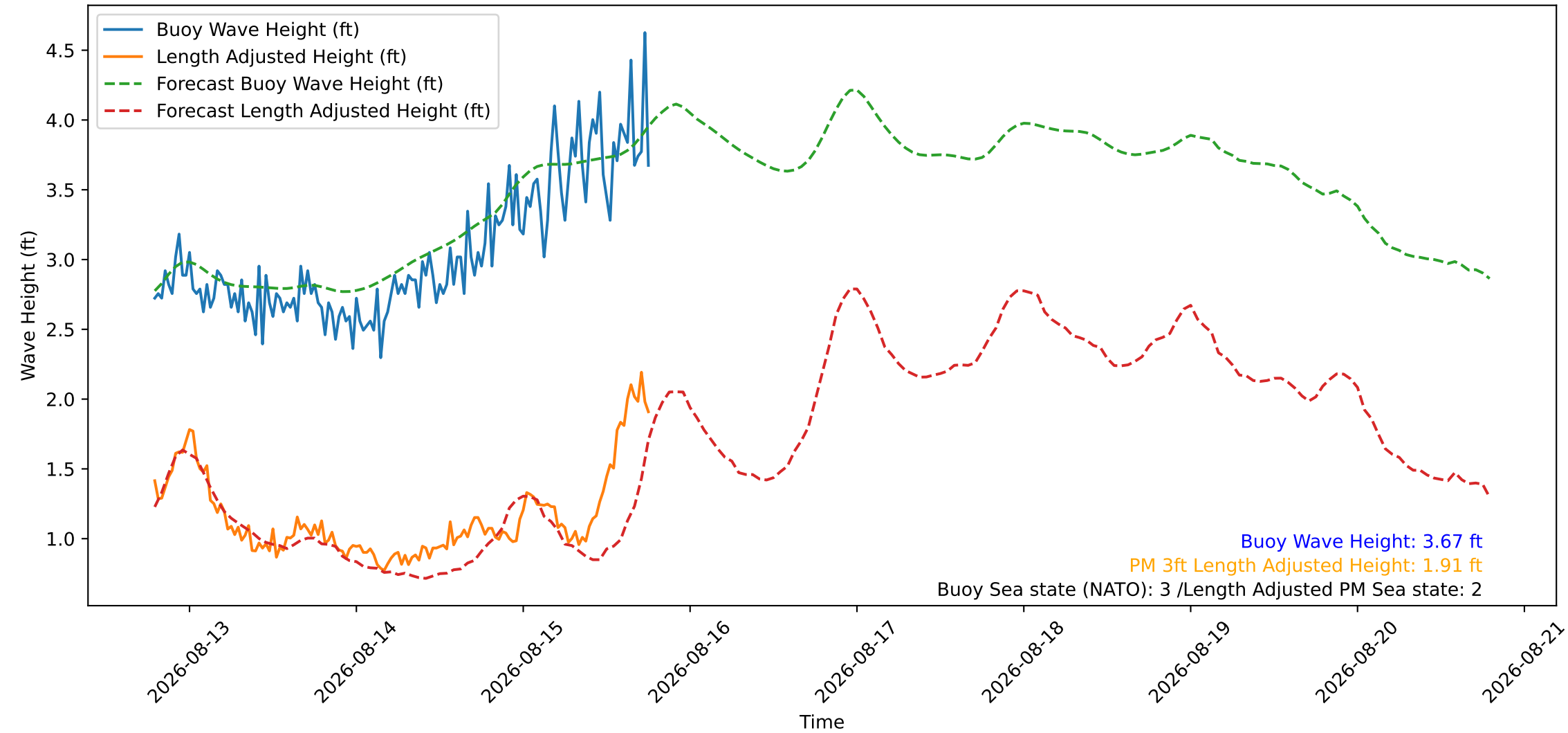
Wave Heights over Time for Oceanside Harbor at 2026-08-15 18:50:27
