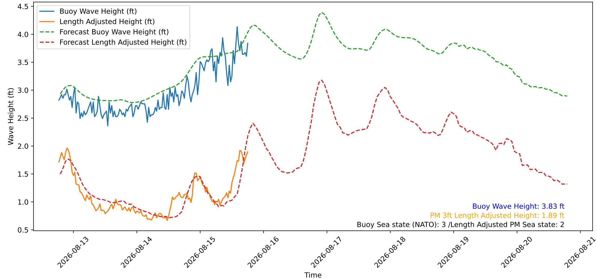
Wave Heights over Time for Green Beach at 2026-08-15 18:51:12
